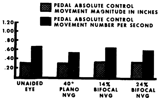
FIGURE 11. Pedal Control Input Data--Hover Forward Maneuver NVG Bifocal Evaluation
