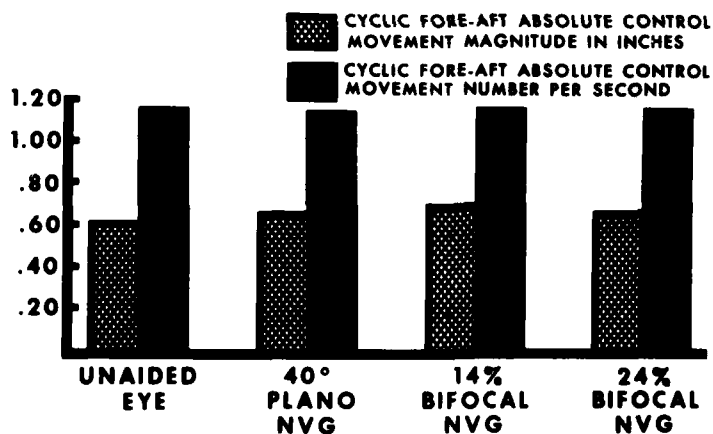
FIGURE 9. Cyclic Fore-Aft Control Input Data-- Hover Forward Maneuver NVG Bifocal Evaluation
