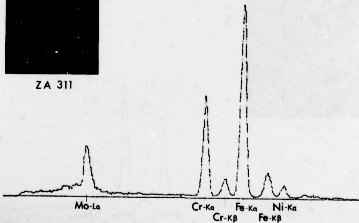
FIG 7 TYPICAL ELECTRON MICROGRAPH, DIFFRACTION PATTERN AND X-RAY ANALYSIS SPECTRUM OF CHI-PHASE IN 316 ss
