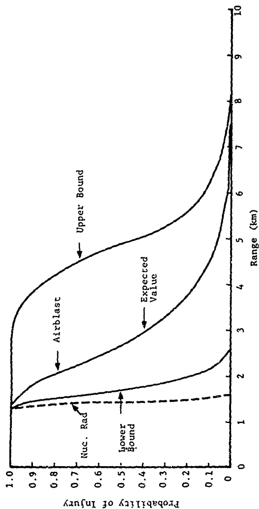
Figure 7.116. Injury Damage Function, People in Basements, 100 KT, 200 ft/KT 1/3 Scaled Height of Burst.
