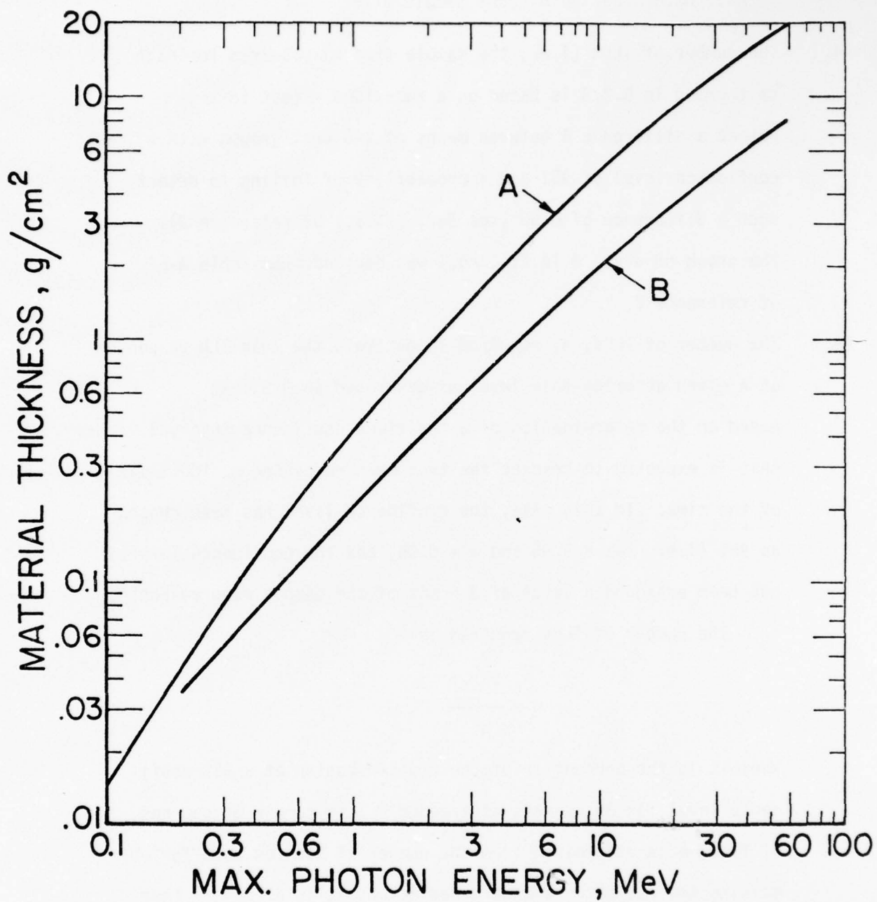
Fig. A3.1 Material thickness required for electron equilibrium. A: electron range. B: depth of peak dose.
