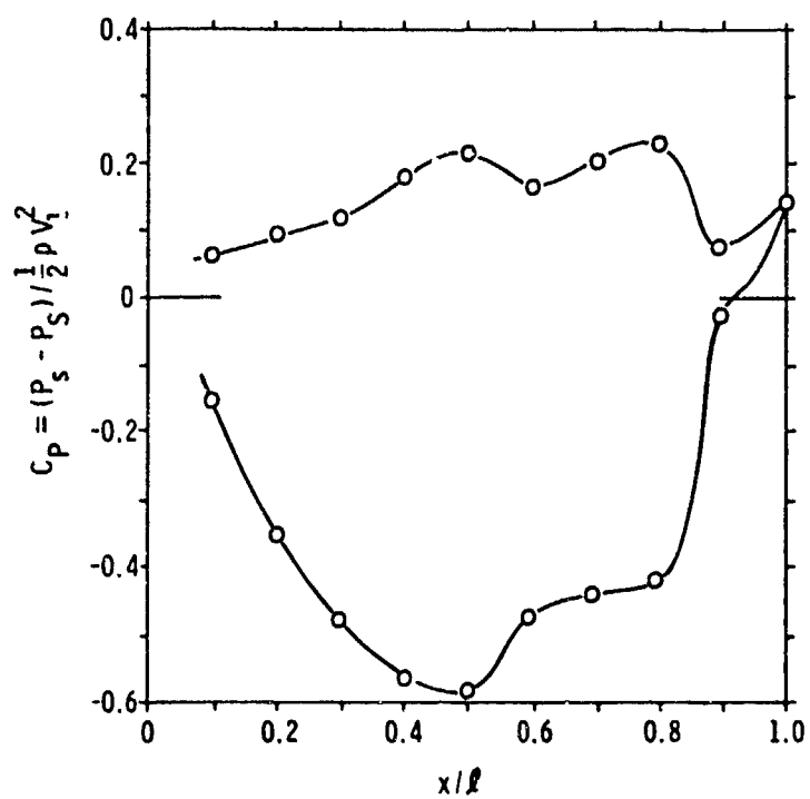
Figure 53. Experimental Cascade Blade Pressure Distribution.
