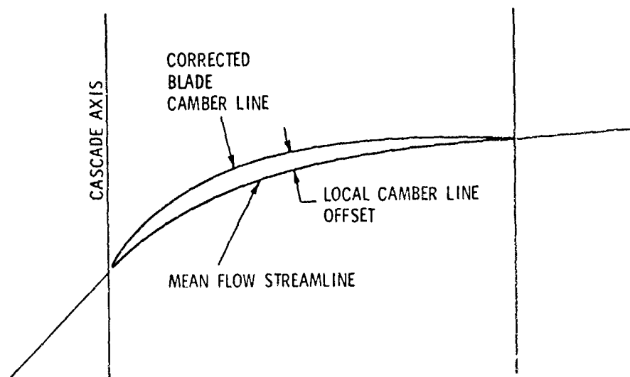
Figure 31. Schematic Representation of Camber Line Corrected to Account for Potential and Real Flow Effects in a Cascade.
