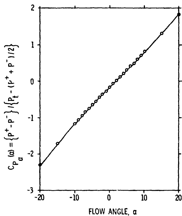
Figure 48. Three-Hole Probe Calibration ( C_{p_a} vs \alpha ).
