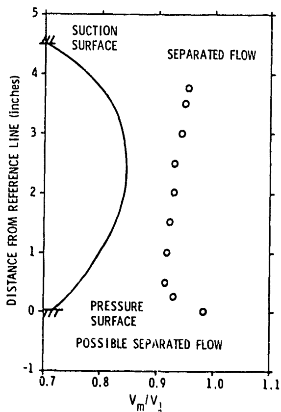
Figure 66. Comparison of the Theoretical and Experimental Velocity Profiles in the Test Cascade Reference Station Coincident with Trailing Edge.
