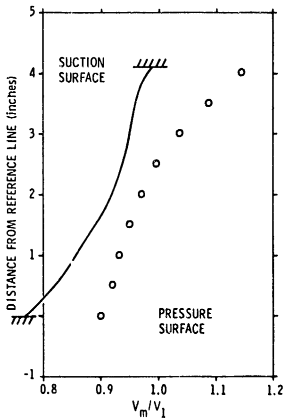
Figure 63. Comparison of the Theoretical and Experimental Velocity Profiles in the Test Cascade Reference Station at 70 Percent of the Blade Chord.
