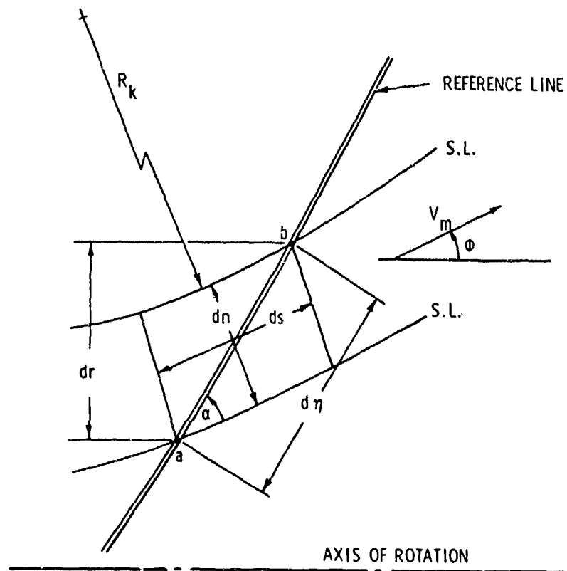
Figure 5. Differential Streamtube Element.
