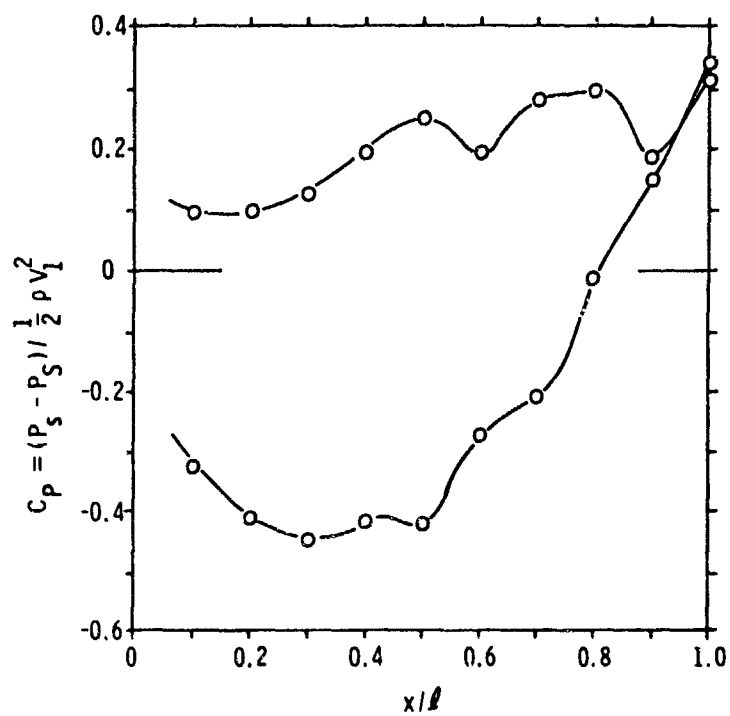
Figure 51. Theoretical Cascade Blade Pressure Distribution from the Streamline Curvature Analysis.
