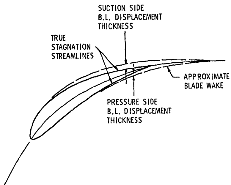
Figure 39. Modification of the Stagnation Streamline to Account for Boundary Layer Displacement Thickness and the Blade Wake.
