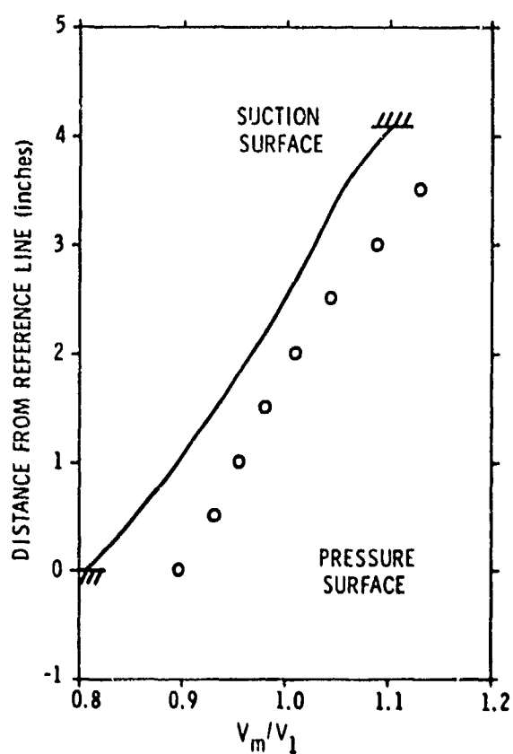
Figure 61. Comparison of the Theoretical and Experimental Velocity Profiles in the Test Cascade Reference Station at 50 Percent of the Blade Chord.
