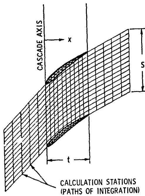
Figure 34. Generalized Cascade Flow Field Geometry.
