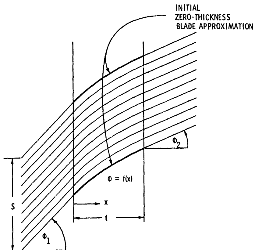
Figure 33. Initial Solution Geometry Consisting of a Number of Parallel Mean Streamlines Between Ideal, Zero Thickness Blades.
