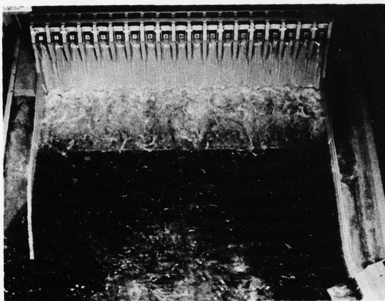
Spillway discharge 260,000 cfs, tailwater elev 788.2.
