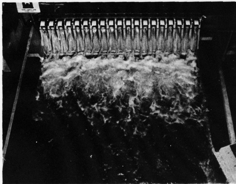
River and spillway discharge 1,200,000 cfs, tailwater elev 825.0.
