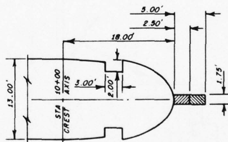
ELLIPTICAL PIER NOSE
