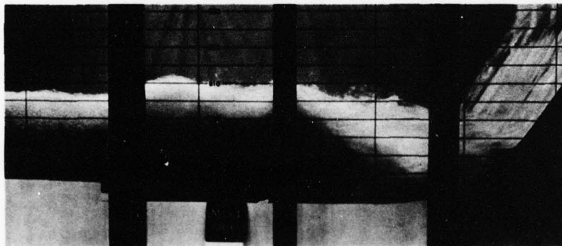
River discharge 440,000 cfs (23,370 cfs per bay), 100-year flood, pool elev 956.0, tailwater elev 798.5, no powerhouse operation.
