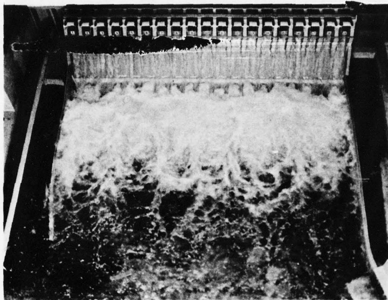
River and spillway discharge 750,000 cfs, tailwater elev 809.8.
