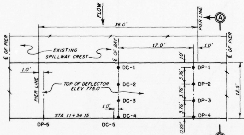
DEFLECTOR WITH PIEZOMETER LOCATIONS
