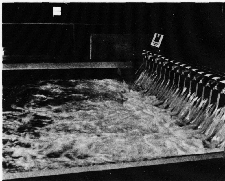
Stilling basin and north training wall.
