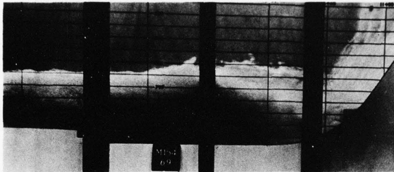
River discharge 440,000 cfs (16,390 cfs per bay), 100-year flood, pool elev 956.0, tailwater elev 798.5, 18 powerhouse units operating.
