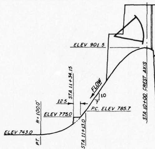
SECTION THROUGH SPILLWAY
