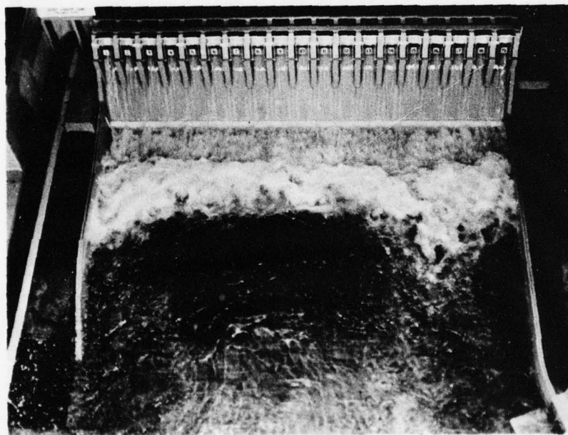
Nonuniform spillway operation (no surging).
