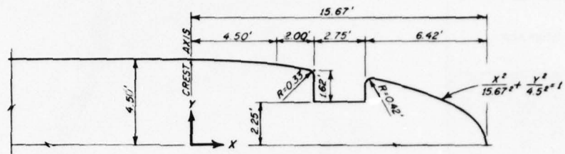
HALF PLAN PIER DETAIL
