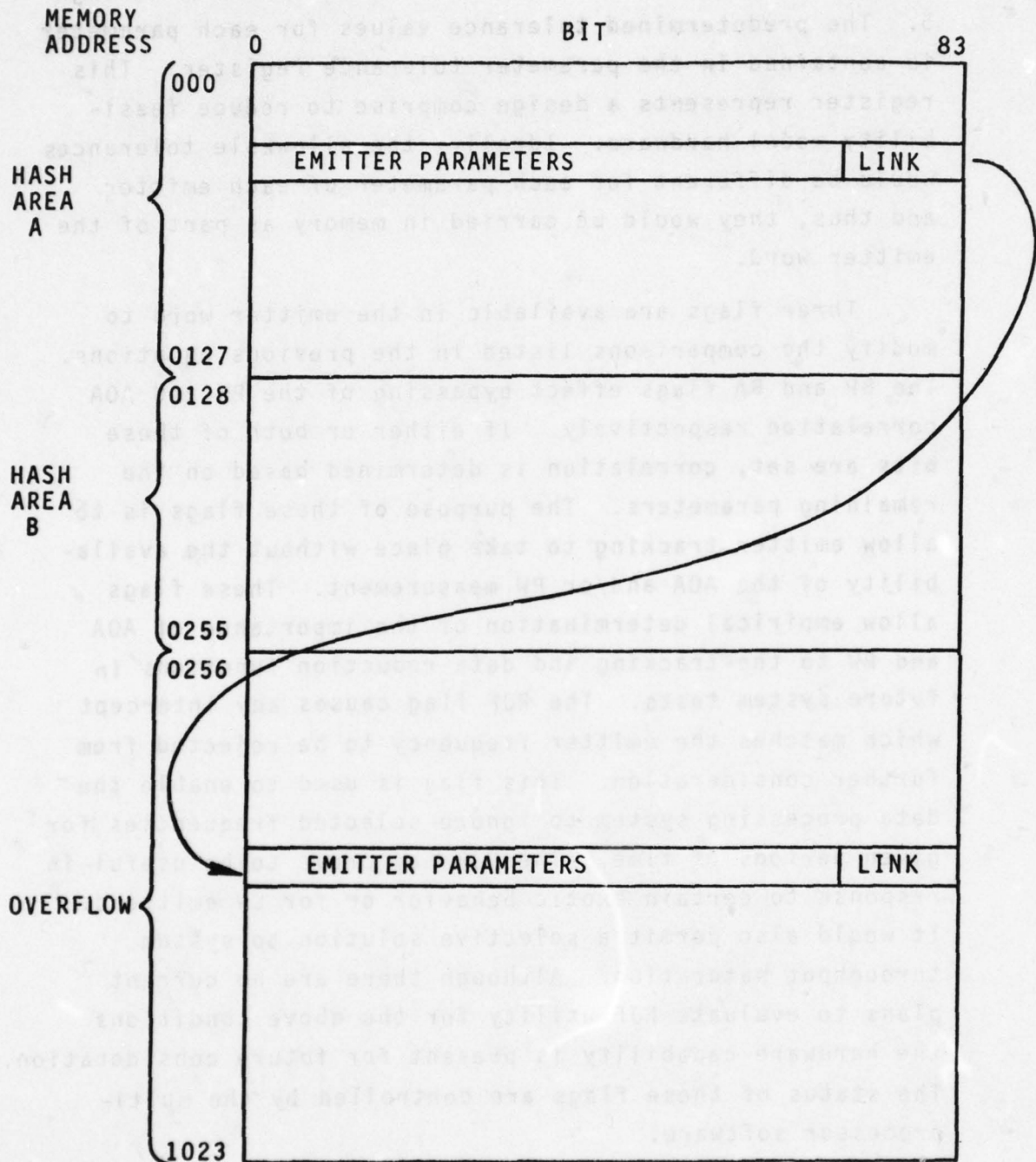
Figure 4 - Emitter File Memory Structure
