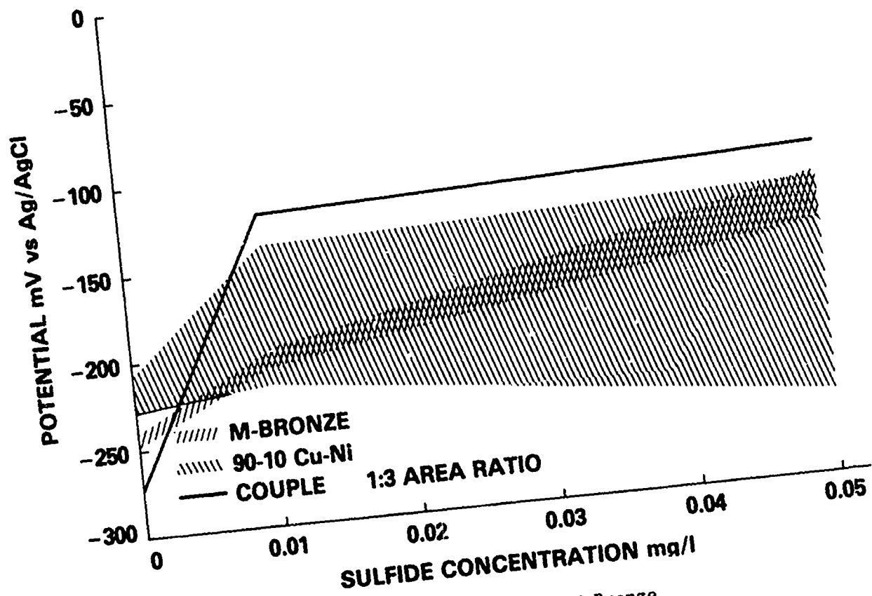
Figure 7 - Potentials of M-Bronze and 90-10 Cu-Ni
