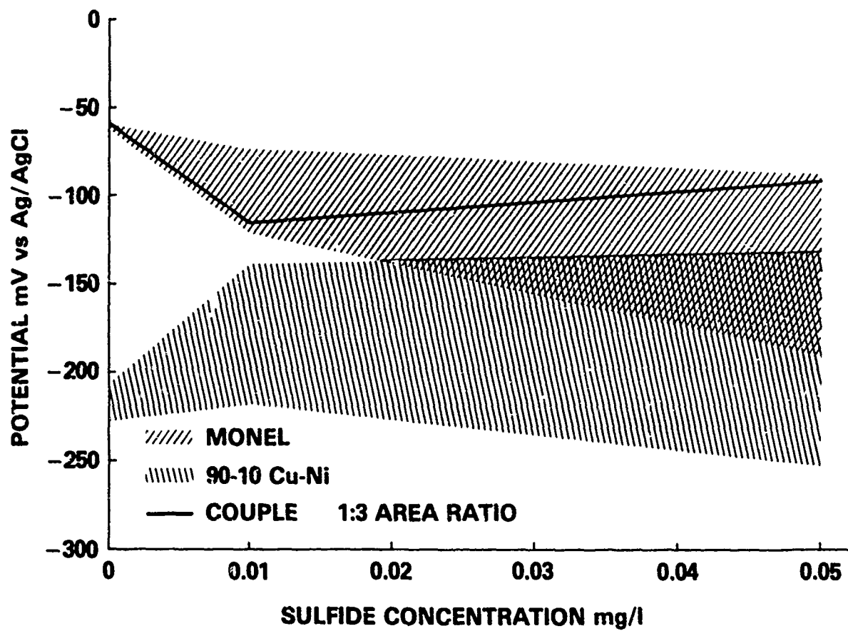
Figure 9 - Potentials of Monel and 90-10 Cu-Ni
