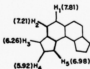
Figure 2 Assignment of ^1\text{H} NMR Chemical Shifts ( \delta ) for XXV.
