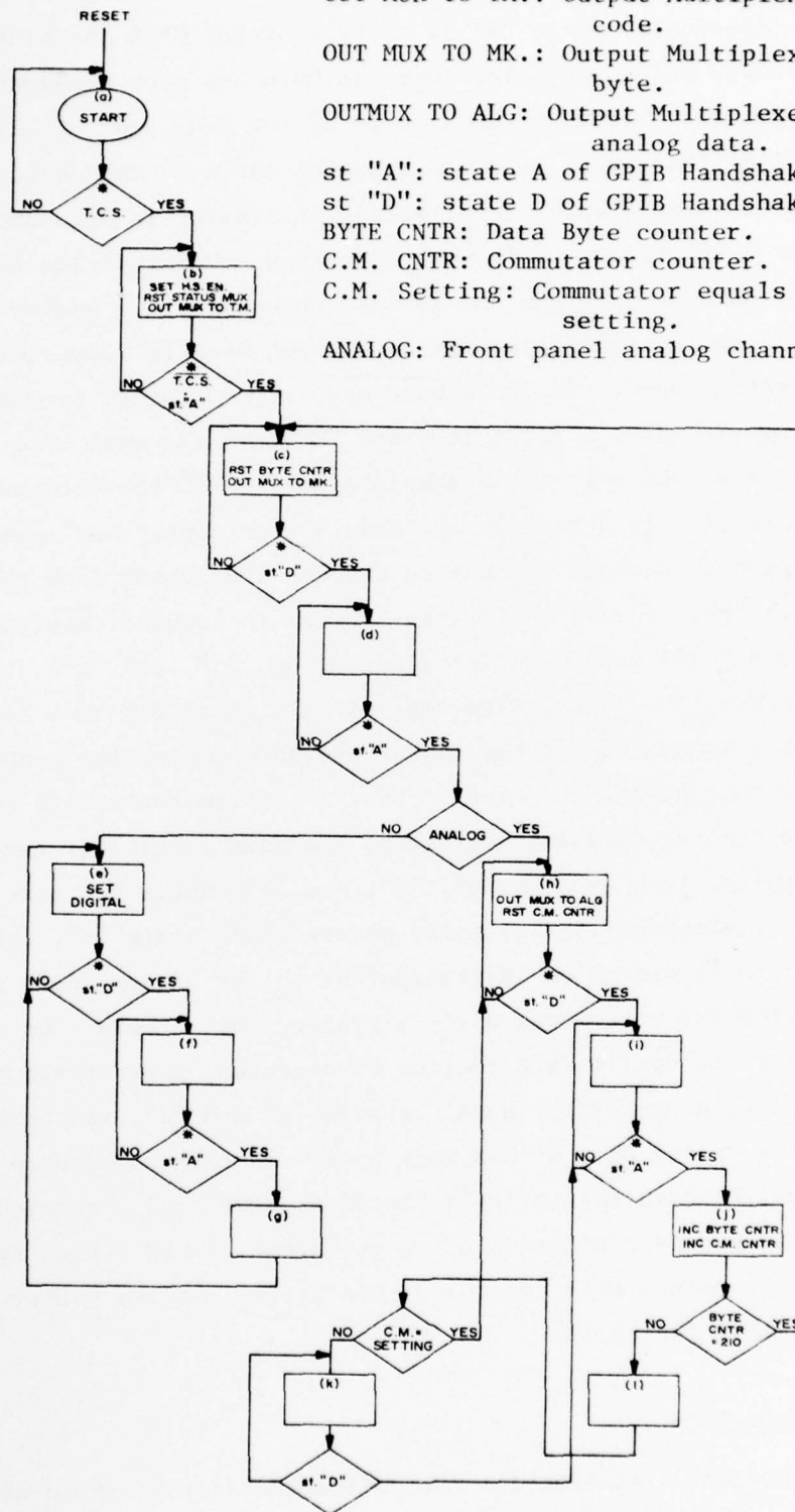
Figure 7. Main System Controller: Flow Chart
