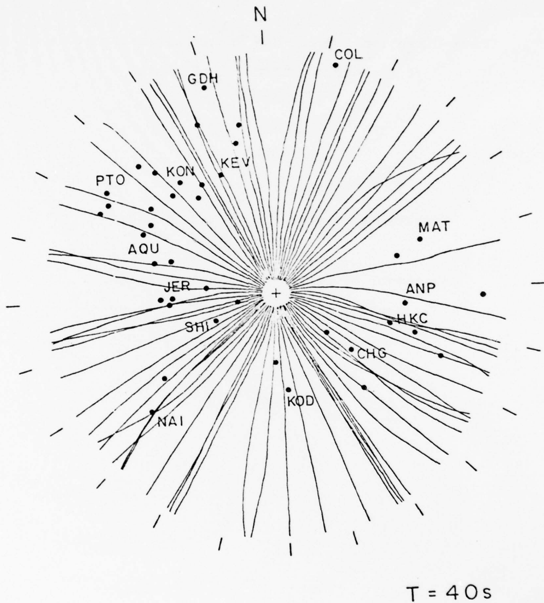
Fig. 5-4.1: Ray paths of 40sec period Rayleigh waves obtained from synthetic ray tracing experiment discussed in the text. Rays leave source (+) at 5° intervals of azimuth. Tick marks are given at 15° intervals.
