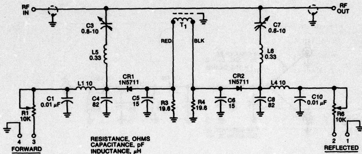
Figure 2-11. Schematic, Power Discriminator.
