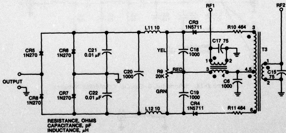
Figure 2-12. Schematic, Phasing Discriminator.
