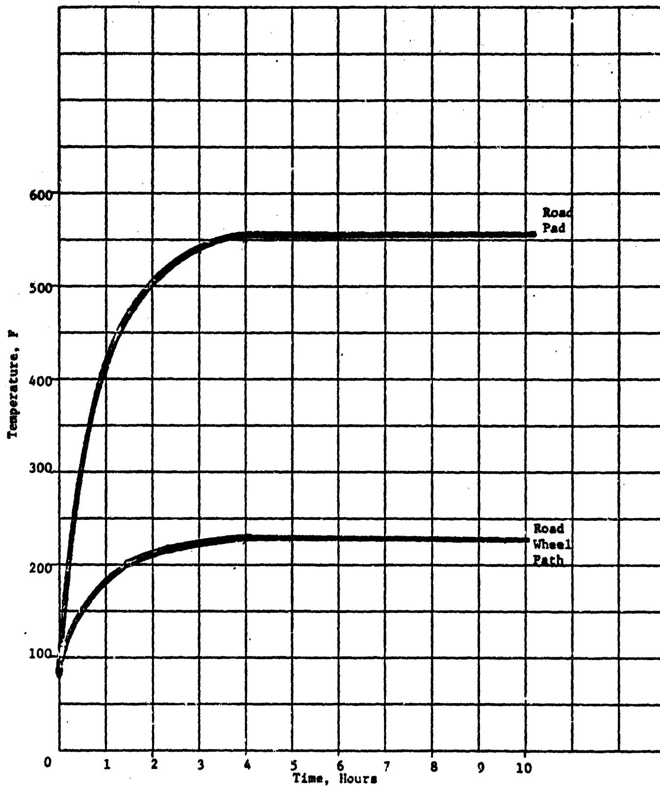
FIGURE 39. ROAD PAD AND ROAD WHEEL PATH TEMPERATURES AT 30 MPH
