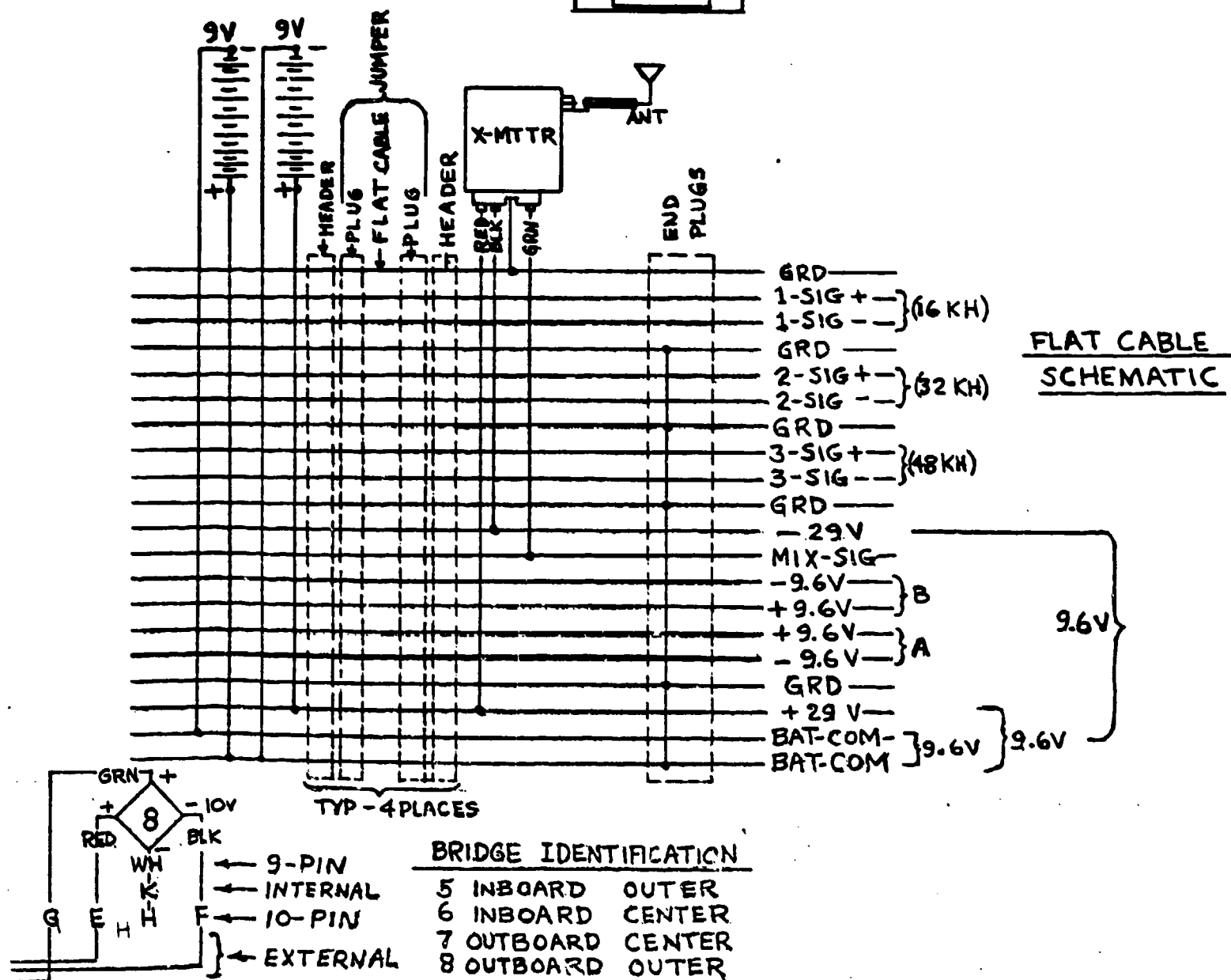
FIGURE G-1. SCHEMATIC DIAGRAM OF TRACK-MOUNTED INSTRUMENTATION CIRCUIT (Continued)
