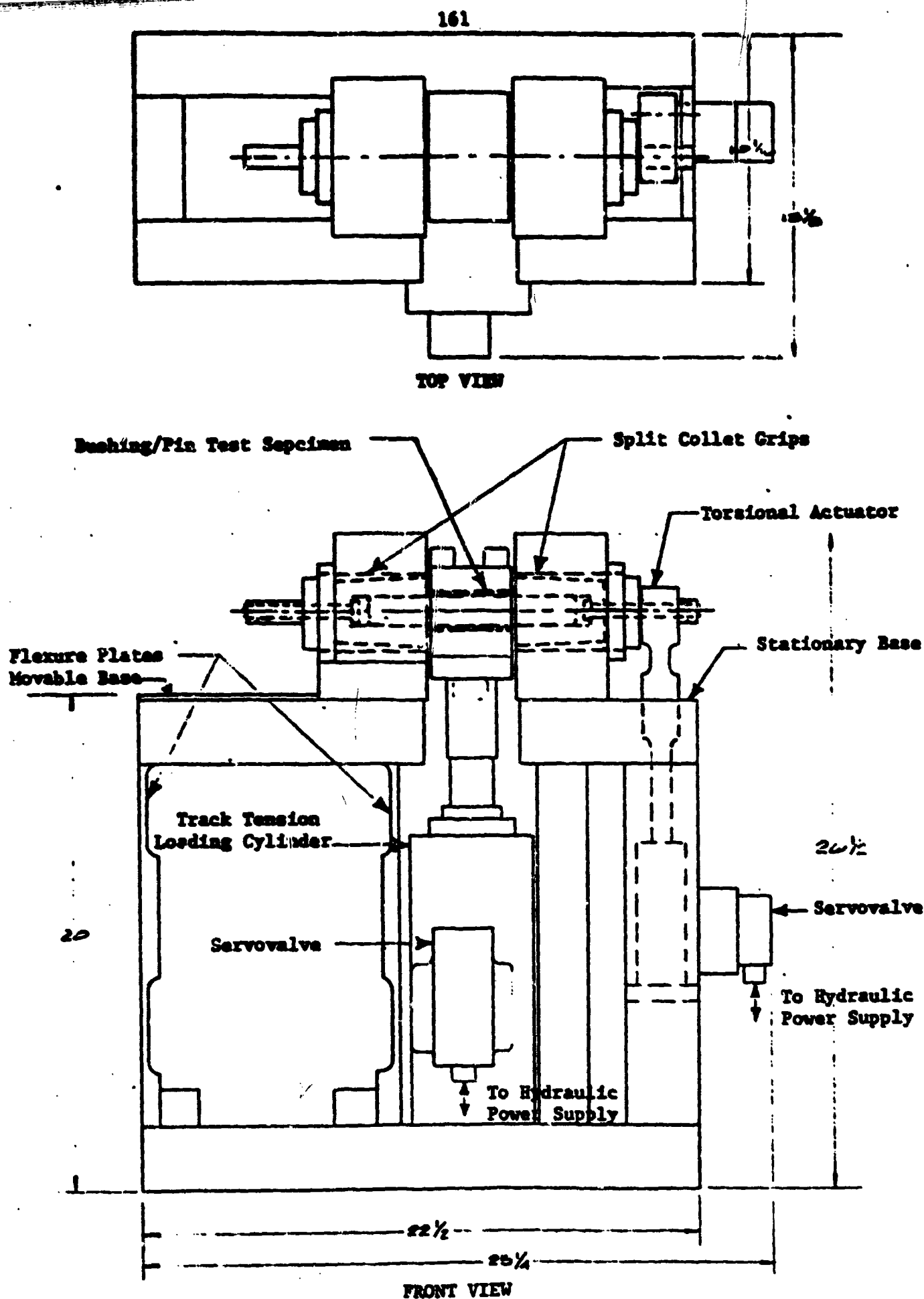
FIGURE 55. BUSHING RESEARCH MACHINE
