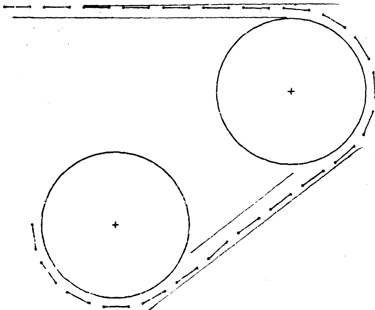
FIGURE 12c. TRACKDYN PLOT SHOWING EFFECT OF BUSHING TORSIONAL STIFFNESS ON TRACK PATH (50 MPH, 5000 LB APPARENT TENSION, TORSIONAL SPRING RATE 1/16 NORMAL) (See page 74 for further discussion.)
