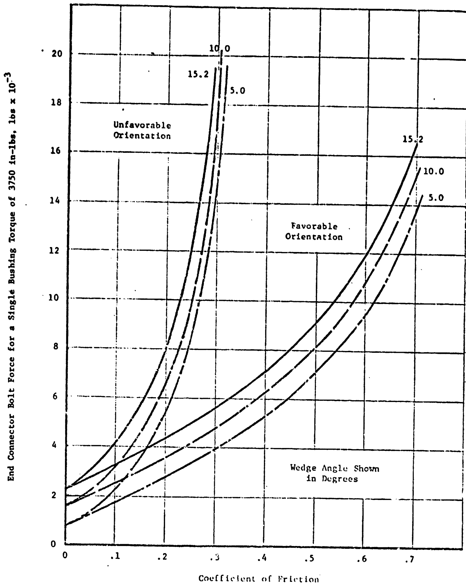
FIGURE 65. WEDGE ANGLE EFFECTS ON CURRENT WEDGE DESIGN
