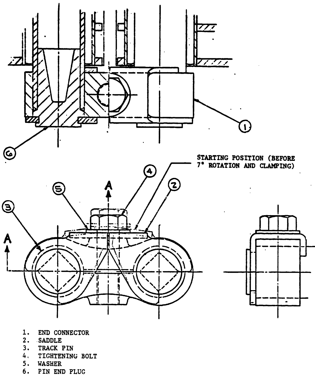
FIGURE 59. CONCEPT FOR IMPROVED END CONNECTOR ASSEMBLY
