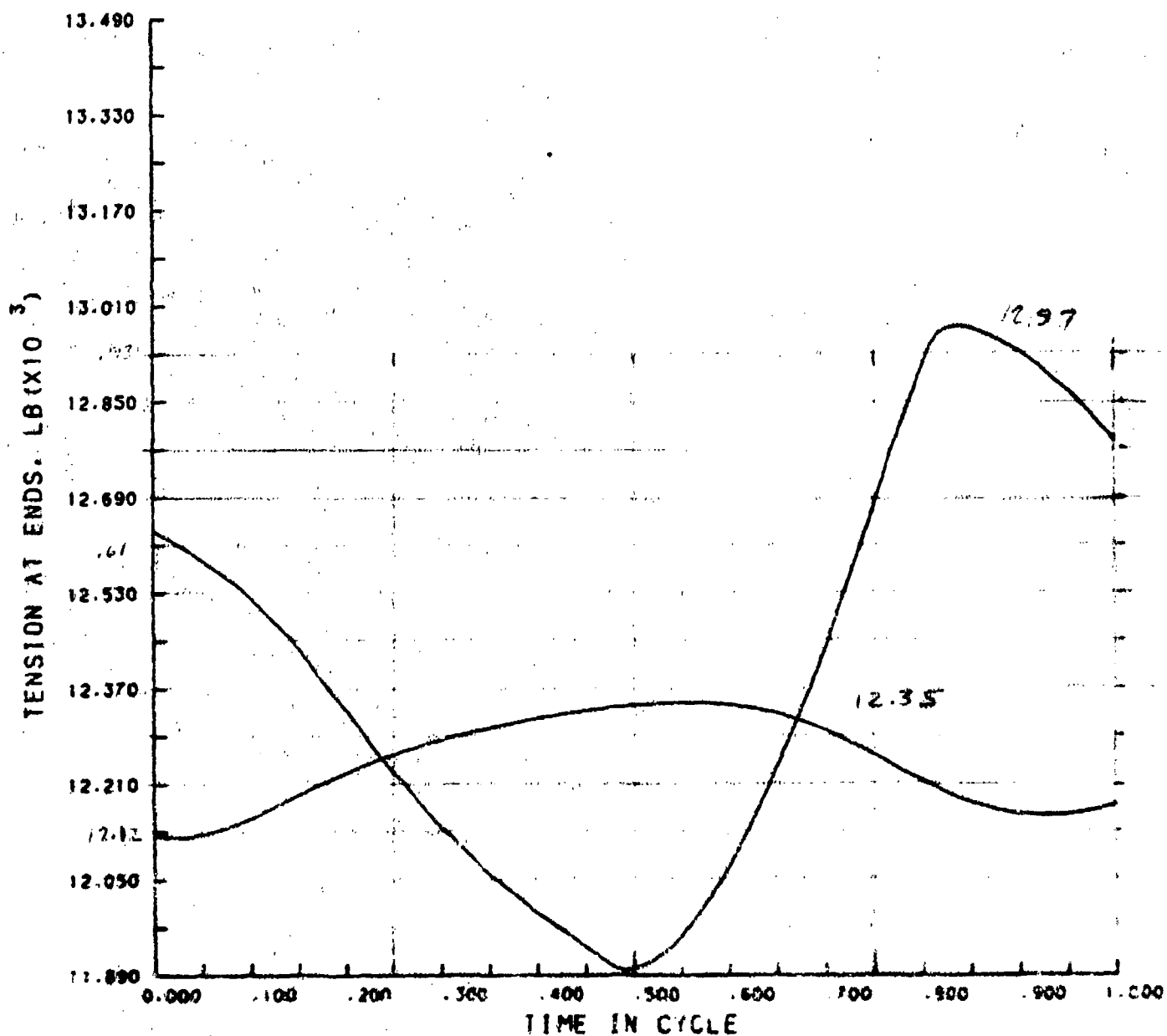
FIGURE 13a. TRACETYPE PLOT OF TENSION HISTORY AT INLET AND NEAR FRONT ROAD WHEEL (35 MPH, 1500 LB APPARENT TENSION)
