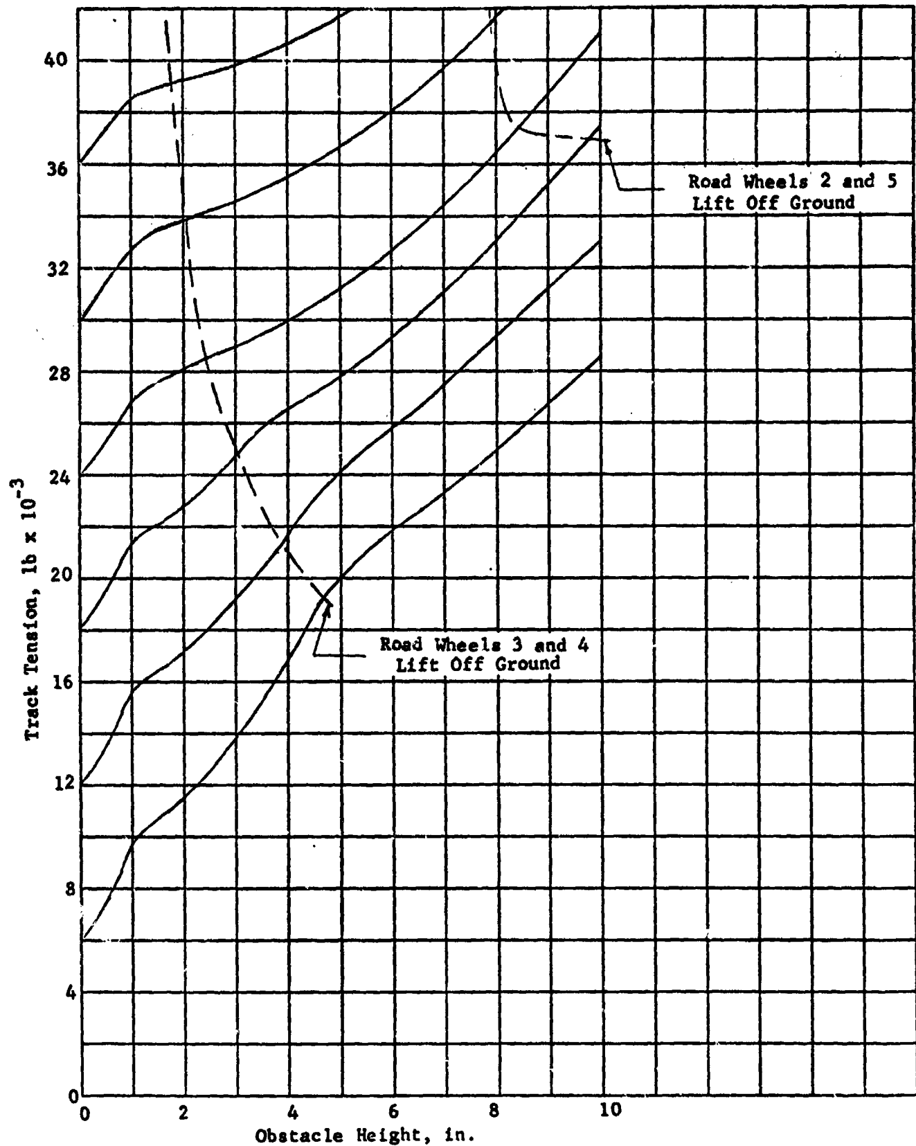
FIGURE 28. EFFECT OF TRACK INITIAL TENSION ON M60 TRACK TENSION WHEN TRAVERSING AN OBSTACLE
