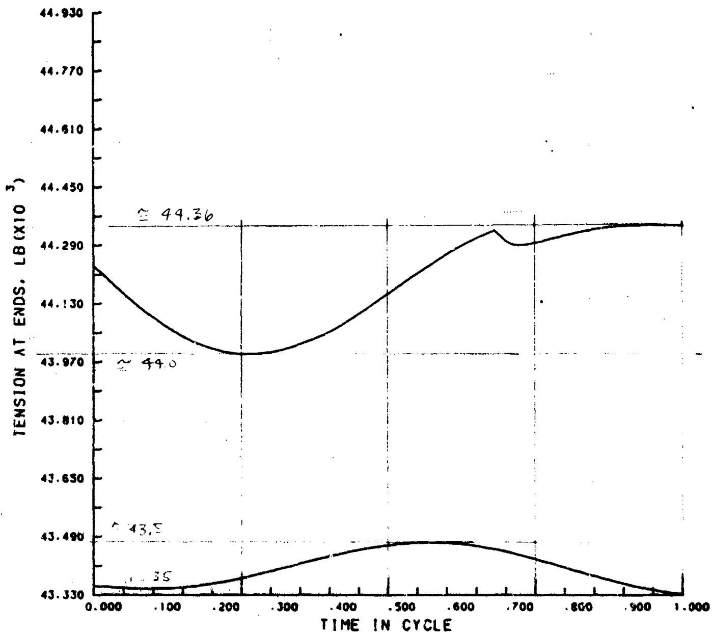
FIGURE 13c. TRACKDYNE PLOT OF TENSION HISTORY AT INLET AND NEAR FRONT ROAD WHEEL (70 MPH, 1500 LB APPARENT TENSION)
