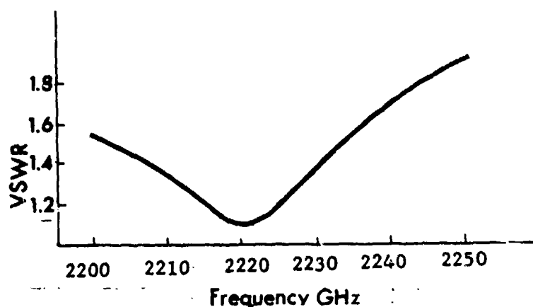
X-BAND VSWR
