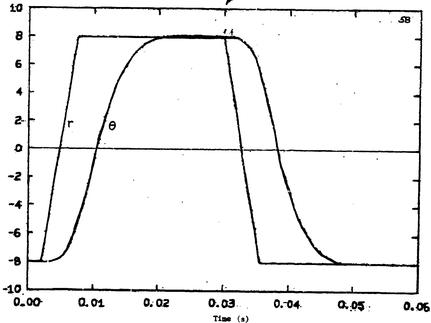
FIGURE E-5. RESPONSE OF BUSHING RESEARCH MACHINE COMPARED TO ACTUAL BUSHING ANGULAR DEFLECTION IN T-142 TRACK (M-60 Tank at 35 mph)
