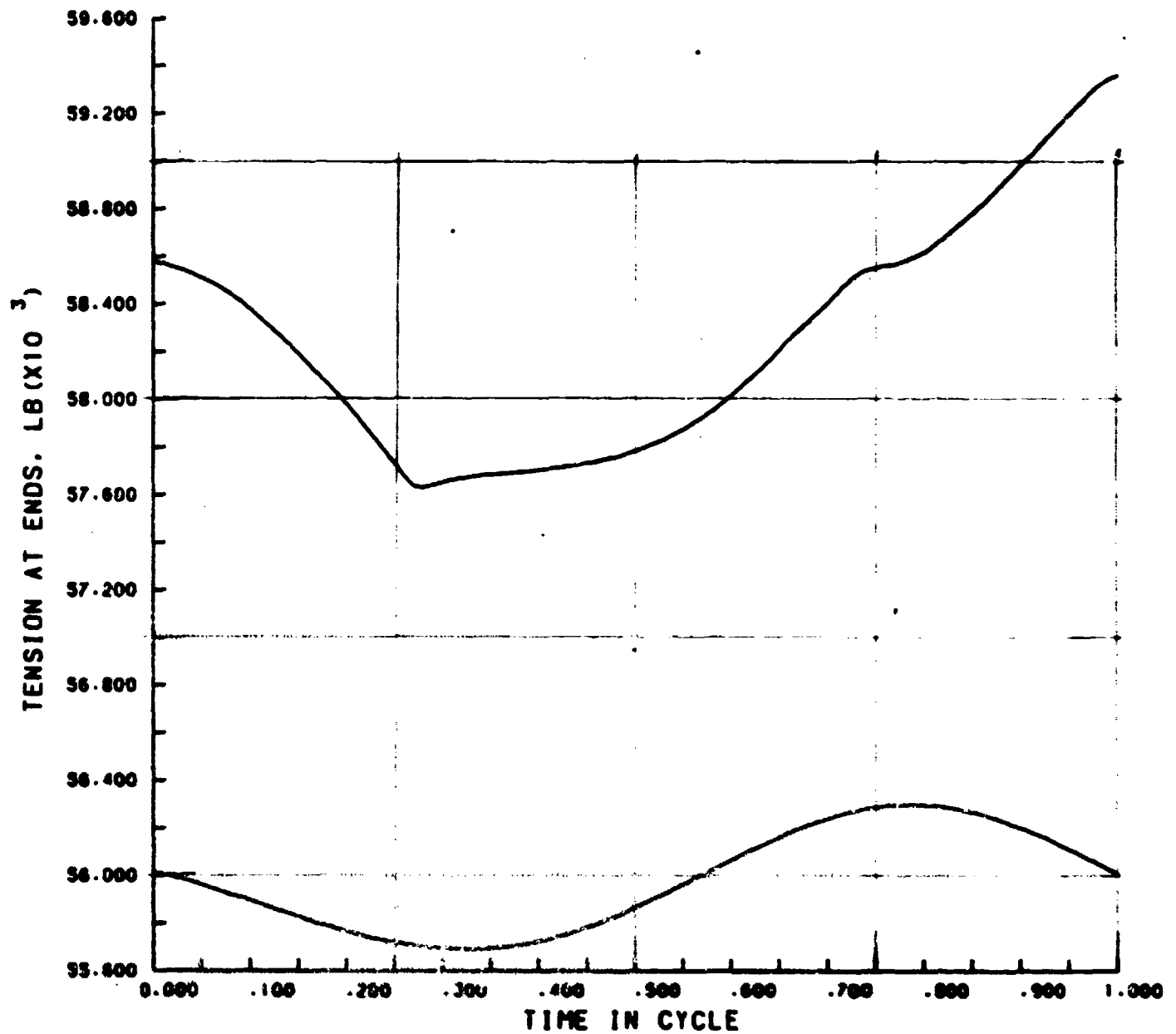
FIGURE 134. TRACKDYNE PLOT OF TENSION HISTORY AT INLET AND NEAR FRONT ROAD WHEEL (70 MPH, 15,000 LB APPARENT TENSION)
