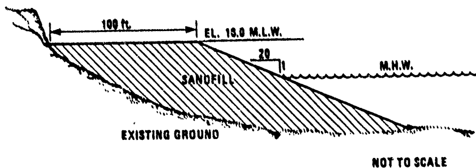
Figure 2-8. Plan VII - Placed Sandfill Only
