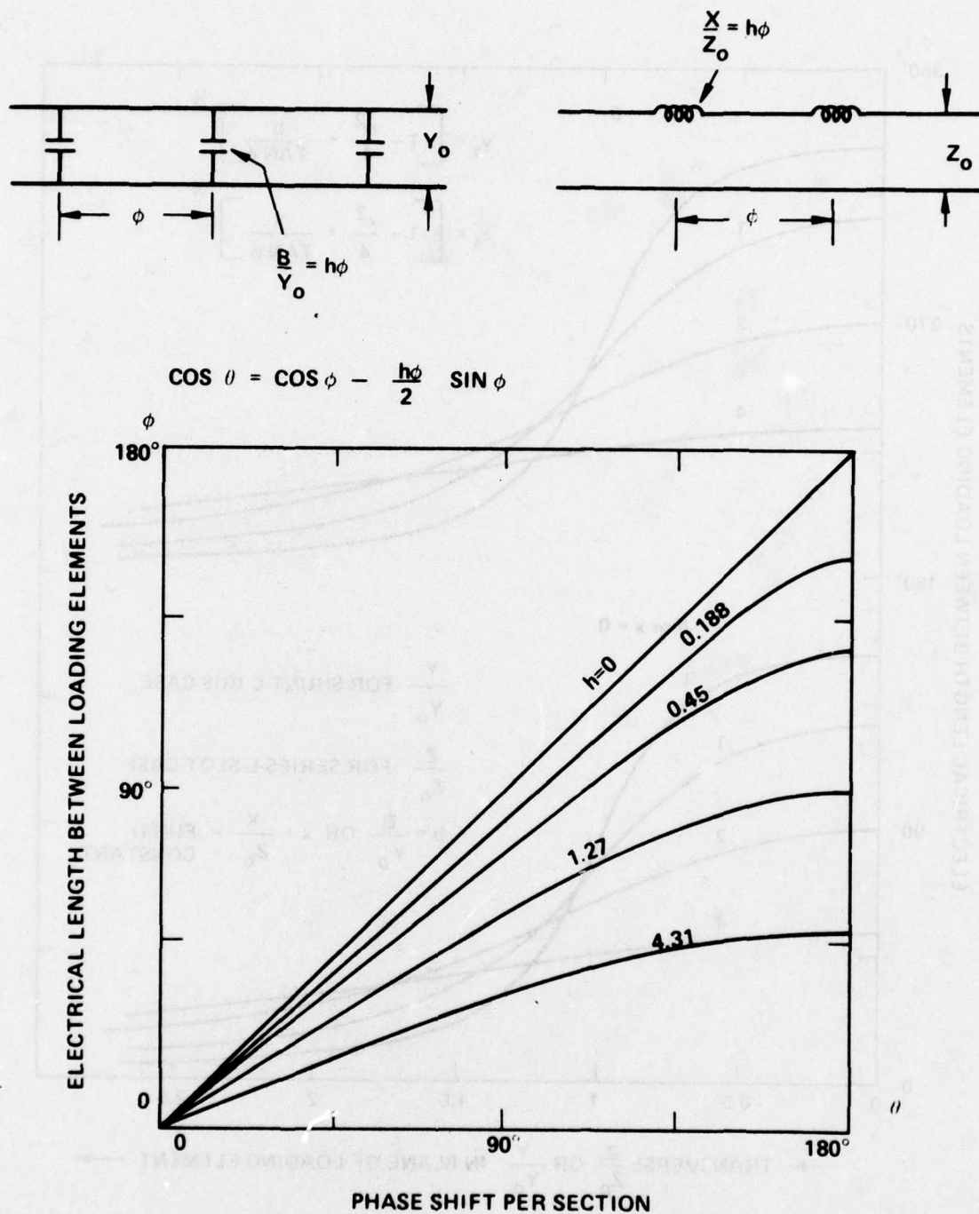
Figure 19. Brillouin-Type Diagram for Transmission Line with Periodic Loading by Either Lumped Series Inductances or Shunt Capacitances; Case 2, ratio B/Y_0 or X/Z_0 is Proportional to Electrical Length \phi .
