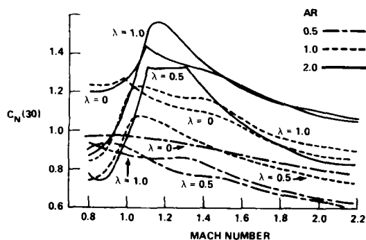
Figure 90. Chart for determining C_{N(30)}
