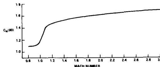
Figure 92. Chart for determining C_{N(90)}
