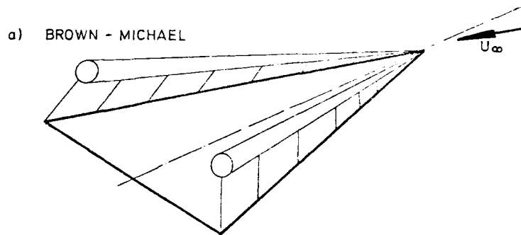
Fig.42 Vortex systems for wings
