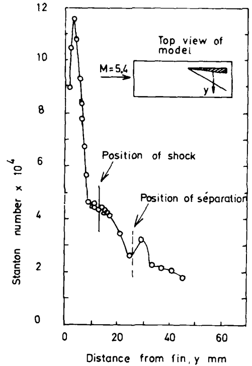
FIG. 10 HEAT TRANSFER DISTRIBUTION ON A SURFACE DUE TO A FIN AT 15^\circ , M = 5.4 . (From VKI unpublished note)
