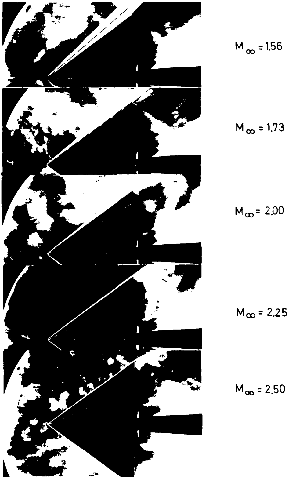
Fig. 9. Supersonic flow past a delta wing, \alpha = 0^\circ . Transition from subsonic to supersonic leading edge. H. H. Sch. Reference 10.
