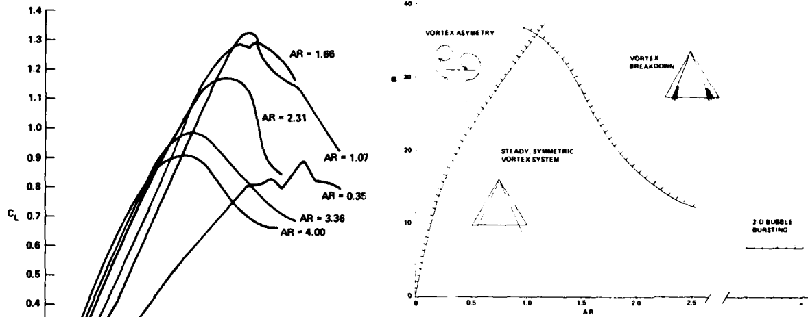
Figure 44. Vortex structures on a delta wing in incompressible flow
