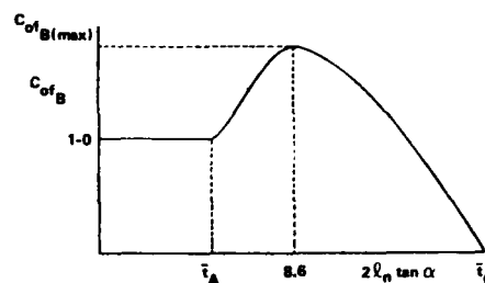
Figure 35. Amplitude of point B on the side force distribution curve. See Table 1 for definition of \epsilon_A and \epsilon_C .
