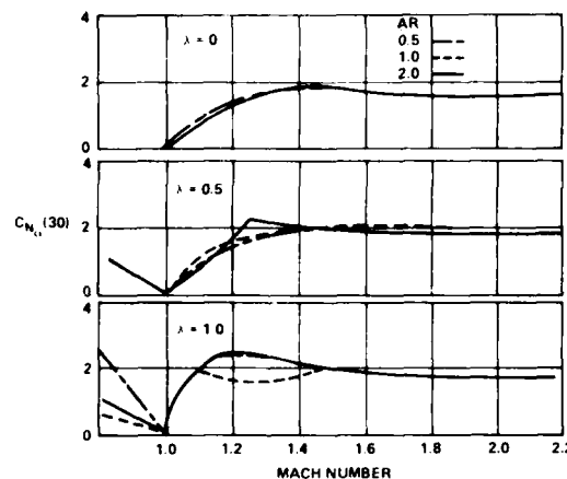
Figure 91. Chart for determining C_{N_\alpha(30)}
