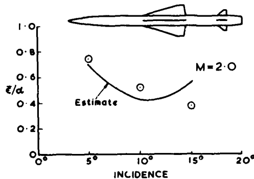
Fig 2 A comparison of experimental downwash and calculations by Plascott's method, at 45 degrees roll angle
