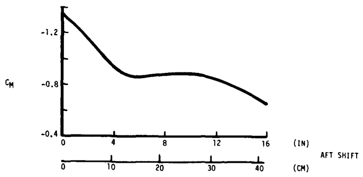
Figure 50 Change in Installed Aerodynamic Pitching Moment with Store Longitudinal Position at Transonic Speeds
