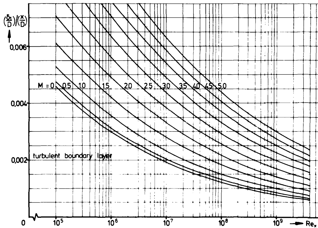
Fig. 30 Boundary layer displacement thickness on long cylinder bodies, l_z/D \geq 5
