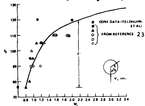
Figure 9. Steady state separation angle as a function of crossflow Mach number
