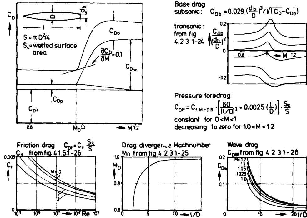
Fig. 4 Datcom method, zero-lift drag in transonic flow [4]
