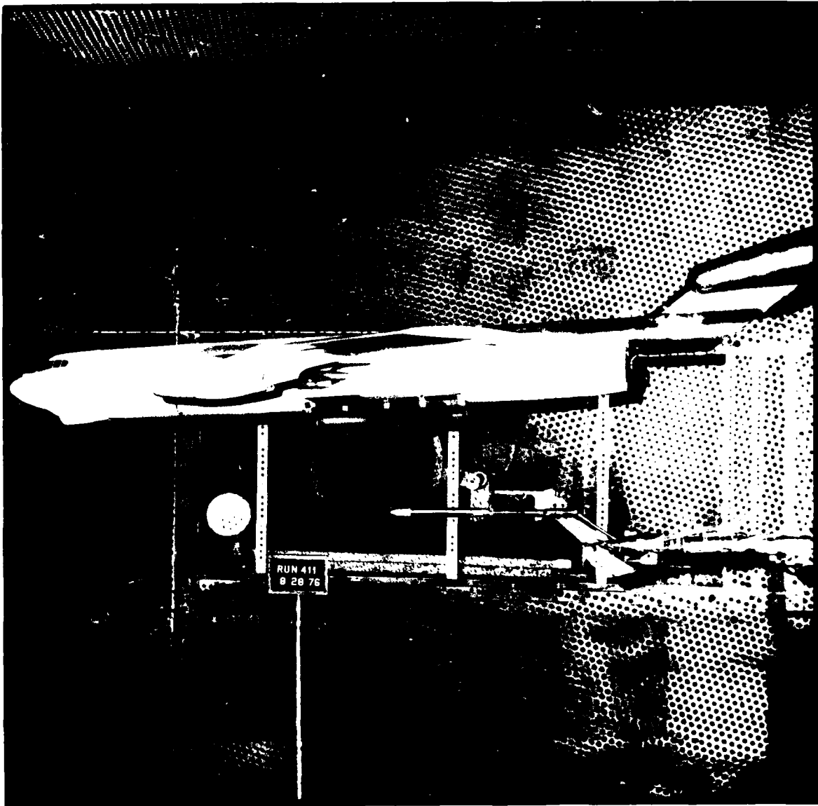
Figure 17 - CW - Calspan Corporation 8-Foot (2.4 M) Transonic Mini Tunnel
