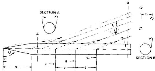
Figure 18. Terminology for Thomson and Morrison's Theory
