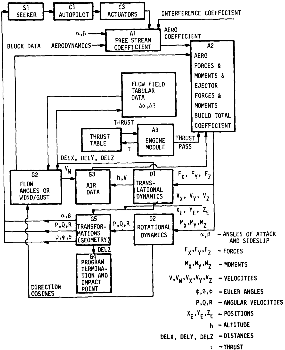
Figure 22 Block Diagram Showing Modules and Subroutines of a Typical Six-Degrees-of-Freedom Computer Simulation for Trajectory Analysis
