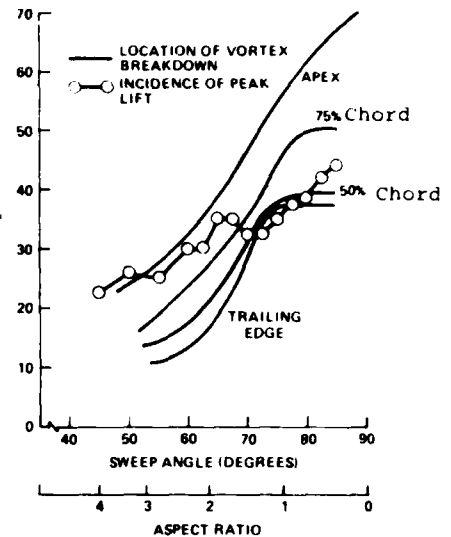
Figure 50. Vortex breakdown position and incidence of maximum lift
