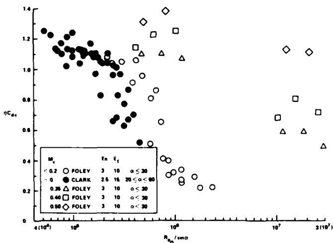
Figure 5. Measured \eta C_{Dc} on inclined bodies as a function of Reynolds number
