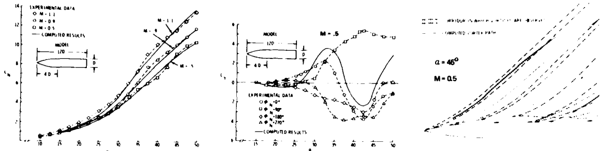
Figure 82. Results of asymmetric concentrated vortex model used in reference 81
