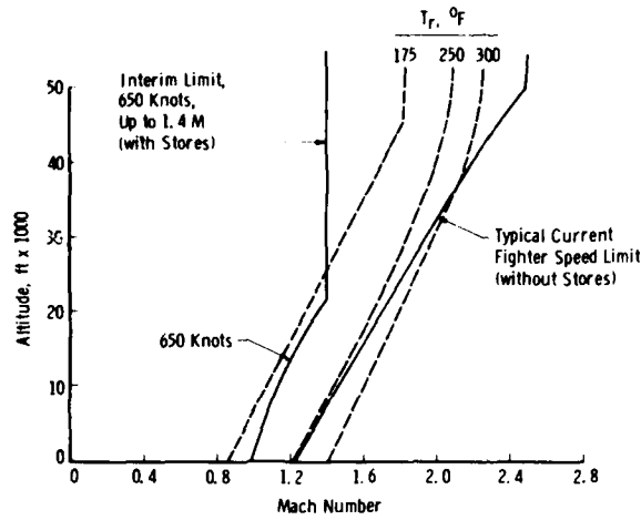
FIG. 2 PERFORMANCE ENVELOPE OF PRESENT-DAY AIRCRAFT (From Ref. 1)
