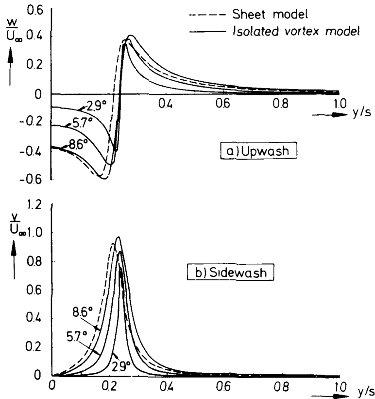
Fig.39(b) Variation of strake vortex upwash and sidewash field with incidence acc. to S.P.Fiddes and J.H.B.Smith, Reference 68
