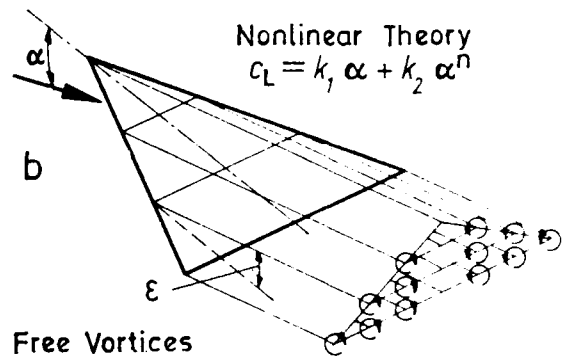
Fig.42 Vortex systems for wings
