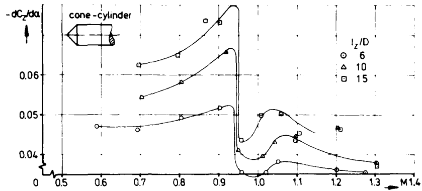
Fig. 27 Slope of normal force coefficient at \alpha=0^\circ for blunt cone cylinders, l_1/D=0.5, 0.5 \cdot 10^6 < Re_D < 1.1 \cdot 10^6 [10]
