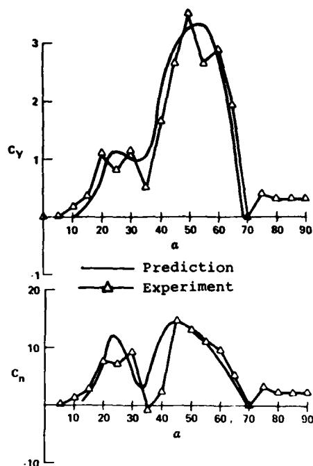
Figure 80. Predicted side force and moment by Lamont and Hunt 44 compared to the measurements of Smith and Nunn 41 on an ogive model ( l_n = 3 , l_t = 15 ). M = .13 , Re_D = 8 \cdot 10^5
