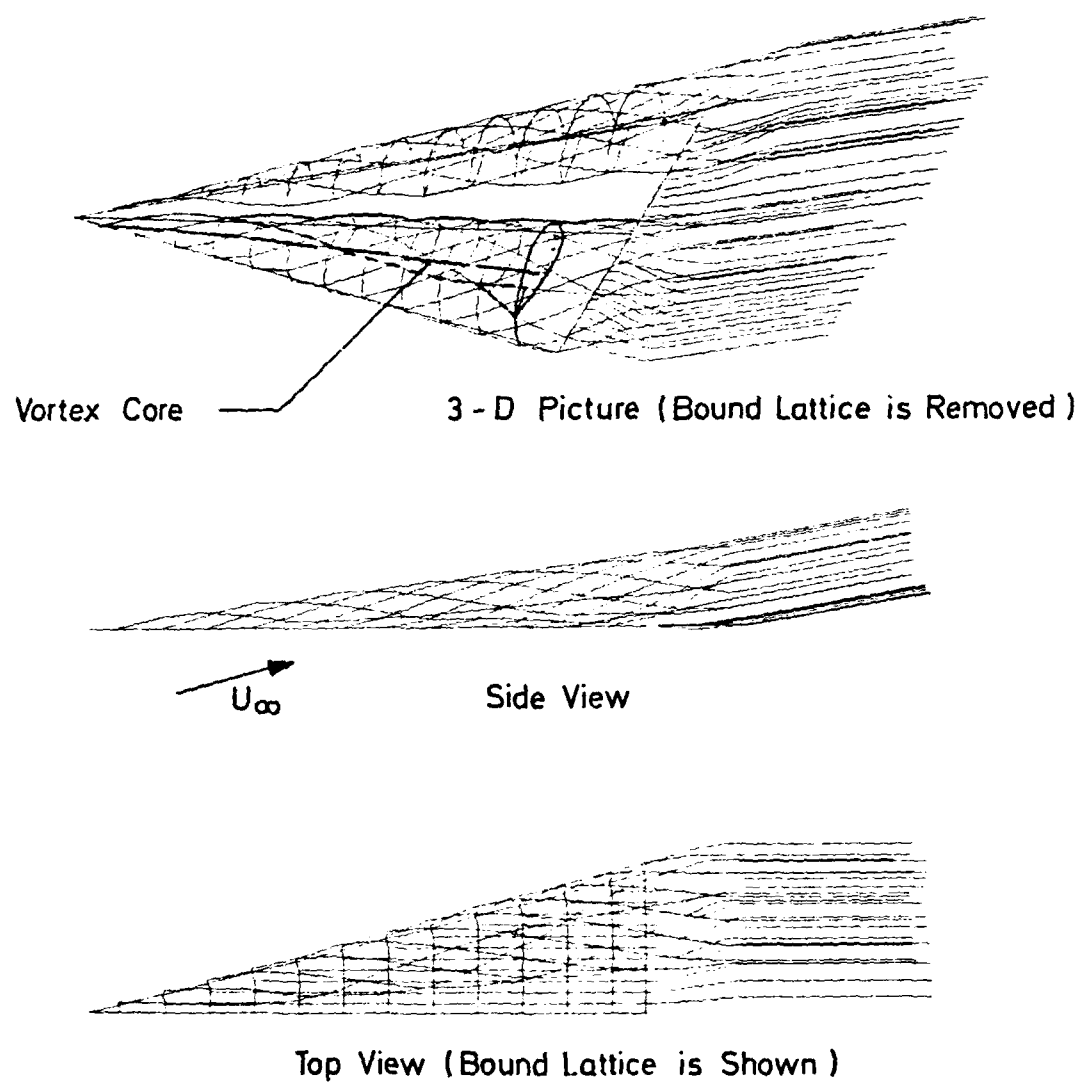
Fig.56 Wake shape of a delta wing. A = 1 , \alpha = 15^\circ , acc. to O.A.Kandil, Reference 123
