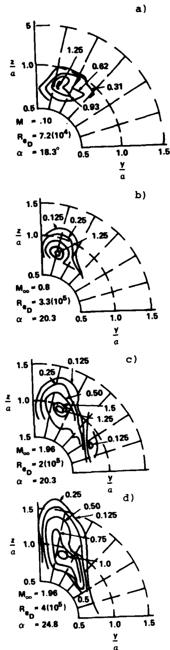
Figure 6. Crossflow plane vorticity ( Dw/4U ). Case A is from reference 11, while remainder are from reference 12. Test body was a tangent ogive, l_n = 3 , x/D = 6 .
