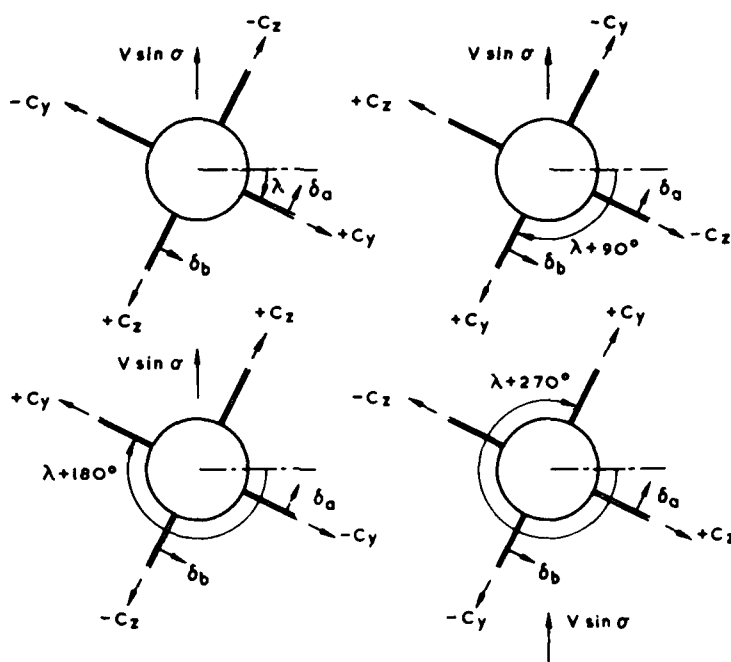
Fig 23 Symmetry relationships
