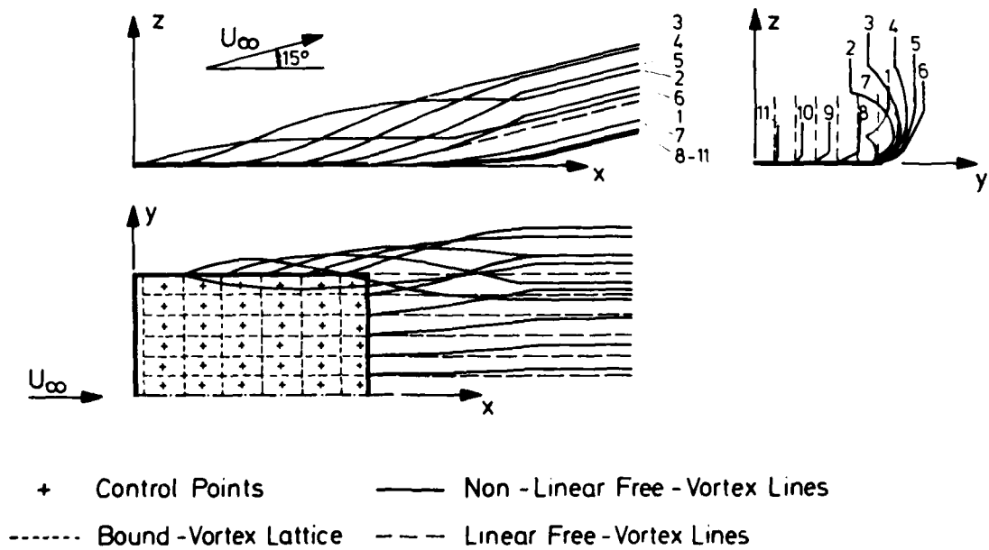
Fig.55 Wake shape of a rectangular wing. A = 1 , acc. to O.A.Kandil, Reference 99
