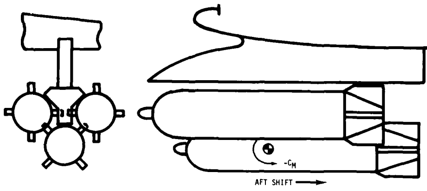
Figure 49 Effects of Varying Static Aerodynamic Stability on Store Pitch
