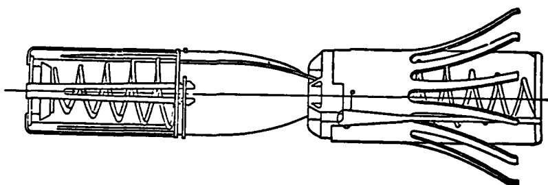
FIG.4. CLUSTER BOMBLET
