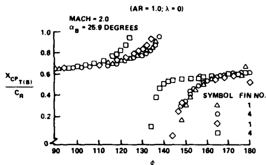
Figure 61. Near the roll orientation where C_N = 0 , center of pressure measurements are difficult to duplicate 58 (See Figure 60 for definition of symbols)
