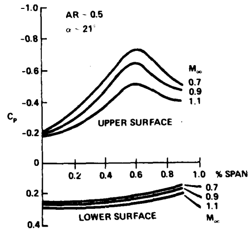
Figure 52. Influence of compressibility on delta wing surface pressure. Reported in reference 49 using the results of reference 52
