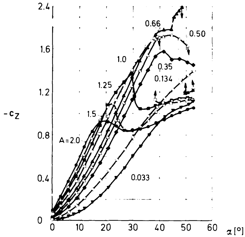
Fig.30 Normal force coefficient for rectangular plates of various aspect ratios, from Reference 40
