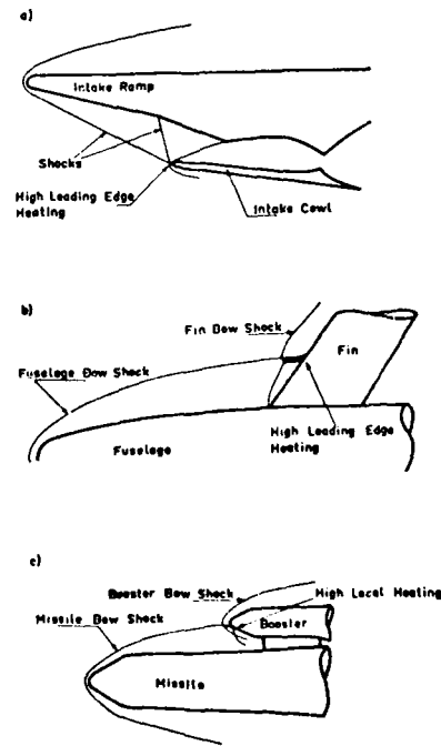
FIG. 7 PRACTICAL EXAMPLES OF SHOCK IMPINGEMENT HEATING
