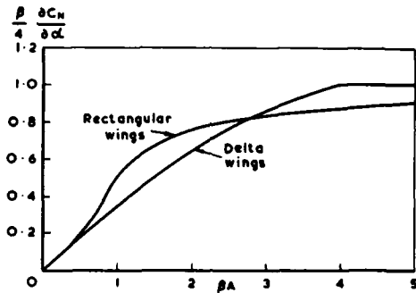
FIG.4 SUPERSONIC LINEAR THEORY LIFT SLOPE FOR THIN WINGS
