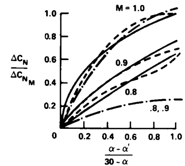
Figure 89. Chart for determining \Delta C_N/\Delta C_{N_M} ; — \lambda=1 --- \lambda=0.5 , -·- \lambda=0 .
