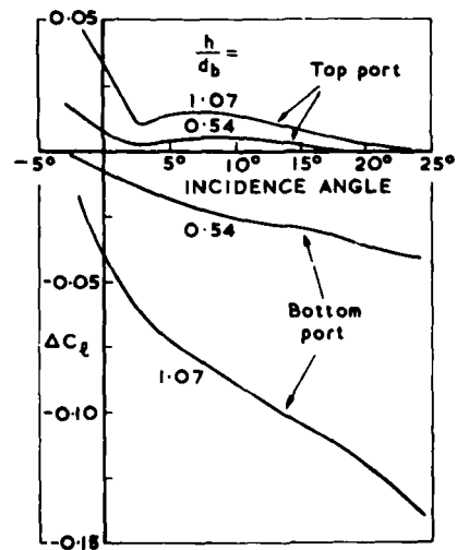
Fig 34 Change in rolling moment due to individual swept spoilers, M = 4.3 (Ref 22)
