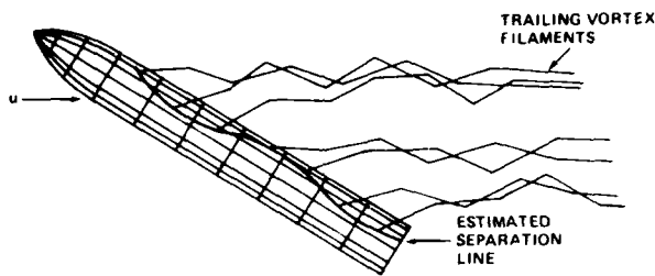
Figure 85. Three dimensional vortex model. Distributed sources are used to satisfy boundary conditions and the flow field is modeled using vortex filaments.
