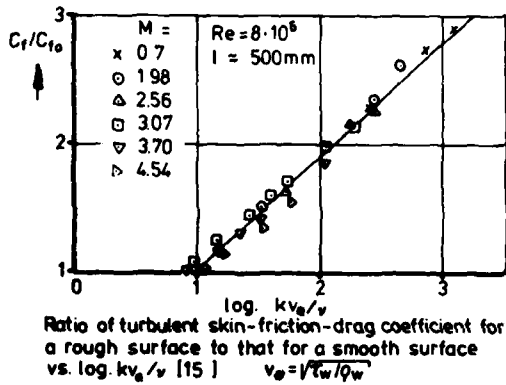
Fig.15 Influences of roughness and heat transfer on turbulent skin friction
