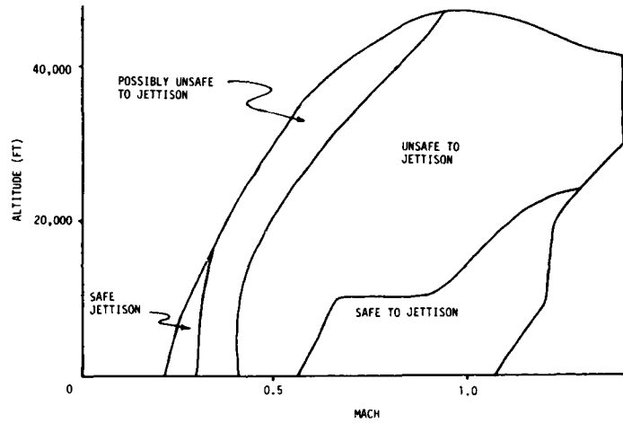
Figure 61 F-4 Jettison Envelope - Nominal Weight Aircraft
