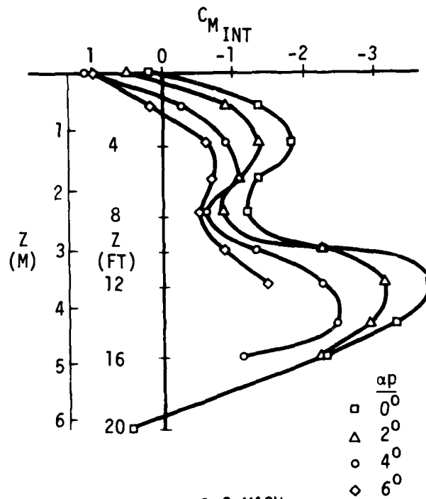
Figure 11 Variation in Interference Pitching Moment Coefficient with Store Vertical Displacement - F-4 Aircraft, 0.8 and 1.2 Mach
