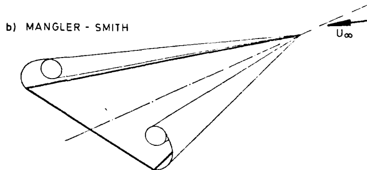
Fig.43 Flow models for slender delta wings (a) Brown-Michael. (b) Mangler-Smith
