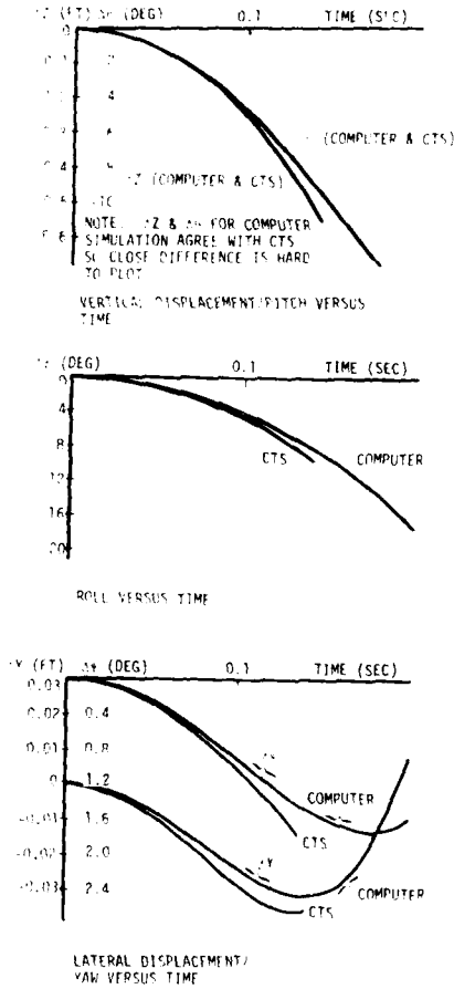
Figure 57 Comparison of CTS and Computer Simulation - Control System Off
