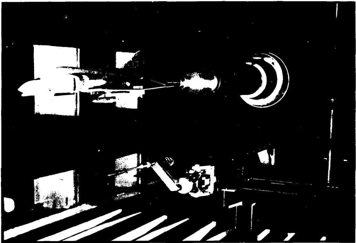
Figure 11. The interior of the wind tunnel, showing the model and the flow direction.
