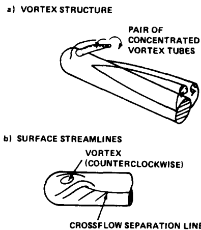
Figure 14. Nose Vortex Structure at \alpha \sim 19^\circ on a Blunt Body in Transonic Flow
