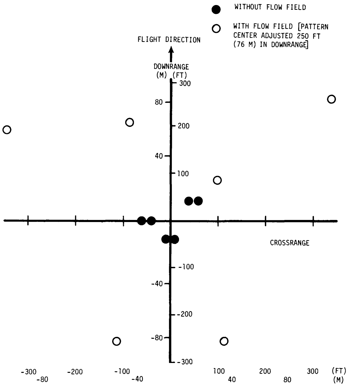
Figure 55 Flow Field Effect on the Impact Pattern of Six M-117 Bombs Released in Ripple Pairs - 40 MS from F-4 Inboard Wing Station TERs - 5,000 Feet/0.9 Mach
