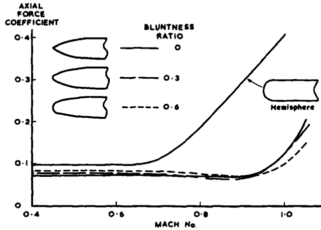
FIG. 12 EFFECT OF NOSE BLUNTNES ON AXIAL FORCE
