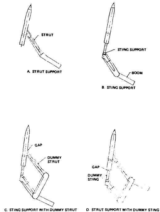
Figure 62. Model support systems tested in reference 61
