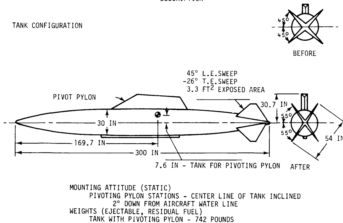
Figure 33 FB-111A 600-Gallon (2271 Litre) Tank/Pylon
