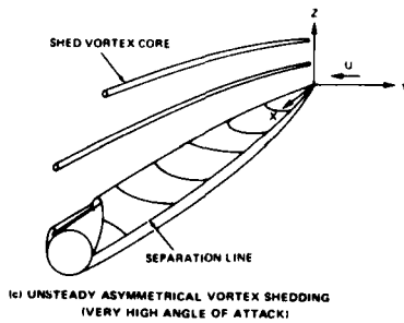
Figure 1. Leeward vortex structure in subsonic flow
