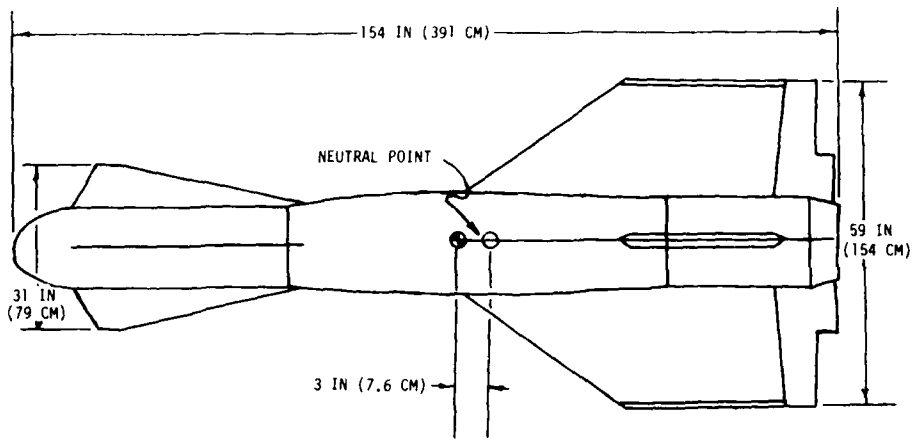
Figure 63 Revised Guided Weapon Design
