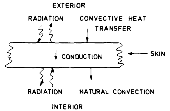
FIG. 3 THE GENERAL HEAT TRANSFER PROBLEM
