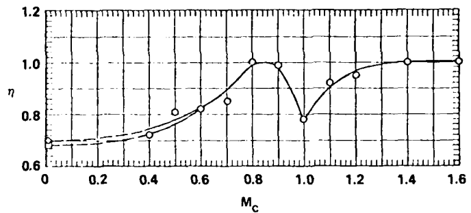
Figure 70. Correction factor of calculate from experimental data on inclined bodies with Re_T \sim 10
