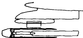
Figure 20 Four Modes to Investigate Store Afterbody Alteration and Sting Interference Effects
