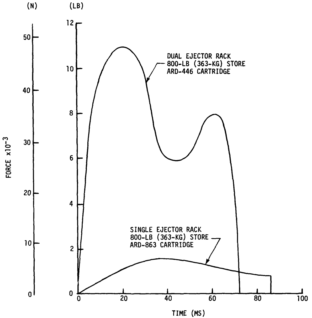
Figure 4 Impulse Performance of Typical Single and Dual Ejector Racks
