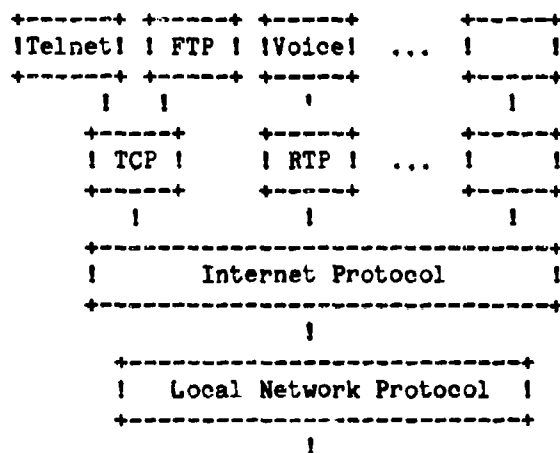
Protocol Relationships
