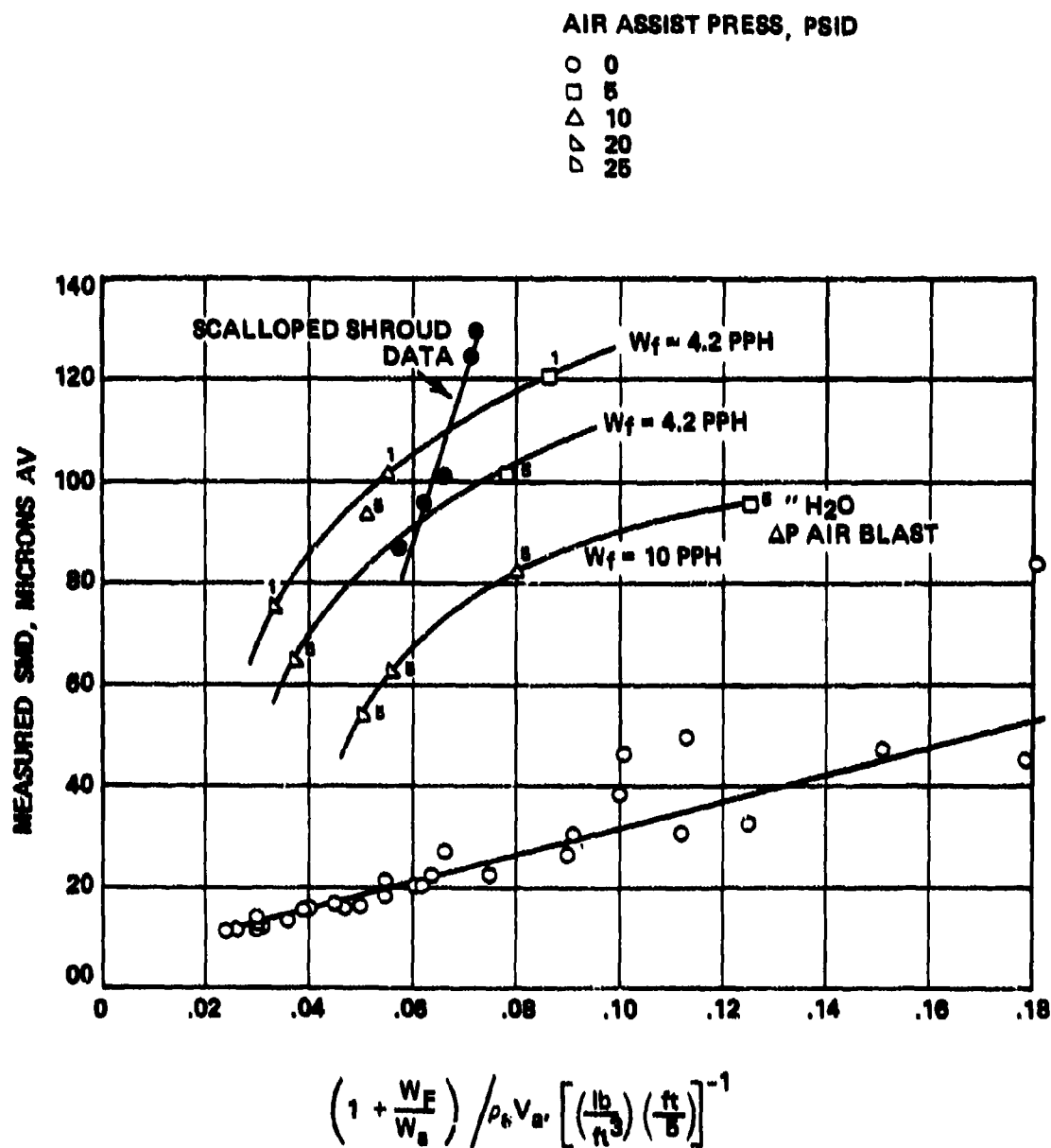
Figure 101. Measured SMD Data of Airblast Nozzle with Different Linear \Delta P and Air-Assist \Delta P .
