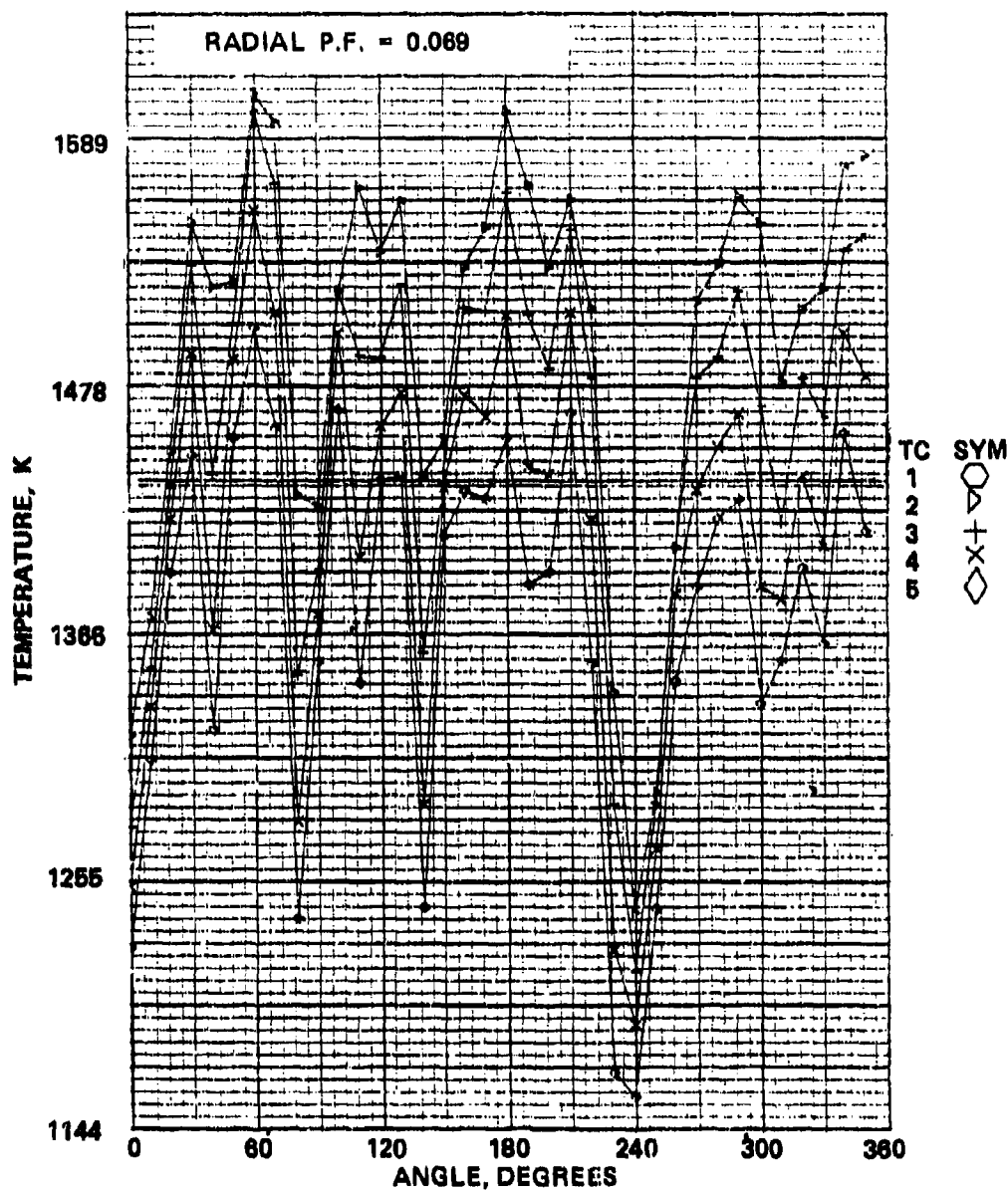
Figure 67. Exhaust-Temperature Scan of Concept II -1 Combustor at Sea-Level, 75-Percent Power Point with Cooled Unscaloped Nozzle Shrouds ( \alpha=90^\circ ) and Air-Assist \Delta P = 0 .
