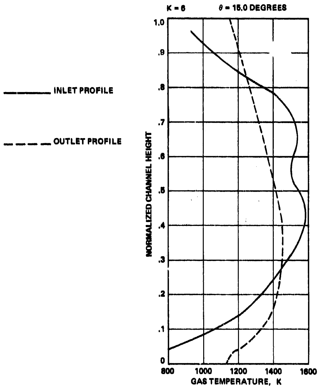
Figure 116. Predicted Stator Inlet Temperature Profiles of Concept I for the Planes \theta = 15, 18, 21 and 24 Degrees (Sheet 1 of 4).
