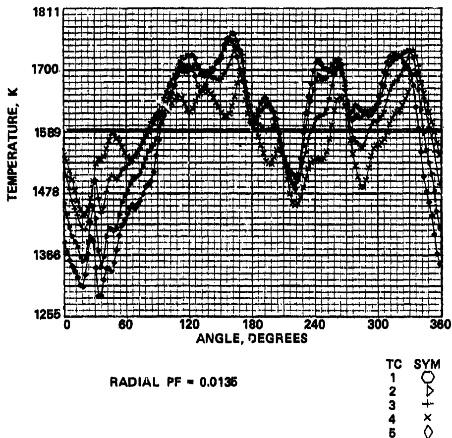
Figure 25. Concept I Combustor Sea-Level, Hot-Day Temperature Scan.
