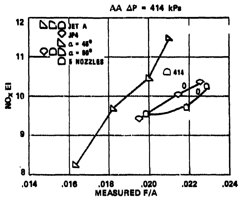
Figure 22. NO_x Emission Index Versus Fuel/Air Ratio of Concept I at Sea-Level, 55-Percent Power point.
