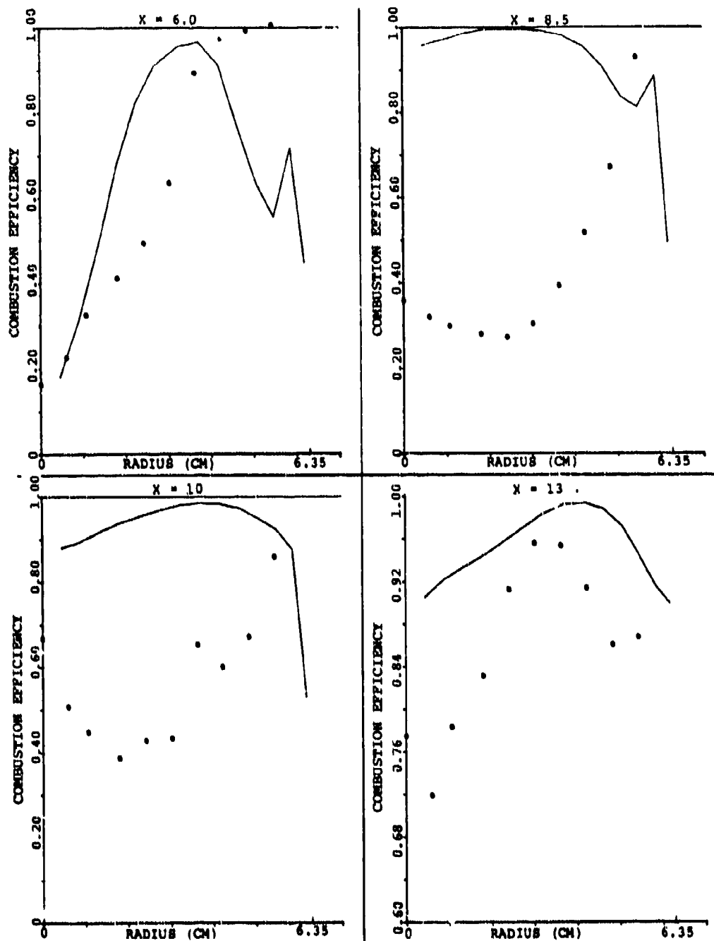
Figure 144. Comparison Between Predicted and Measured Combustion Efficiency for the X-Y Planes In Between the Primary Jet for Set-7 of Table 15 (Sheet 1 of 2).
