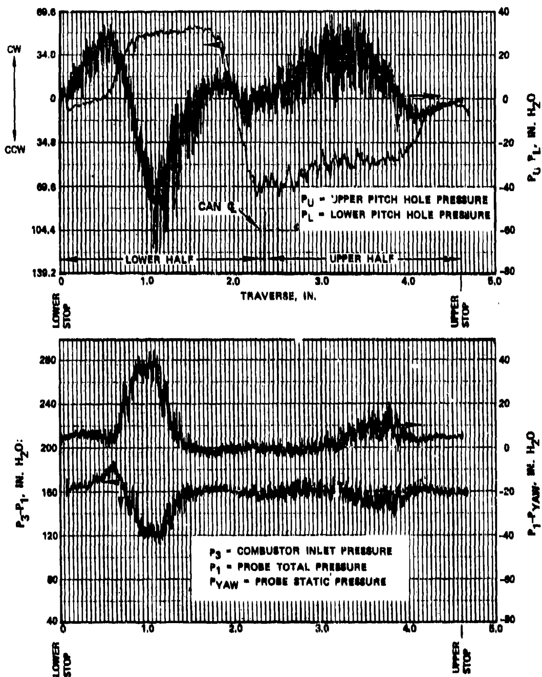
Figure 47. Typical Pressure and Yaw Angle Traces.
