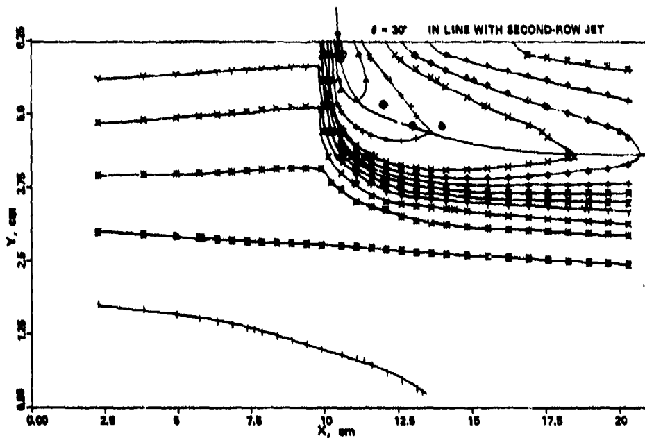
Figure 97. Comparison Between Predicted and Measured Jet Trajectories of Two Staggered Rows of Six-Opposing Jets; Jet Momentum Ratio = 4.5.
