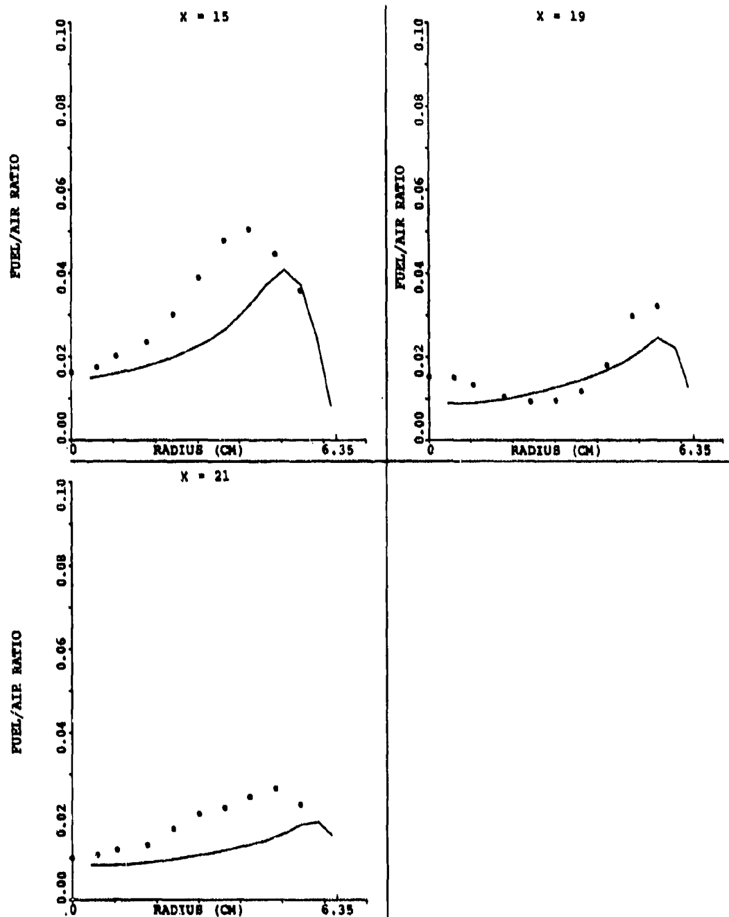
Figure 117. Comparison Between Predicted and Measured Profiles of Fuel/Air Ratio Along \theta = 0^\circ for Set-2, Table 15 (Sheet 2 of 2).
