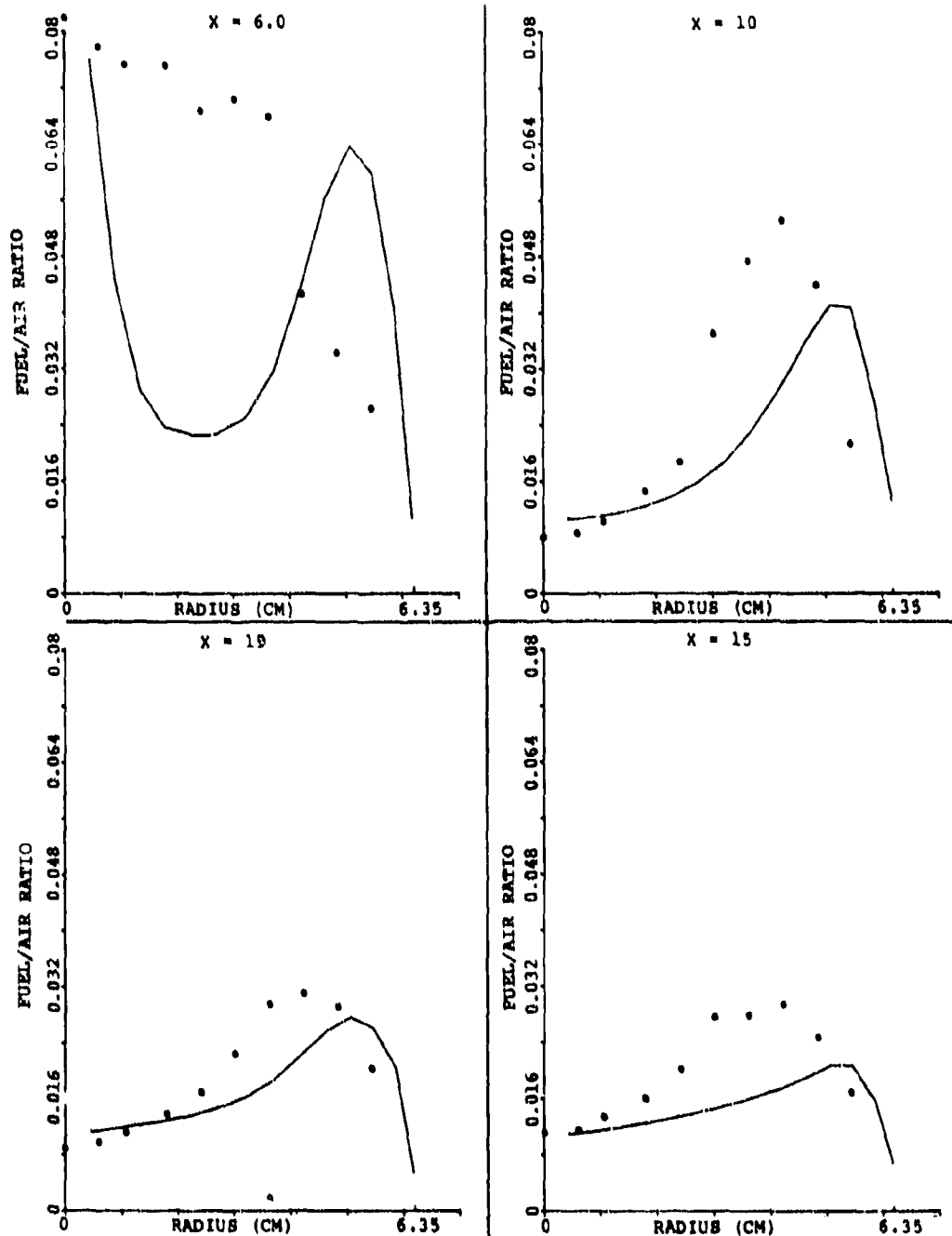
Figure 133. Comparison Between Predicted and Measured Profiles of Fuel/Air Ratio for the X-Y Planes In Between the Primary Jet for Set-8 of Table 15 (Sheet 1 of 2).
