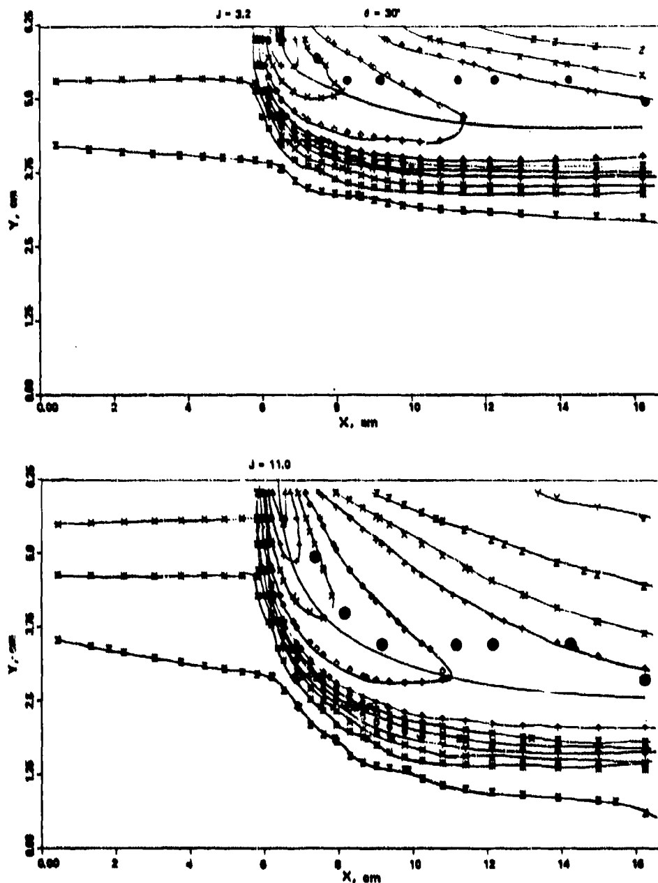
Figure 91. Comparison Between Predicted and Measured Jet Trajectories of Six-Opposing Jets With Jet Momentum Ratio As a Parameter. (Sheet 1 of 3)
