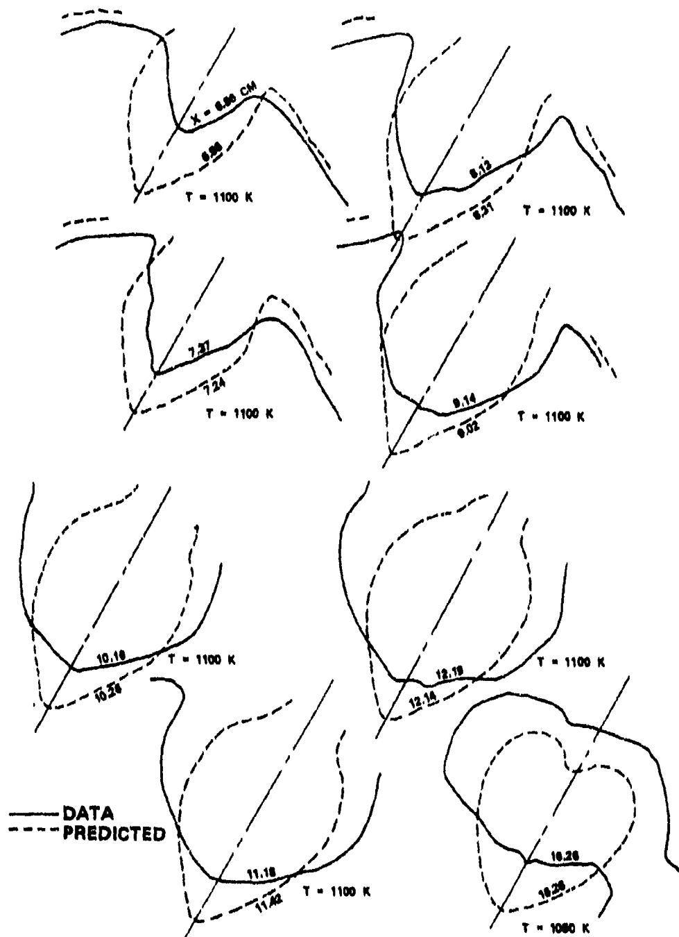
Figure 93. Comparison Between Predicted and Measured Isothermal Lines of a Six-Opposing Jet, J = 11.0 , Set-2 of Table 11.
