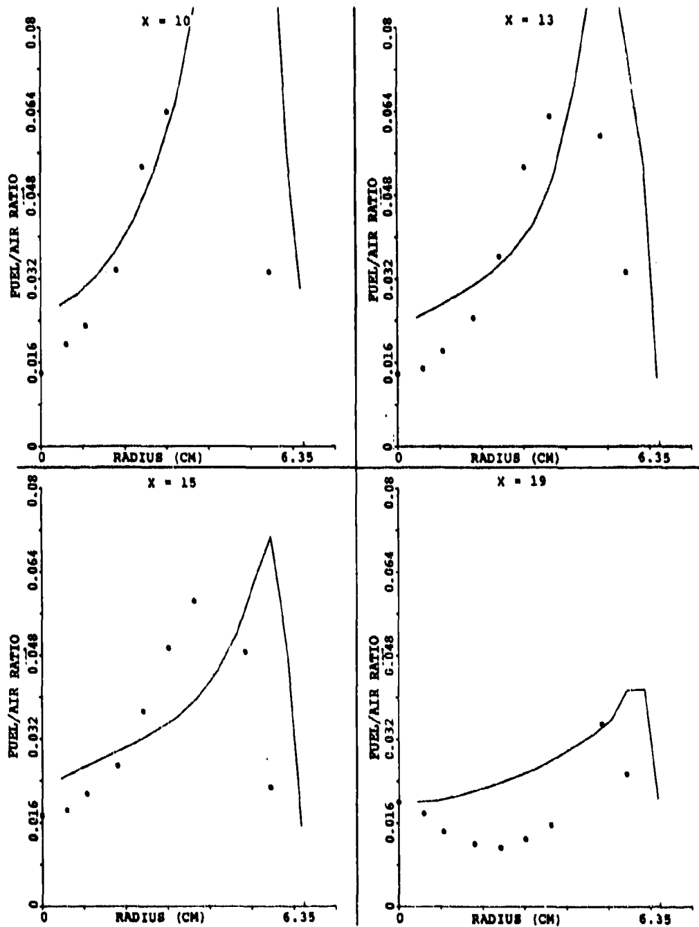
Figure 147. Comparison Between Predicted and Measured Profiles of Fuel/Air Ratio for the X-Y Planes In Between the Primary Jet for Set-10 of Table 16 (Sheet 1 of 2).
