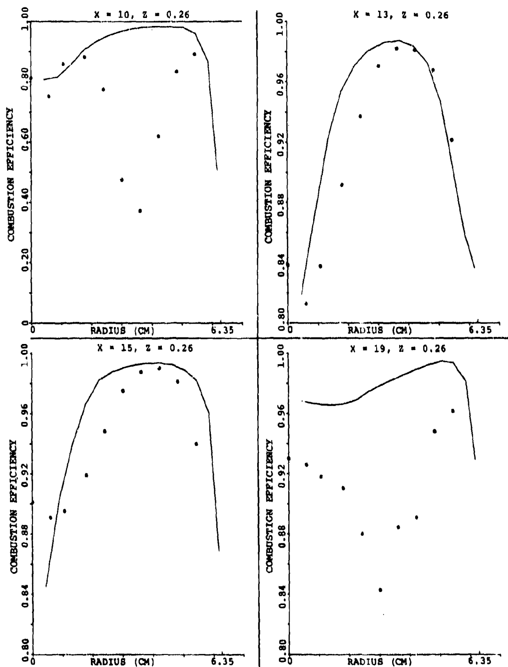
Figure 129. Combustion Efficiency Profiles for the \theta = 15^\circ Planes for Set-8 of Table 16 (Sheet 1 of 2).
