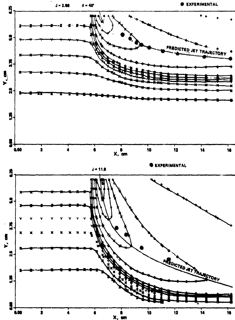
Figure 86. Comparison Between Predicted and Measured Jet Trajectories of Four-Opposing Jets With Jet Momentum Ratio As a Parameter; Refer to Table 10 for Other Details.
