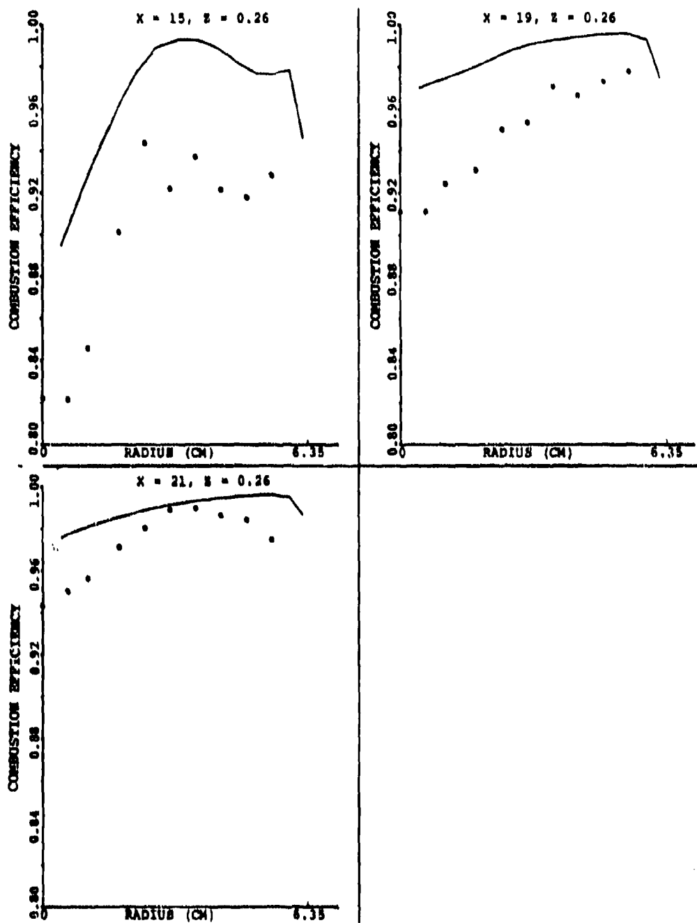
Figure 121. Comparison Between Predicted and Measured Combustion Efficiency Along \theta = 15^\circ for Set-2, Table 15 (Sheet 2 of 2).
