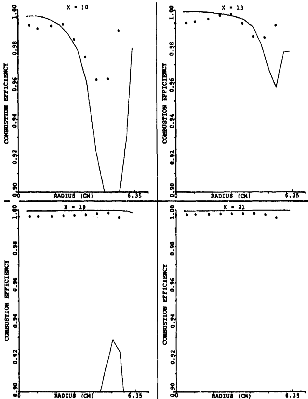
Figure 150. Comparison Between Predicted and Measured Combustion Efficiency for the X-Y Planes In Between the Primary Jet for the Set-11 of Table 16.
