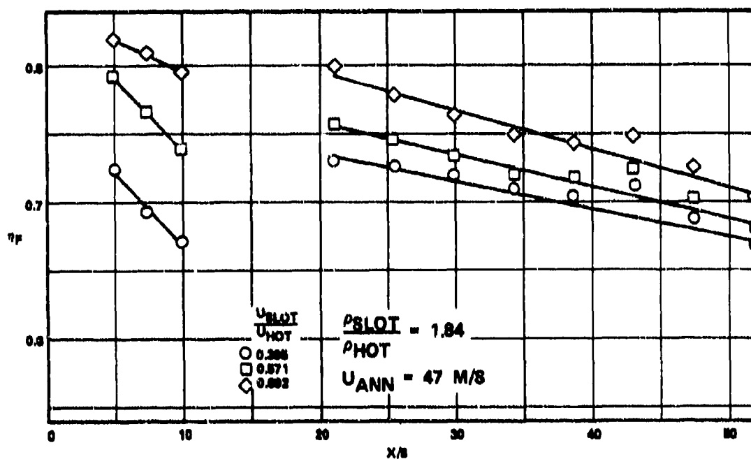
Figure 26. Performance of Film/Extended Surface Convection Cooling Scheme.
