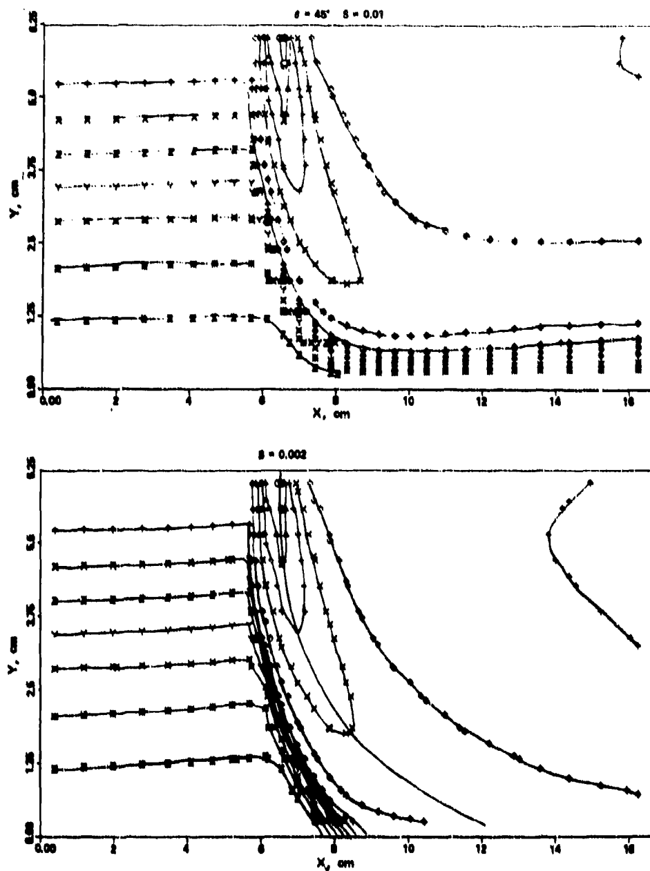
Figure 83. Effect of Cumulative Mass Residual (S) on Predicted Isothermal Profiles of Set-3 of Table 10.
