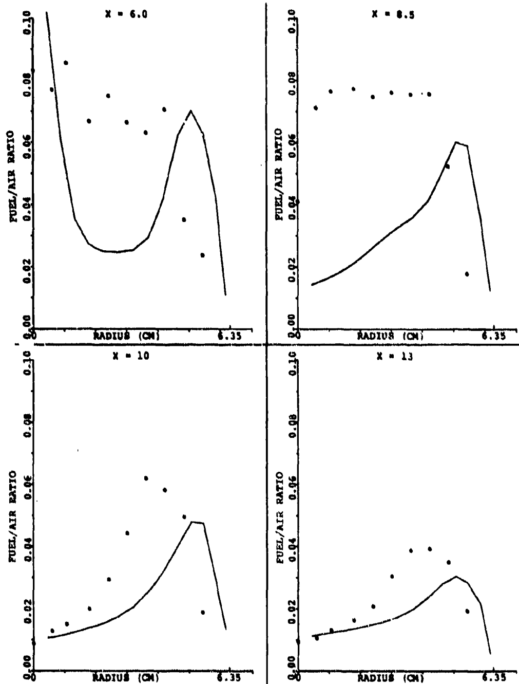
Figure 141. Comparison Between Predicted and Measured Profiles of Fuel/Air Ratio for the X-Y Planes In Between the Primary Jet for Set-5 of Table 15 (Sheet 1 of 2).
