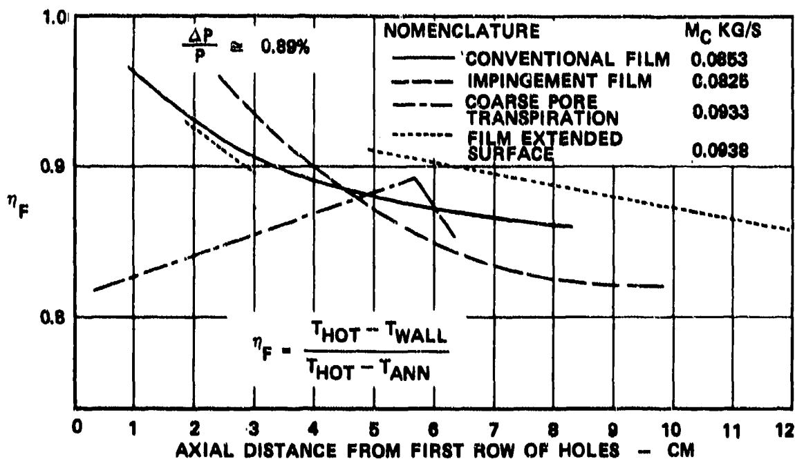
Figure 31. Comparison of the Four Cooling Schemes in Nonreacting Flow Fields.
