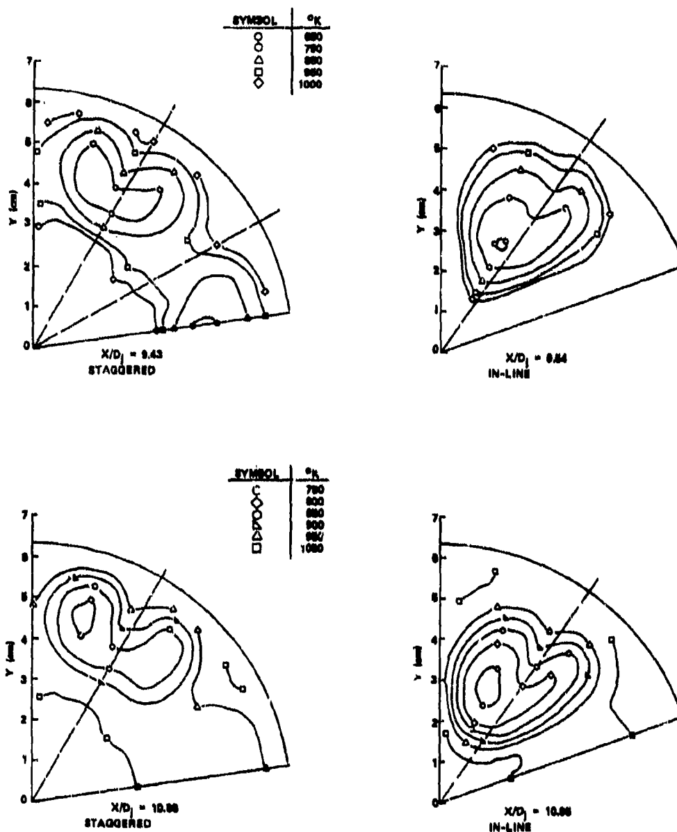
Figure 36. A Typical Comparison Between Mixing Characteristics of In-Line and Staggered Rows of Dilution Jets in the Region Downstream of the Second Row (Sheet 2 of 2).
