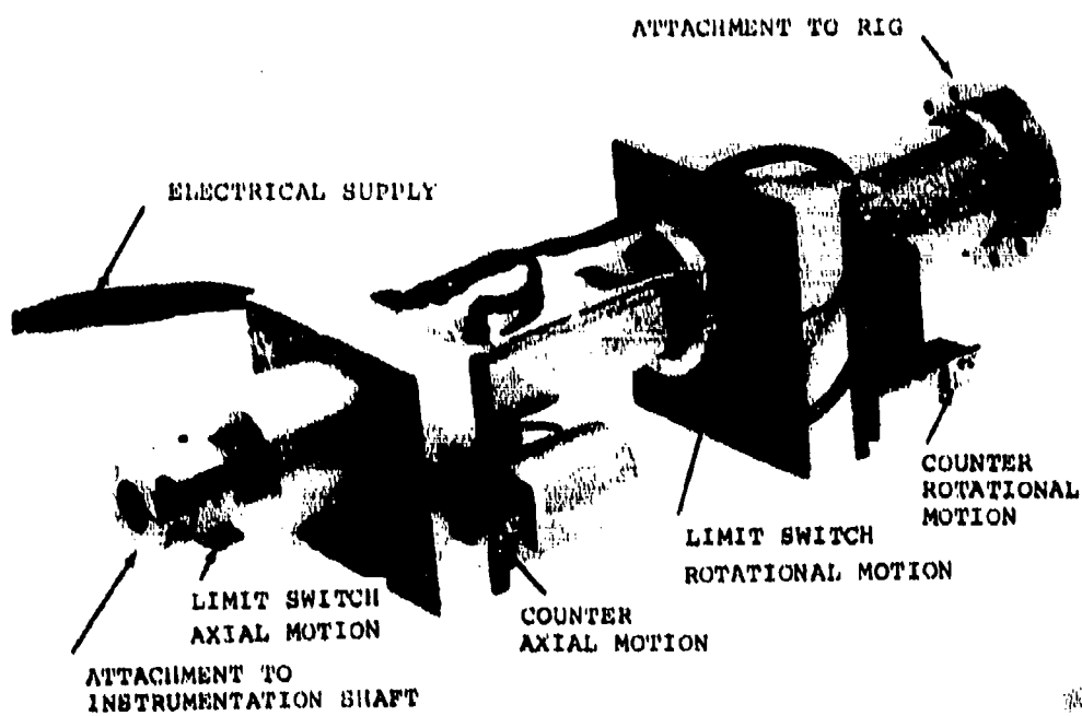
Figure 10. Probe Actuator.
