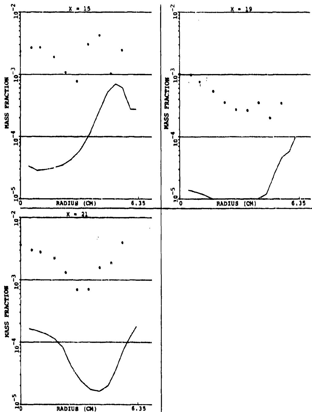
Figure 110. Comparison Between Predicted and Measured Unburned Fuel at Different X-Y Planes ( \theta = 0^\circ ) In Between Primary Jet ( \theta = 30^\circ ) for Set-2, Table 15. (Sheet 2 of 2)
