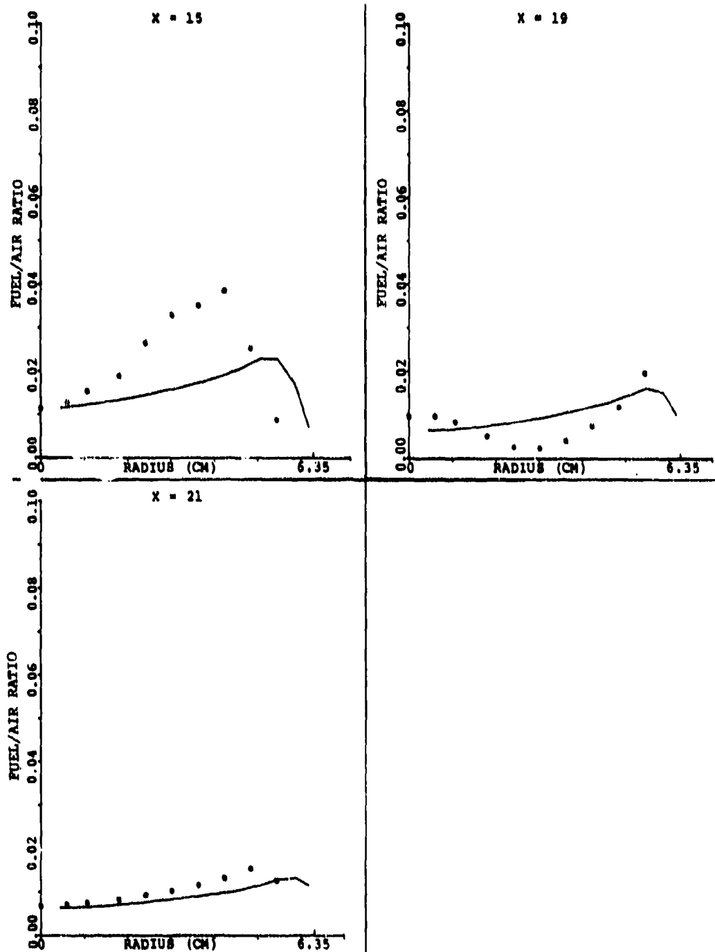
Figure 141. Comparison Between Predicted and Measured Profiles of Fuel/Air Ratio for the X-Y Planes In Between the Primary Jet for Set-5 of Table 15 (Sheet 2 of 2).
