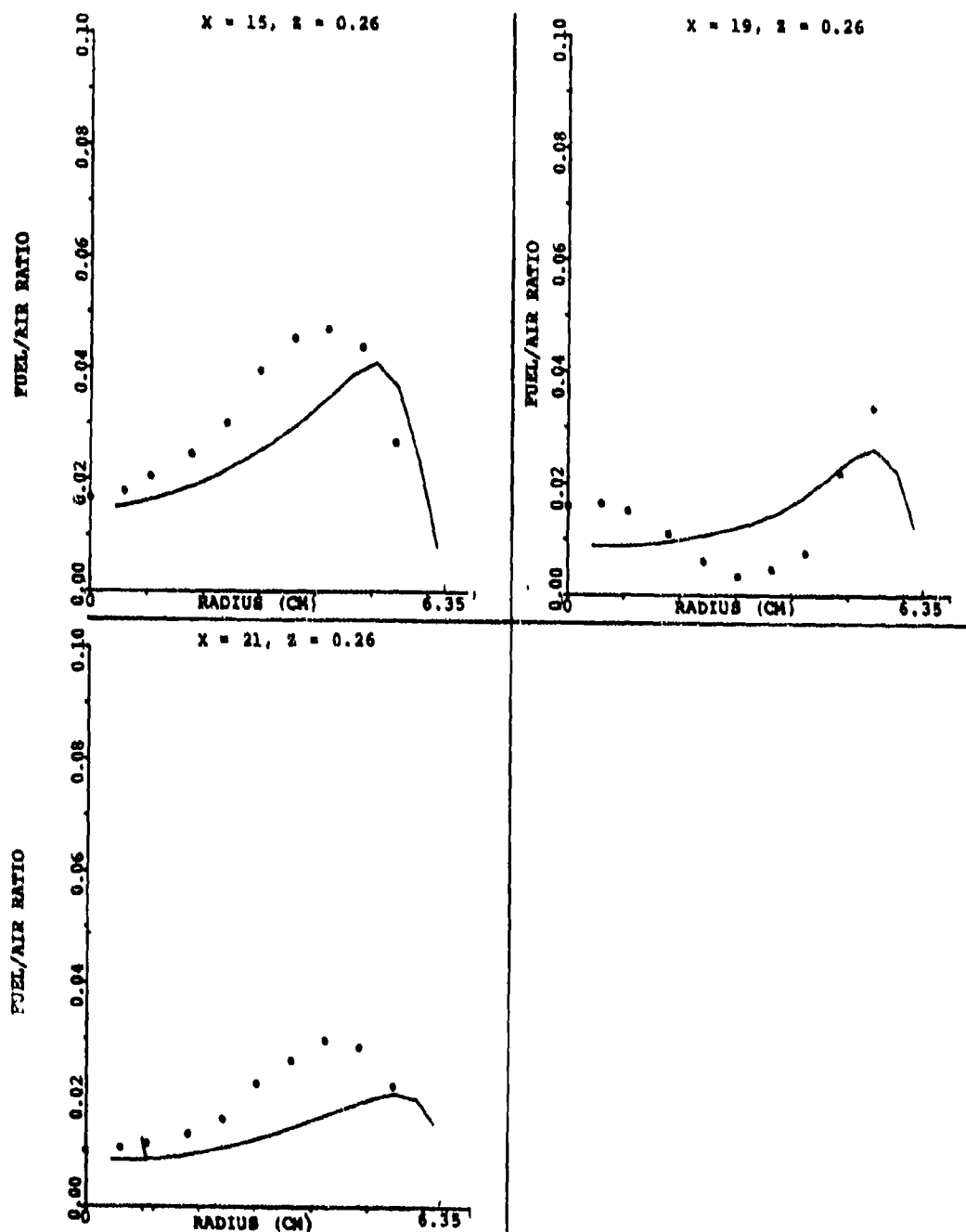
Figure 118. Comparison Between Predicted and Measured Profiles of Fuel/Air Ratio Along \theta = 15^\circ for Set-2, Table 15 (Sheet 2 of 2).
