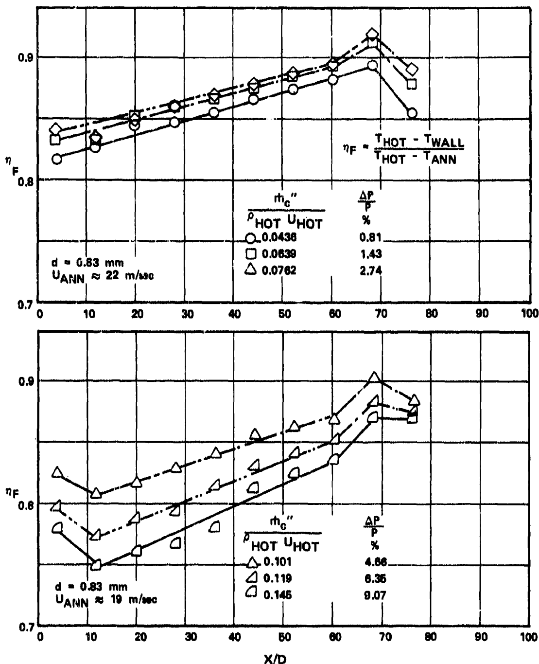
Figure 29. Performance of Coarse-Pore Transpiration Cooling Scheme.
