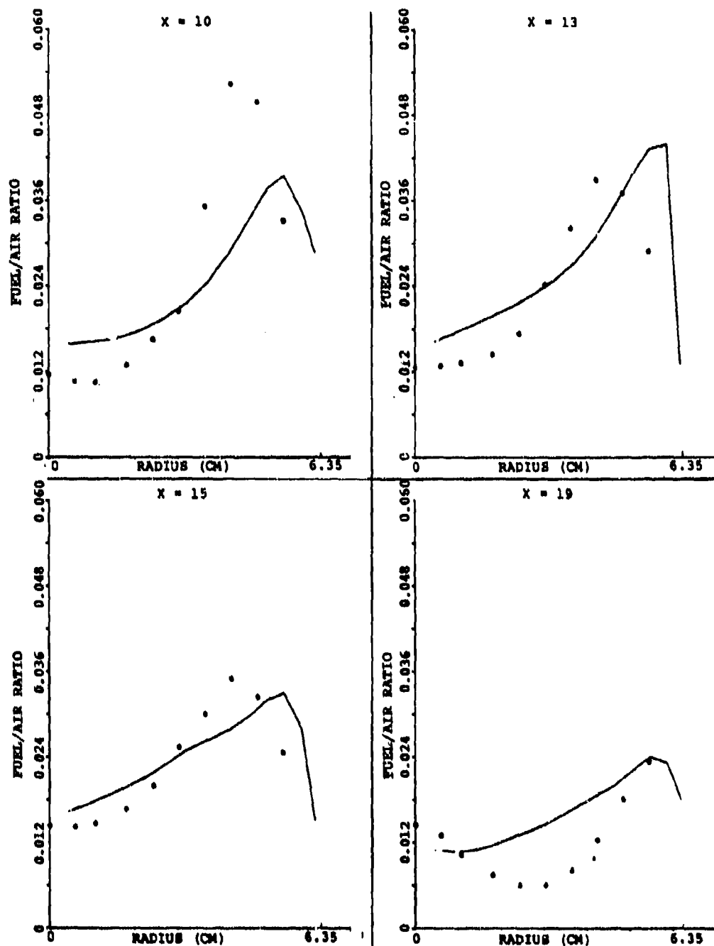
Figure 125. Comparison Between Predicted and Measured Profiles of Fuel/Air Ratio for the X-Y Planes ( \theta = 0 ) In Between Primary Jet ( \theta = 30^\circ ) for Set-8 of Table 16 (Sheet 1 of 2).
