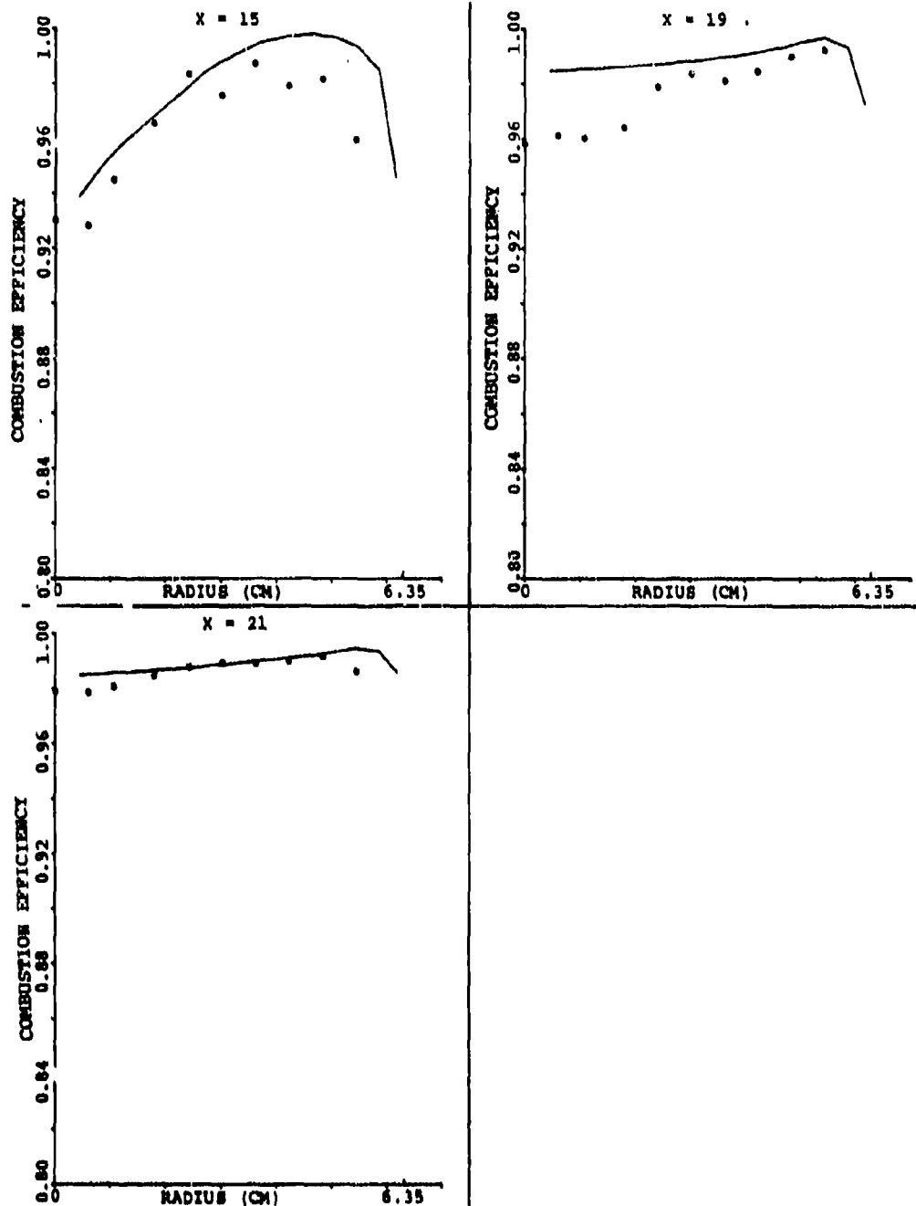
Figure 142. Comparison Between Predicted and Measured Combustion Efficiency for the X-Y Planes In Between the Primary Jet for Set-5 of Table 15 (Sheet 2 of 2).
