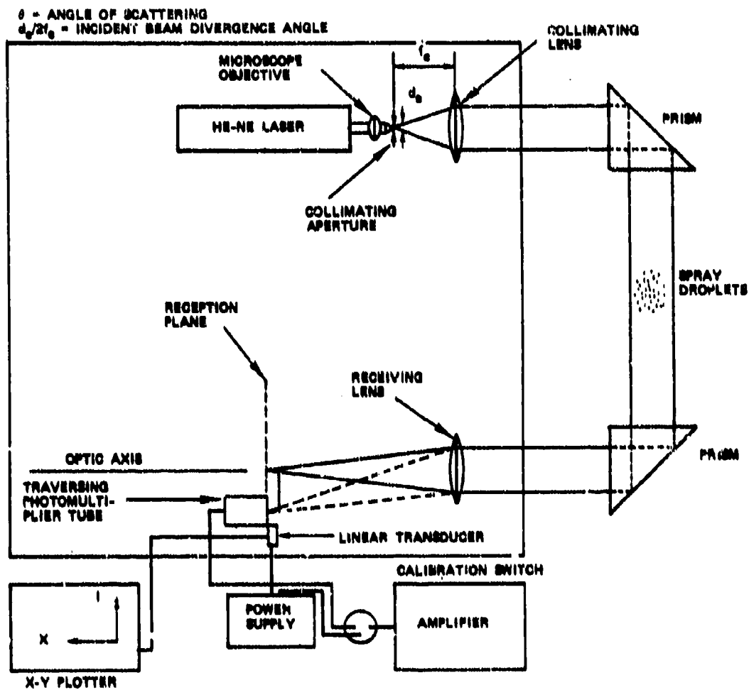
Figure 62. Schematic of Optical Apparatus used in Light-Scattering Technique.
