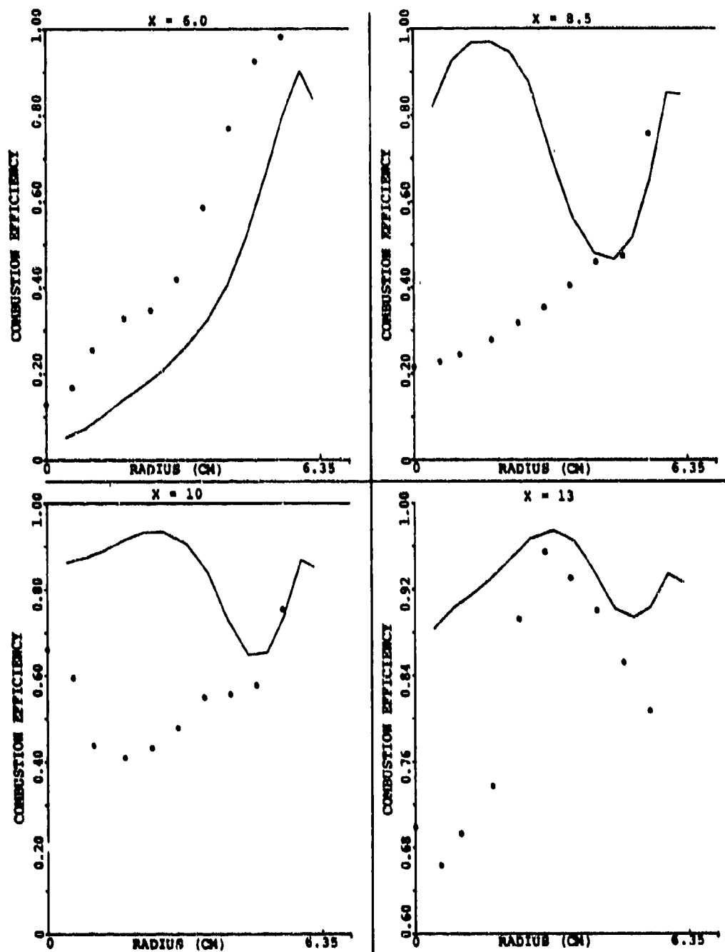
Figure 120. Comparison Between Predicted and Measured Combustion Efficiency Along \theta = 0^\circ for Set-2, Table 15 (Sheet 1 of 2).
