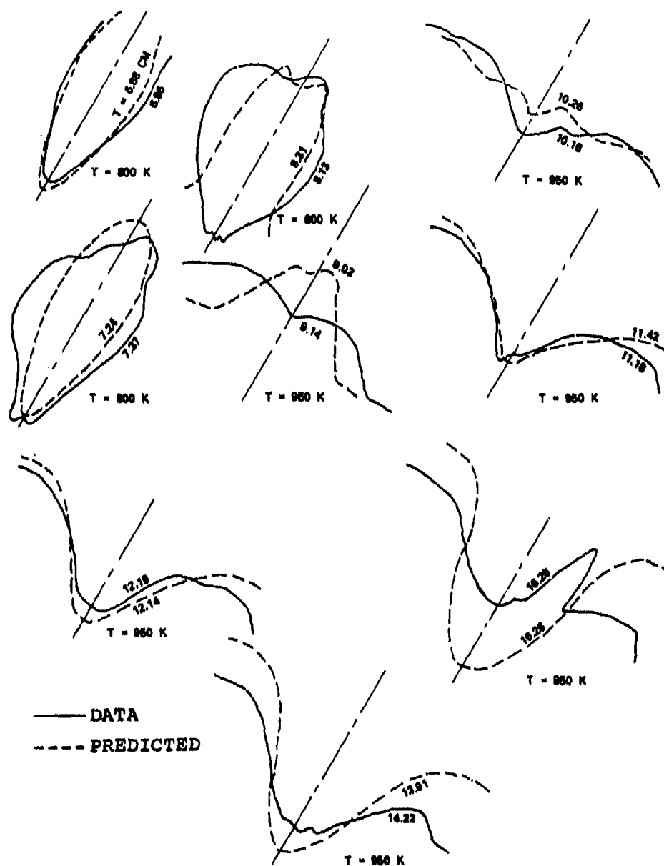
Figure 96. Comparison Between Predicted and Measured Isothermal Lines of a Six-Opposing Jet, T = 61.1 , Set-5 of Table 11.
