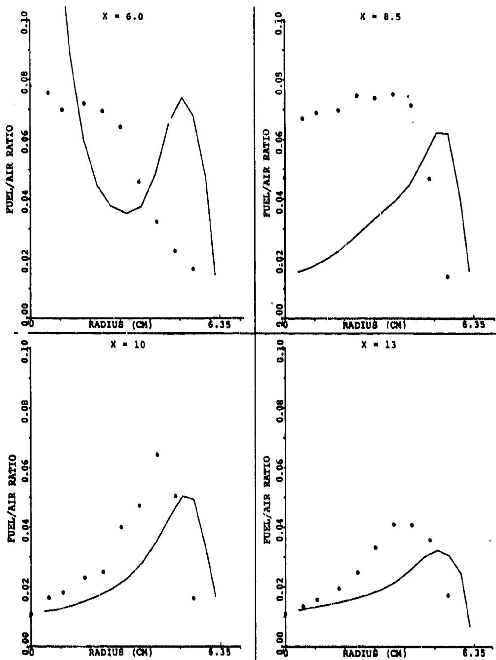
Figure 143. Comparison Between Predicted and Measured Profiles of Fuel/Air Ratio for the X-Y Planes In Between the Primary Jet for Set-7 of Table 15 (Sheet 1 of 2).
