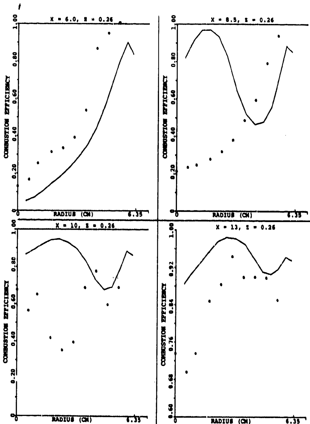
Figure 121. Comparison Between Predicted and Measured Combustion Efficiency Along \theta = 15^\circ for Set-2, Table 15 (Sheet 1 of 2).
