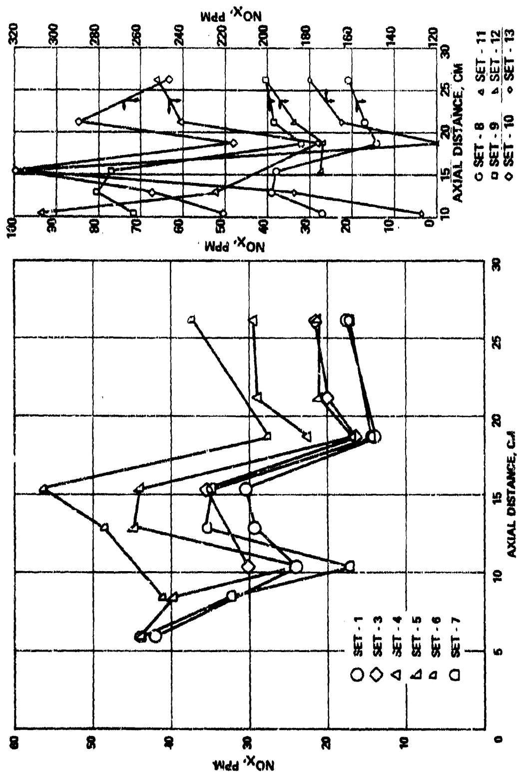
Figure 59. Average Profiles for NO x for Set-1 Through Set-13.
