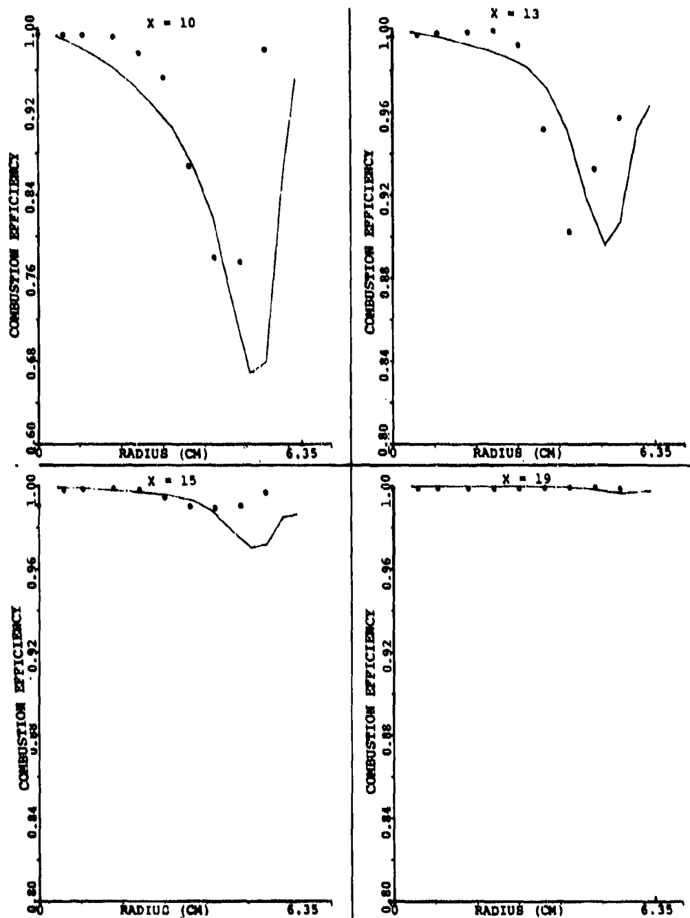
Figure 154. Comparison Between Predicted and Measured Combustion Efficiency for the X-Y Planes In Between the Primary Jet for Set-13 of Table 16 (Sheet 1 of 2).
