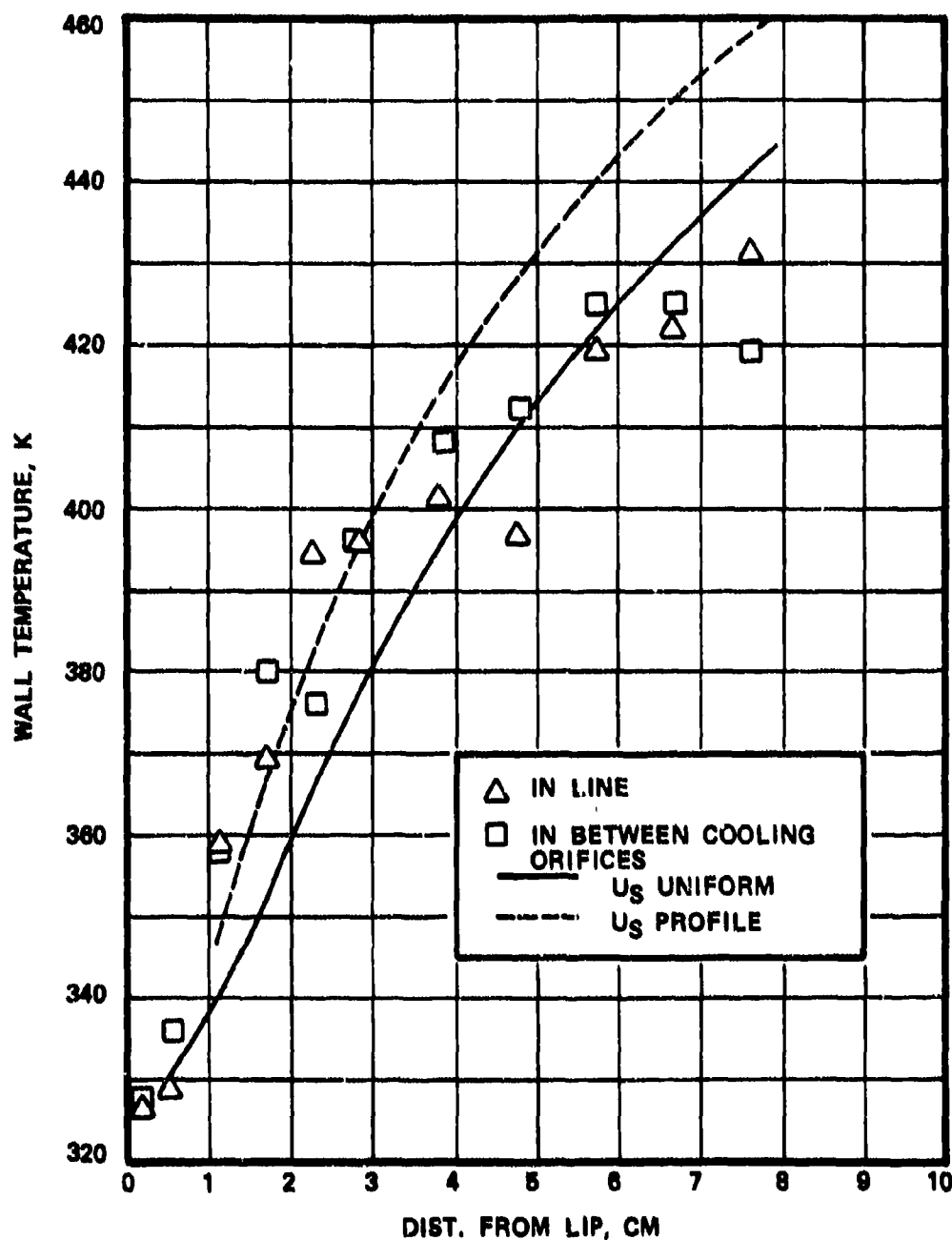
Figure 77. A Comparison Between Predicted and Measured Liner Wall Temperatures for Set-1 of Table 2.
