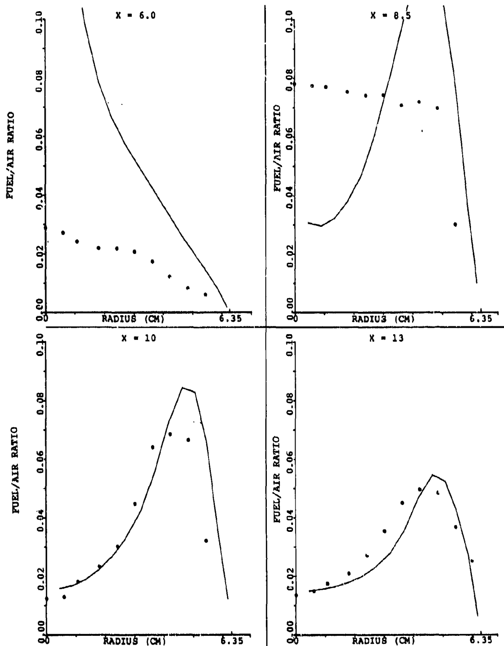
Figure 117. Comparison Between Predicted and Measured Profiles of Fuel/Air Ratio Along \theta = 0^\circ for Set-2, Table 15 (Sheet 1 of 2).
