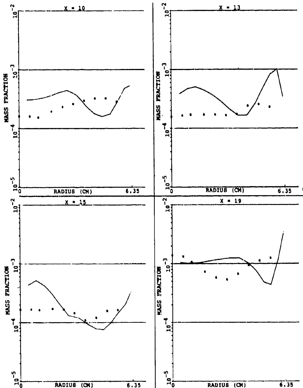
Figure 132. Comparison Between Predicted and Measured CO Profiles for the X-Y Planes In Between the Primary Jet for Set-8 of Table 16 (Sheet 1 of 2).
