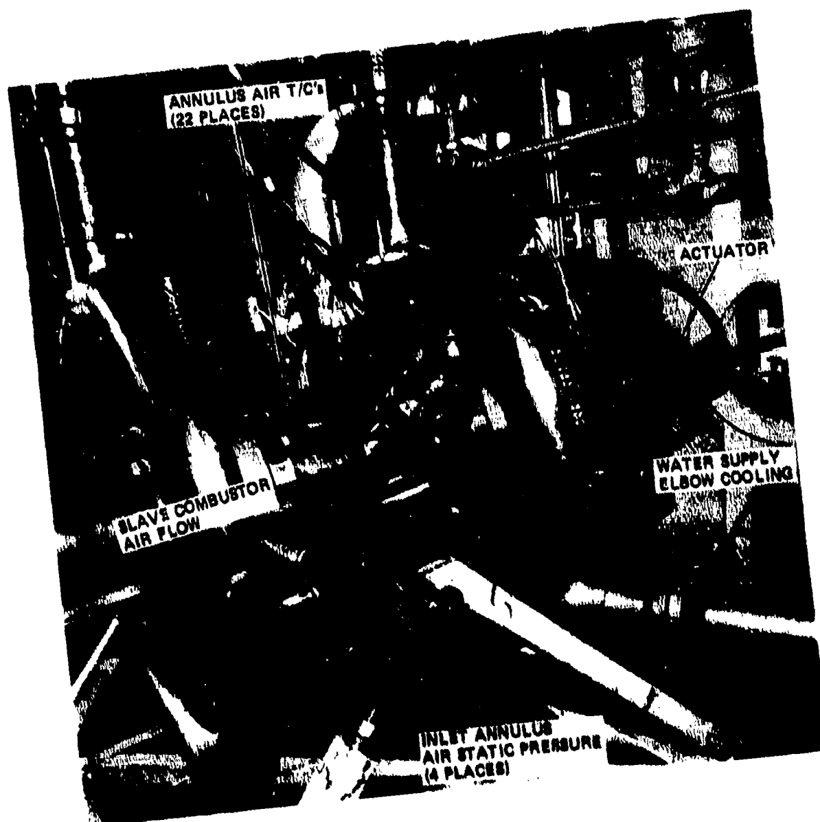
Figure 12. Liner Cooling/Impinging Jet Test Section.
