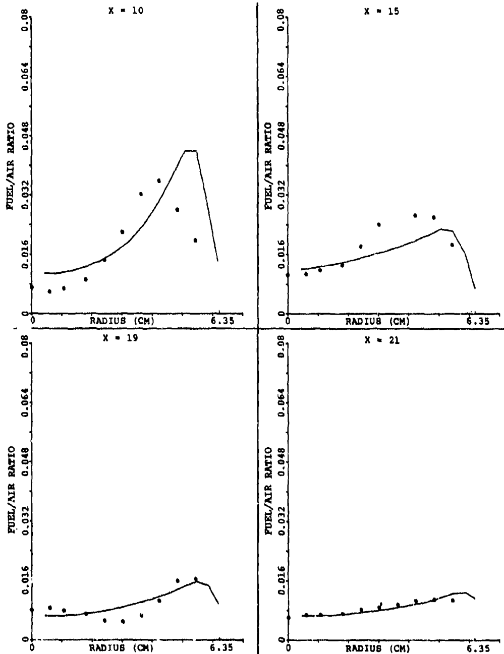
Figure 135. Comparison Between Predicted and Measured Profiles of Fuel/Air Ratio for the X-Y Planes In Between the Primary Jet for Set-3 of Table 15.
