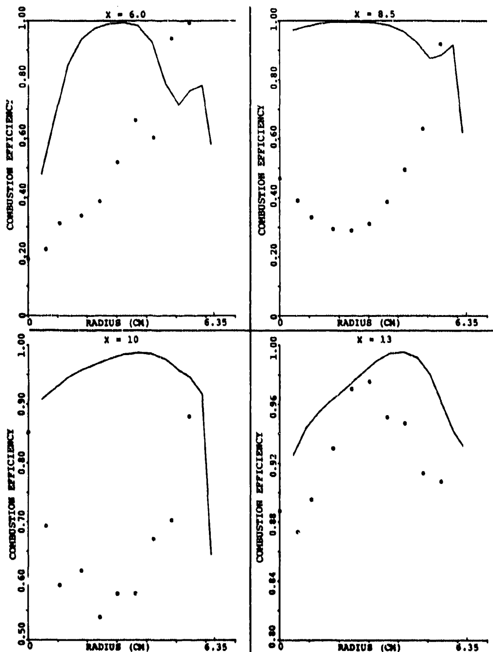
Figure 142. Comparison Between Predicted and Measured Combustion Efficiency for the X-Y Planes In Between the Primary Jet for Set-5 of Table 15 (Sheet 1 of 2).
