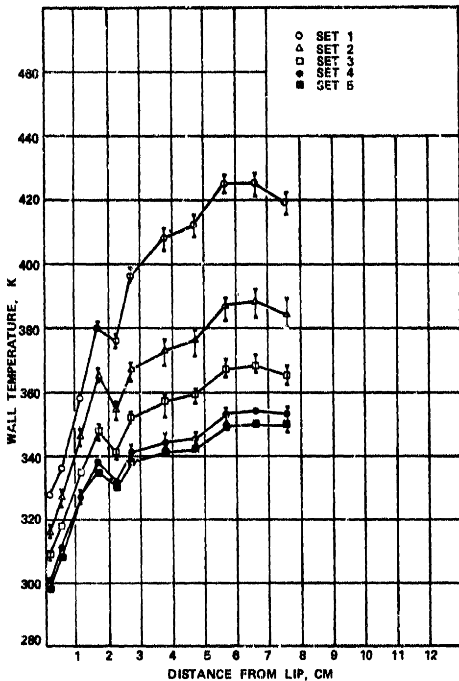
Figure 15. Measured Wall Temperatures of Conventional Film In Between Cooling Orifices.
