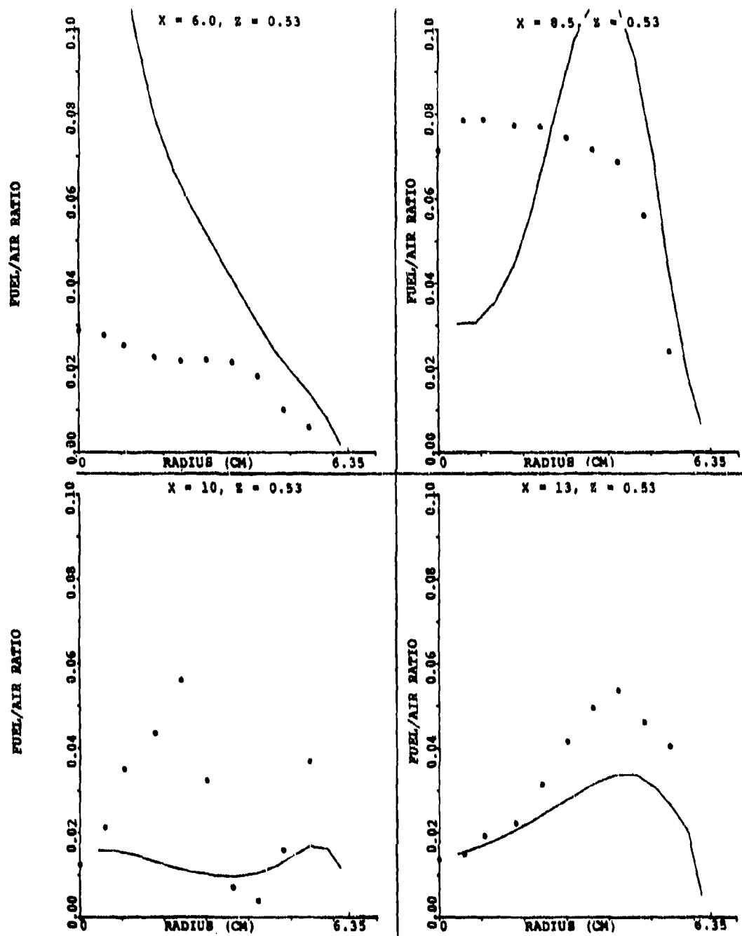
Figure 119. Comparison Between Predicted and Measured Profiles of Fuel/Air Ratio Along \theta = 30^\circ for Set-2, Table 15 (Sheet 1 of 2).
