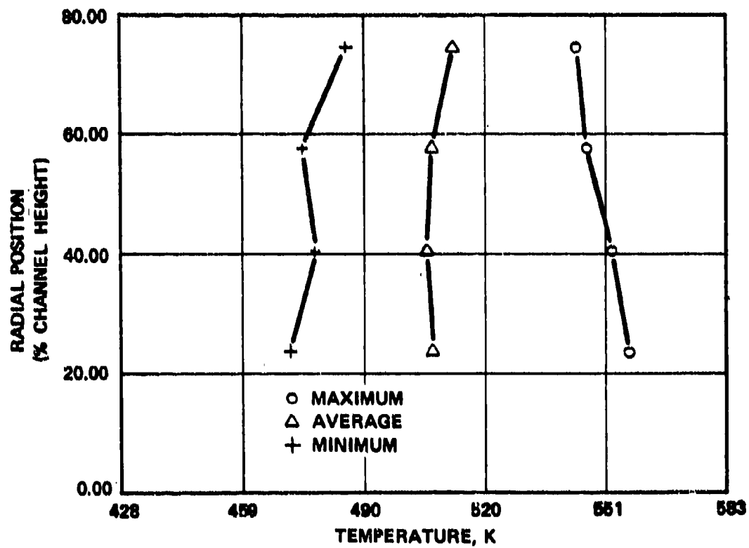
Figure 73. Transition Mixing Tests, Scan-1.
