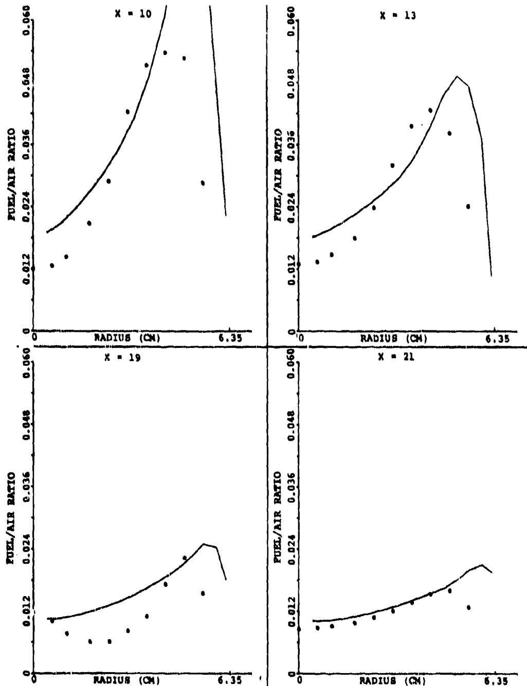
Figure 149. Comparison Between Predicted and Measured Profiles of Fuel/Air Ratio for the X-Y Planes In Between the Primary Jet for Set-11 of Table 16.
