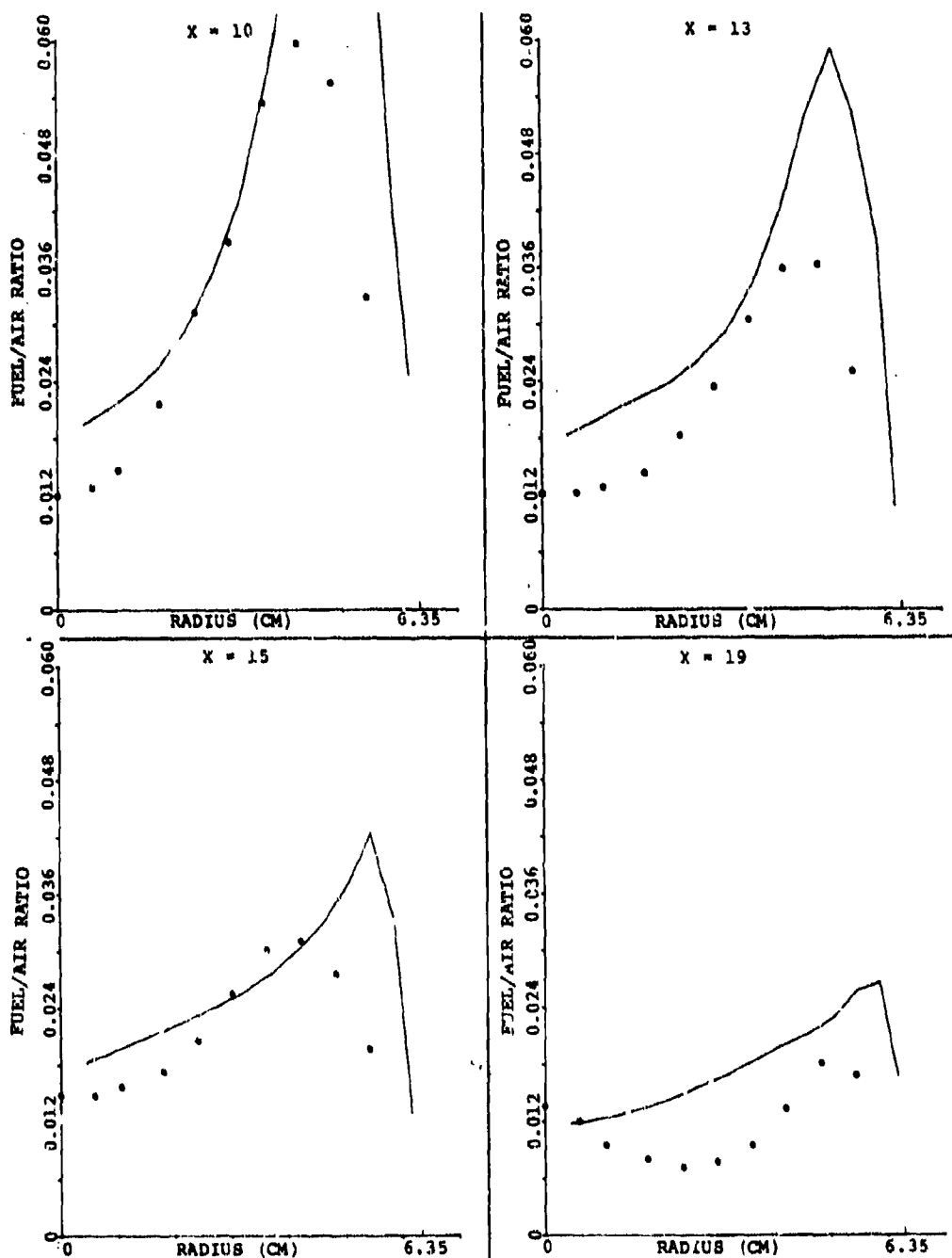
Figure 145. Comparison Between Predicted and Measured Profiles of Fuel/Air Ratio for the X-Y Planes In Between the Primary Jet for Set-9 of Table 16 (Sheet 1 of 2).
