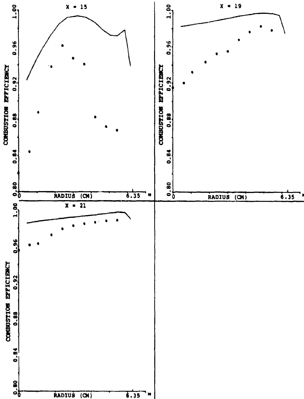
Figure 138. Comparison Between Predicted and Measured Combustion Efficiency for the X-Y Planes In Between the Primary Jet for Set-4 of Table 15.
