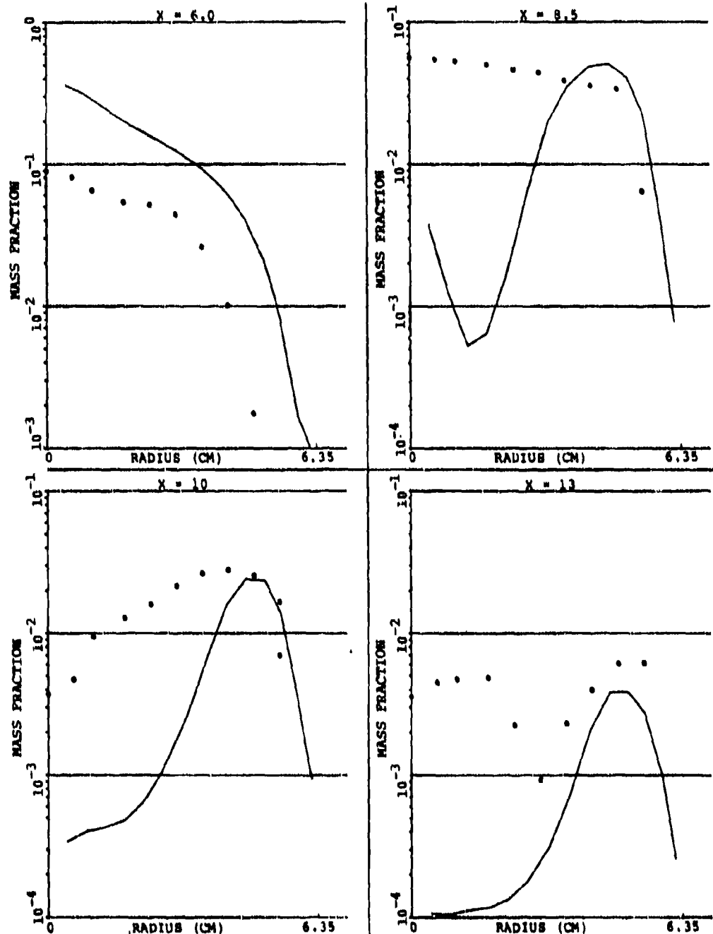
Figure 110. Comparison Between Predicted and Measured Unburned Fuel at Different X-Y Planes ( \theta = 15^\circ ) In Between Primary Jets ( \theta = 30^\circ ) for Set-2, Table 15. (Sheet 1 of 2)
