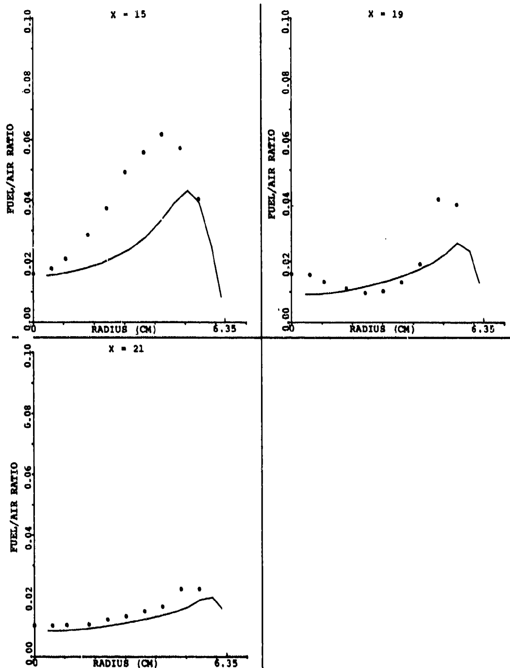
Figure 137. Comparison Between Predicted and Measured Profiles of Fuel/Air Ratio for the X-Y Planes In Between the Primary Jet for Set-4 of Table 15.
