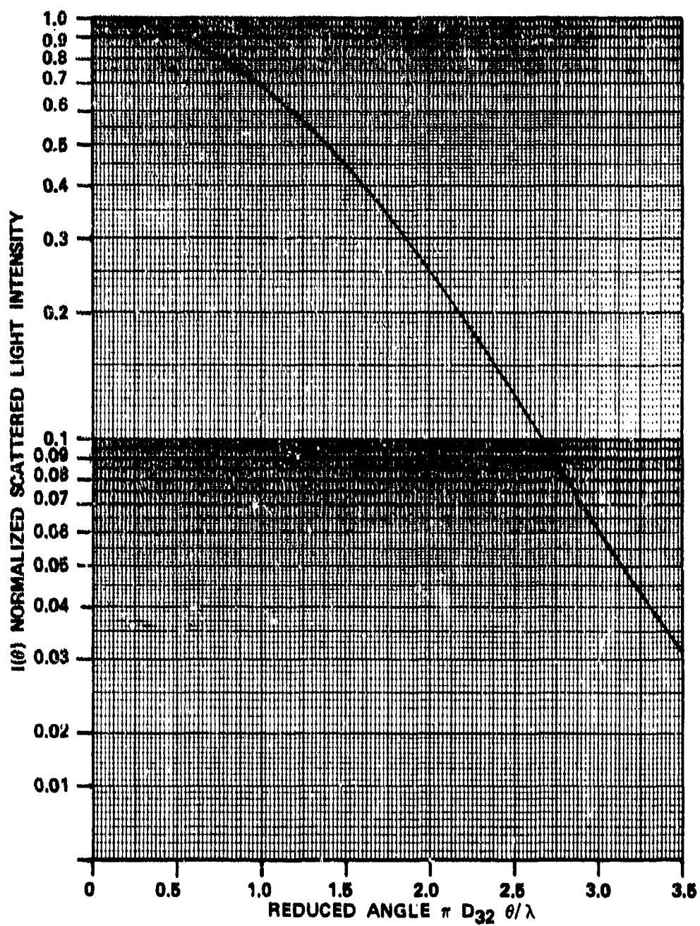
Figure 64. Mean Theoretical Illumination Profile.
