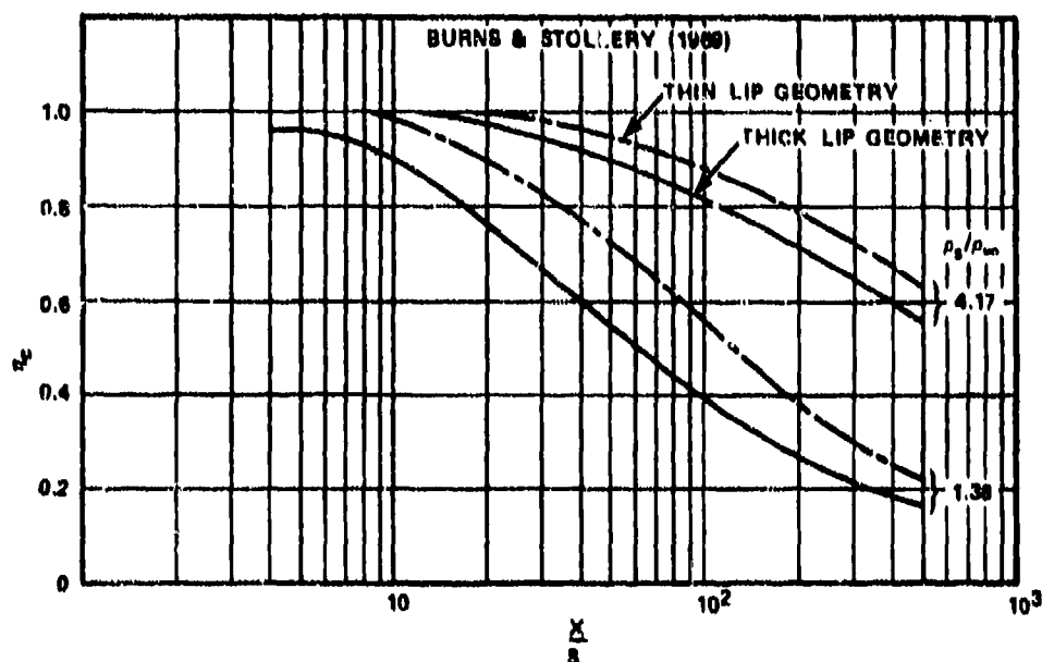
Figure 8. Effect of Density Ratio, \rho_g/\rho_\infty , Lip Geometry and Main Stream Boundary Layer Thickness on Impermeable Wall Effectiveness, \eta_c , as Reported by Burns and Stollery 15 .
