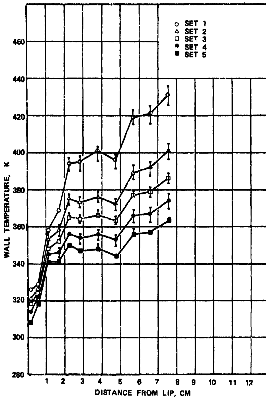
Figure 14. Measured Wall Temperatures of Conventional Film In Line With Orifice.
