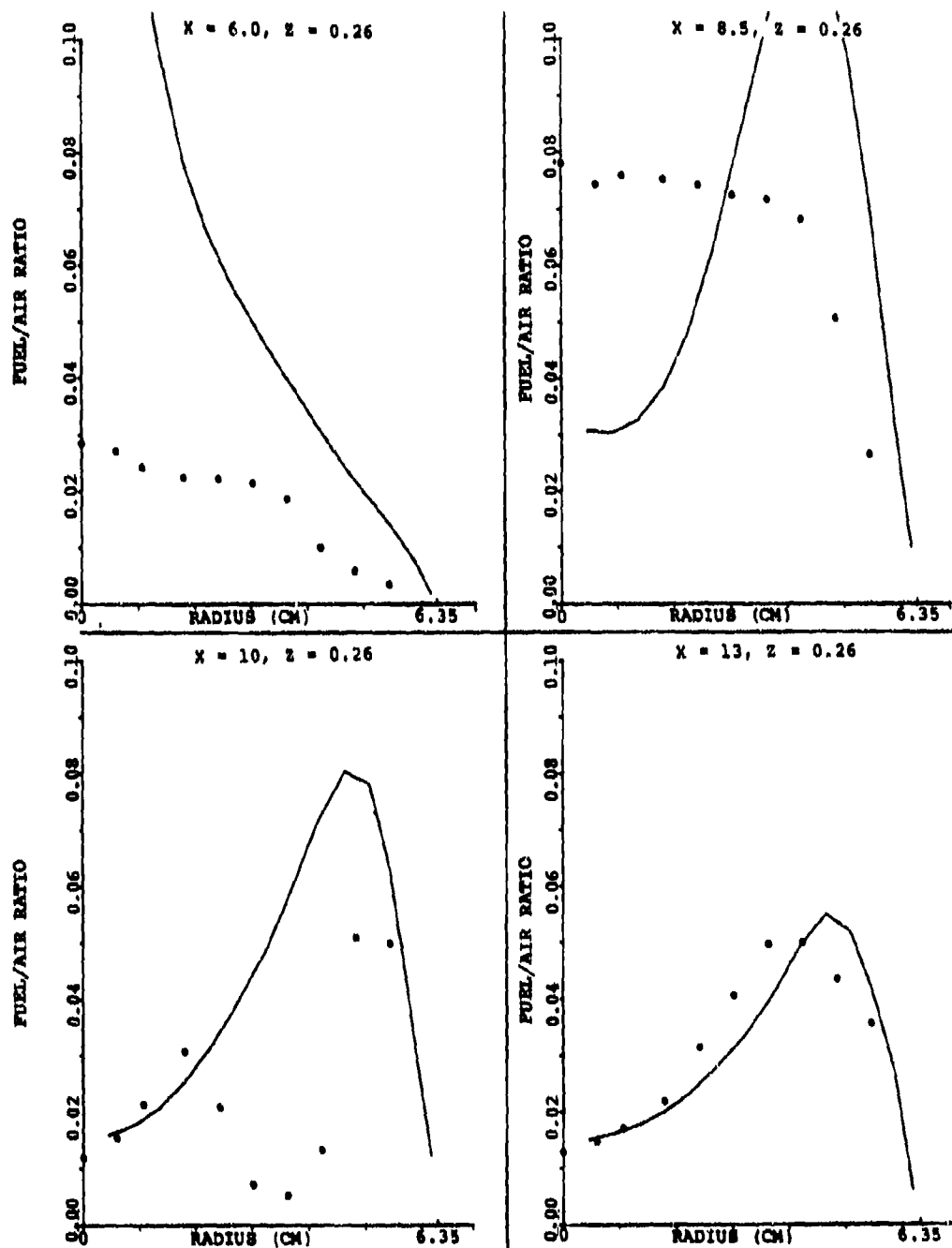
Figure 118. Comparison Between Predicted and Measured Profiles of Fuel/Air Ratio Along \theta = 15^\circ for Set-2, Table 15 (Sheet 1 of 2).
