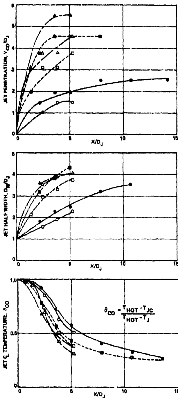
Figure 41. Measured Mixing Characteristics of the In-line Six-Opposing Jets.
