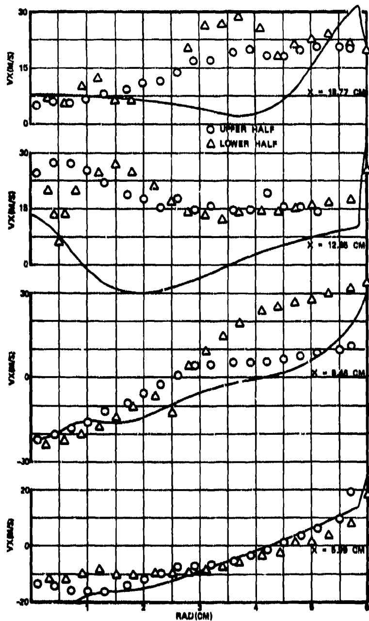
Figure 104. Comparison Between Predicted and Measured Axial Velocity Profiles in Different X-Y Planes in Between Primary Jet; Combustor Air-flow Rate = 2.26 kg/s. (Sheet 1 of 2)
