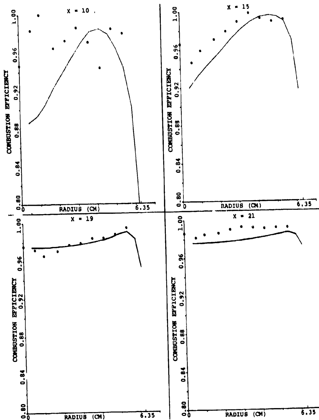
Figure 136. Comparison Between Predicted and Measured Combustion Efficiency for the X-Y Planes In Between the Primary Jet for Set-3 of Table 15.
