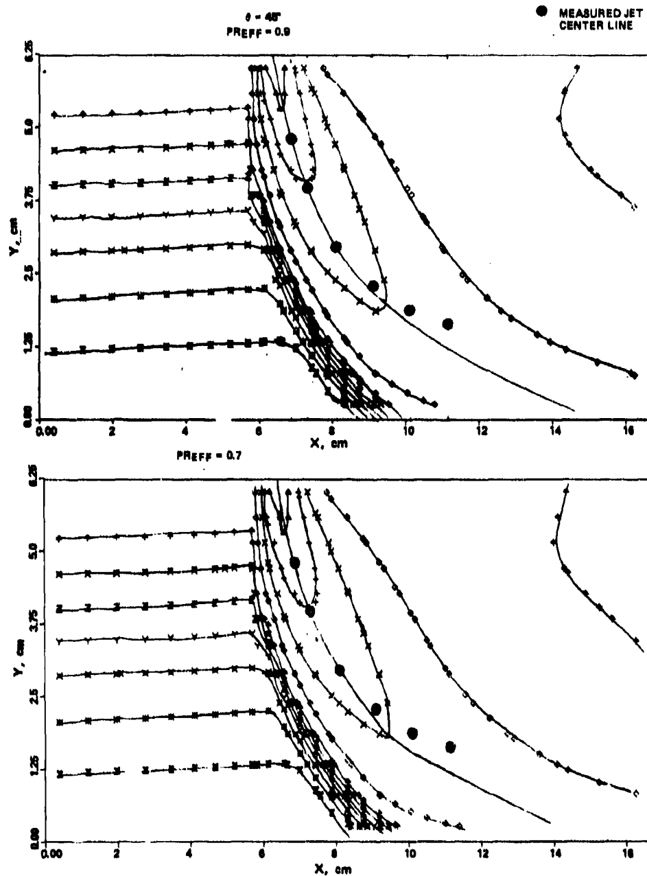
Figure 85. Effect of Prandtl Number on Predicted Isothermal Plots of Set-3 of Table 10.
