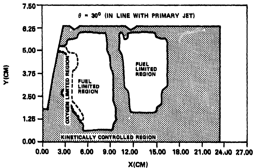
Figure 124. Predicted Regions Controlled by Availability of Oxygen and Fuel, and Chemical Kinetics for Set-1 of Table 15.
