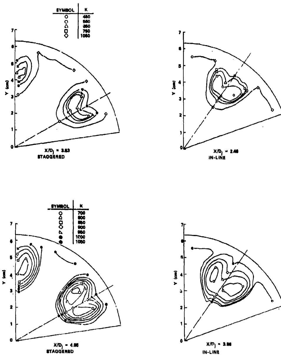
Figure 35. A Typical Comparison Between Mixing Characteristics of In-Line and Staggered Rows of Dilution Jets Upstream of the Second Row (Sheet 2 of 3).
