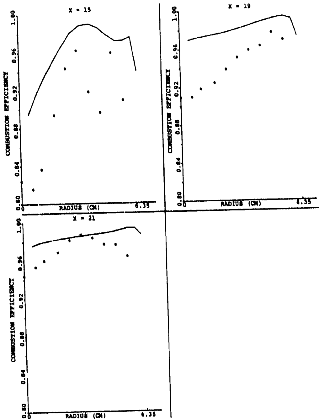
Figure 120. Comparison Between Predicted and Measured Combustion Efficiency Along \theta = 0^\circ for Set-2, Table 15 (Sheet 2 of 2).
