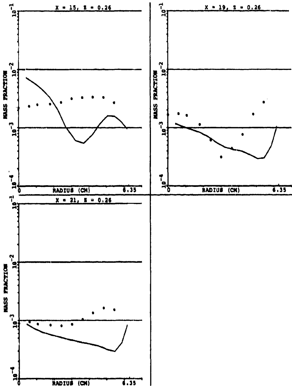
Figure 115. Comparison Between Predicted and Measured CO at Different X-Y Planes ( \theta = 15^\circ ) for Set-2, Table 15 (Sheet 2 of 2).
