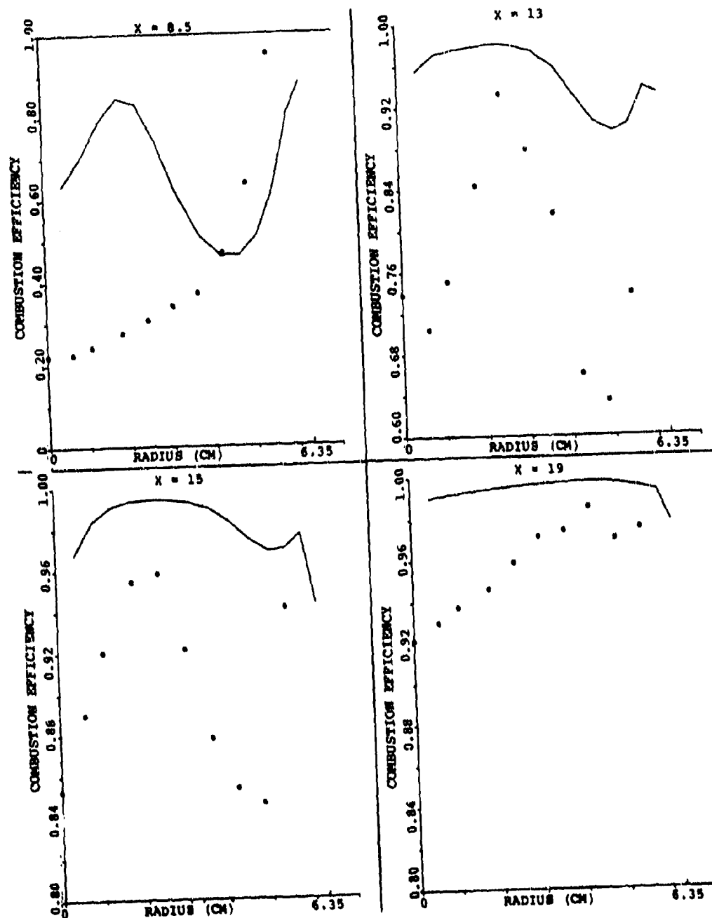
Figure 140. Comparison Between Predicted and Measured Combustion Efficiency for the X-Y Planes In Between the Primary Jet for Set-6 of Table 15.
