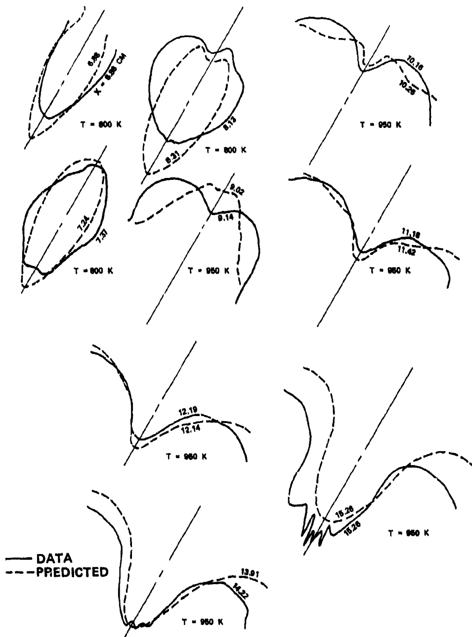
Figure 95. Comparison Between Predicted and Measured Isothermal Lines of a Six-Opposing Jet, J = 41.1 , Set-4 of Table 11.
