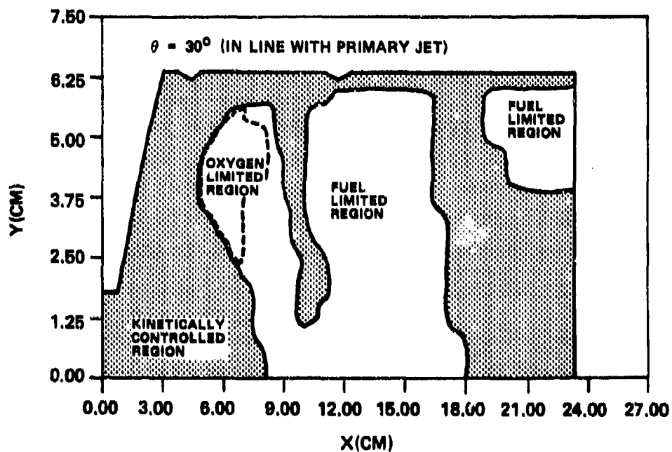
Figure 123. Predicted Regions Controlled by Availability of Oxygen and Fuel and Chemical Kinetics for Set-2 of Table 15.
