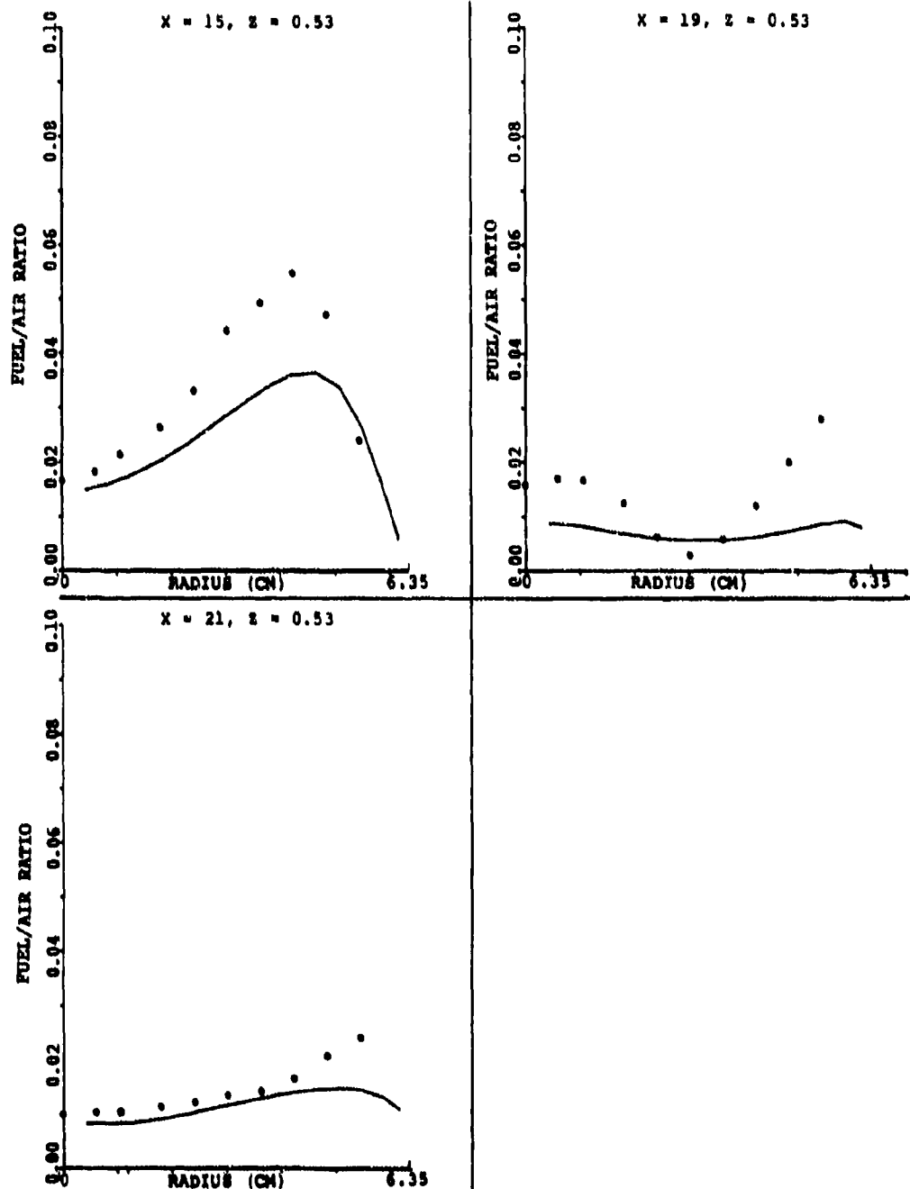
Figure 119. Comparison Between Predicted and Measured Profiles of Fuel/Air Ratio Along \theta = 30^\circ for Set-2, Table 15 (Sheet 2 of 2).
