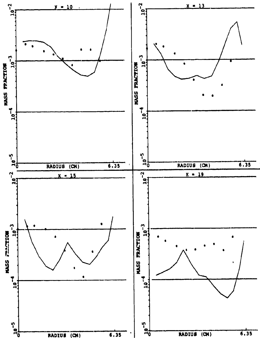
Figure 131. Comparison Between Measured and Predicted Unburned Fuel for the X-Y Planes In Between the Primary Jet for Set-8 of Table 16 (Sheet 1 of 2).
