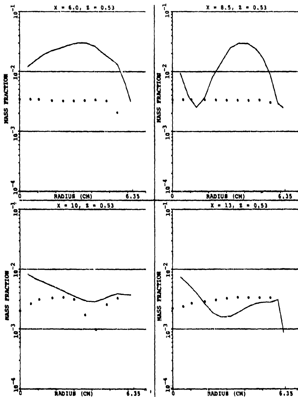
Figure 116. Comparison Between Predicted and Measured CO at Different X-Y Planes ( \theta = 30^\circ ) for Set-2, Table 15 (Sheet 1 of 2).
