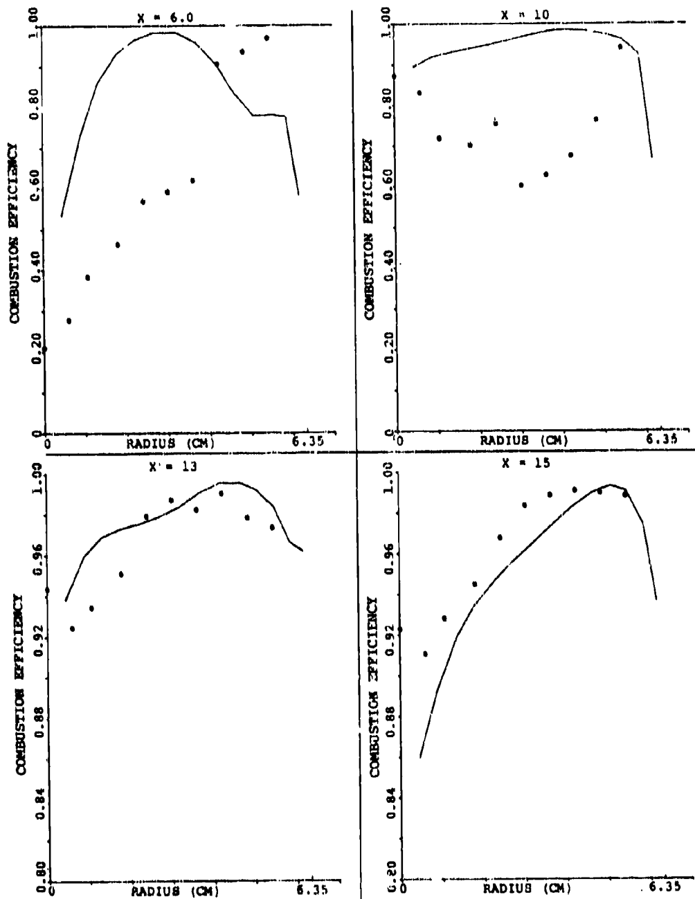
Figure 134. Comparison Between Predicted and Measured Combustion Efficiency for the X-Y Planes In Between the Primary Jet for Set-1 of Table 15 (Sheet 1 of 2).
