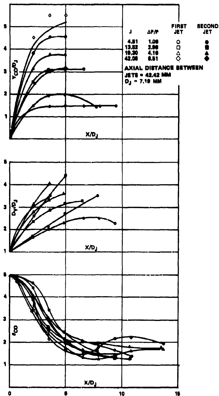
Figure 42. Measured Mixing Characteristics of the Staggered Six-Opposing Jets.
