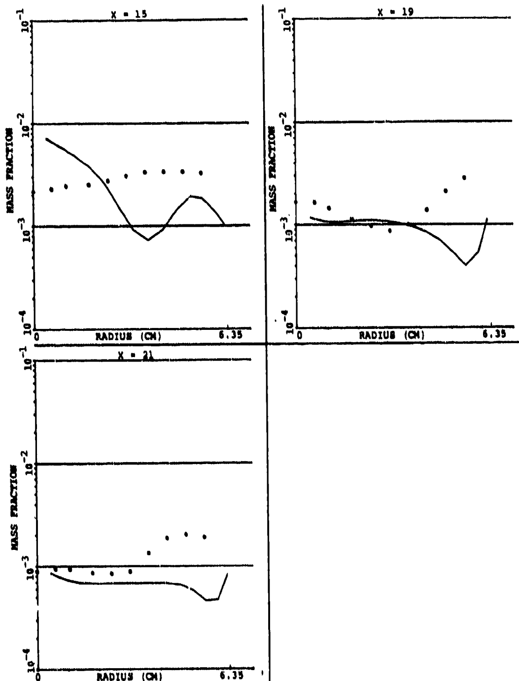
Figure 114. Comparison Between Predicted and Measured Profiles of CO at Different X-Y Planes ( \theta = 0^\circ ) In Between the Primary Jet ( \theta = 30^\circ ) for Set-2, Table 15 (Sheet 2 of 2)
