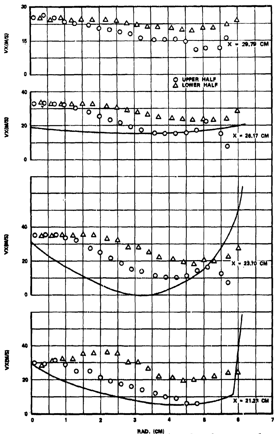
Figure 105. Comparison Between Predicted and Measured Axial Velocity Profiles in Different X-Y Planes In Line With Primary Jet; Combustor Airflow Rate = 2.74 kg/s. (Sheet 2 of 2)
