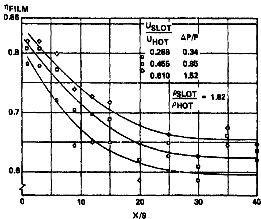
Figure 23. Film Effectiveness of Impingement/Film Cooling Scheme with Density Ratio as Parameter.
