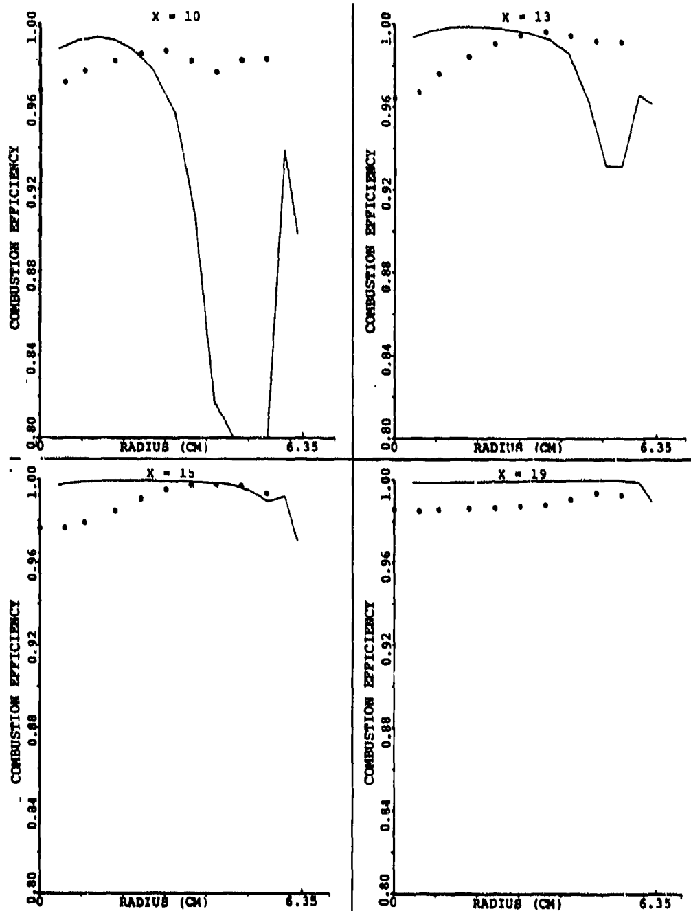
Figure 146. Comparison Between Predicted and Measured Combustion Efficiency for the X-Y Planes In Between the Primary Jet for Set-9 of Table 16 (Sheet 1 of 2).
