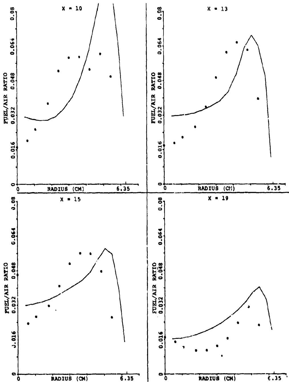
Figure 153. Comparison Between Predicted and Measured Profiles of Fuel/Air Ratio for the X-Y Planes In Between the Primary Jet for Set-13 of Table 16 (Sheet 1 of 2).
