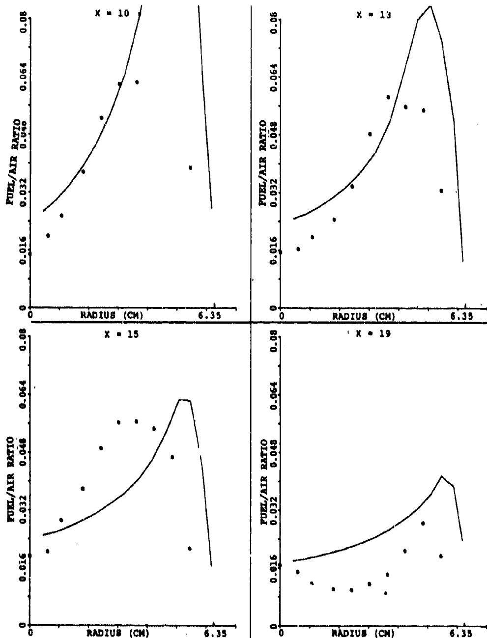
Figure 151. Comparison Between Predicted and Measured Profiles of Fuel/Air Ratio for the X-Y Planes In Between the Primary Jet for Set-12 of Table 16 (Sheet 1 of 2).
