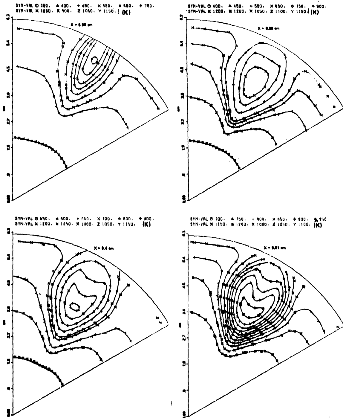
Figure 98. Predicted Mixing Characteristics of a First-Row Jet of Two In-Line Rows of Six-Opposing Jets Configuration; Location of First Row x = 6.35 cm.
