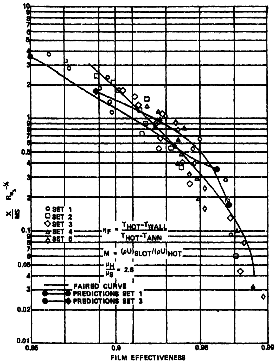
Figure 18. Film Effectiveness of Conventional Film Cooling Scheme.
