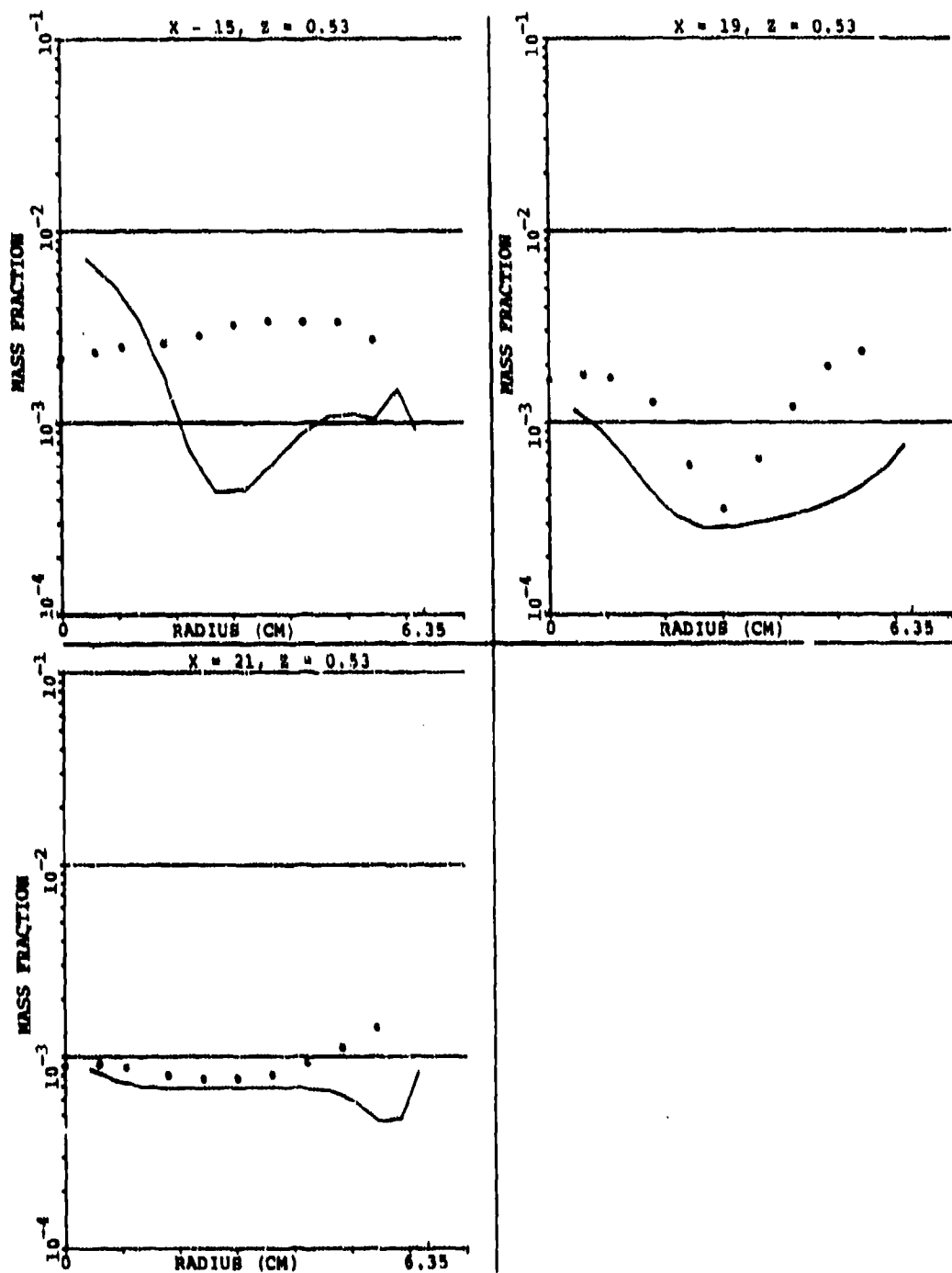
Figure 116. Comparison Between Predicted and Measured CO at Different X-Y Planes ( \theta = 30^\circ ) In Line With the Primary Jet ( \theta = 30^\circ ) for Set-5, Table 15 (Sheet 2 of 2).
