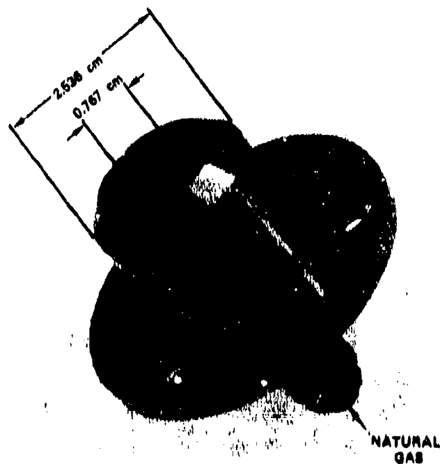
Figure 54. Natural Gas Nozzle and Airblast Nozzle Used for the Can Combustor Mapping.
