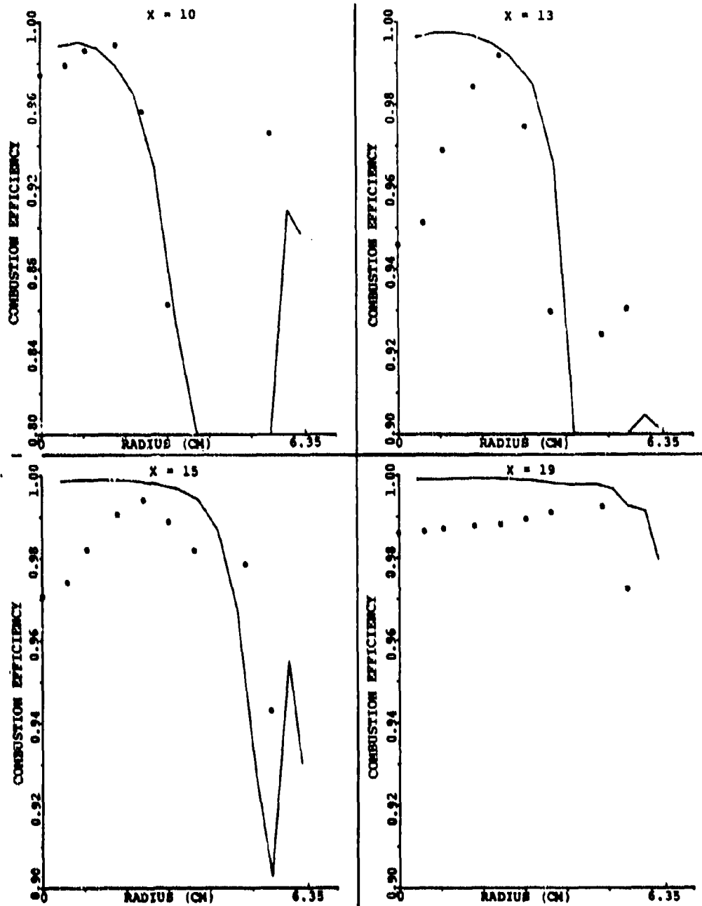
Figure 148. Comparison Between Predicted and Measured Combustion Efficiency for the X-Y Planes In Between the Primary Jet for Set-10 of Table 16 (Sheet 1 of 2).
