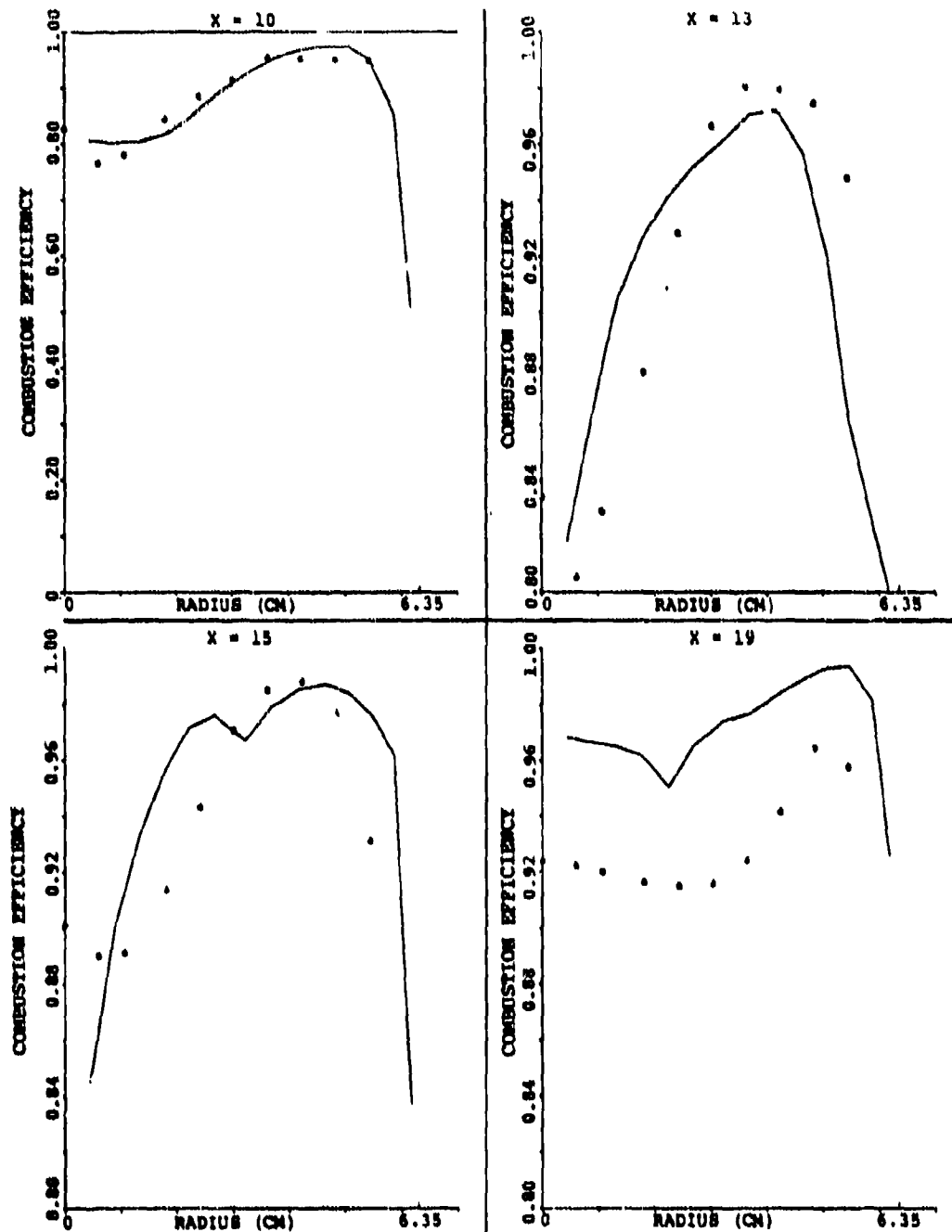
Figure 128. Combustion Efficiency Profiles for the X-Y Planes ( \theta = 0^\circ ) In Between the Primary Jet for Set-8 of Table 16 (Sheet 1 of 2).
