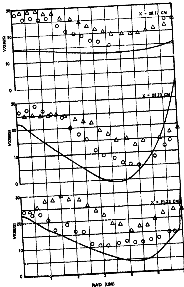
Figure 104. Comparison Between Predicted and Measured Axial Velocity Profiles in Different X-Y Planes In Between Primary Jet; Combustor Air-flow Rate = 2.26 kg/s. (Sheet 2 of 2)
