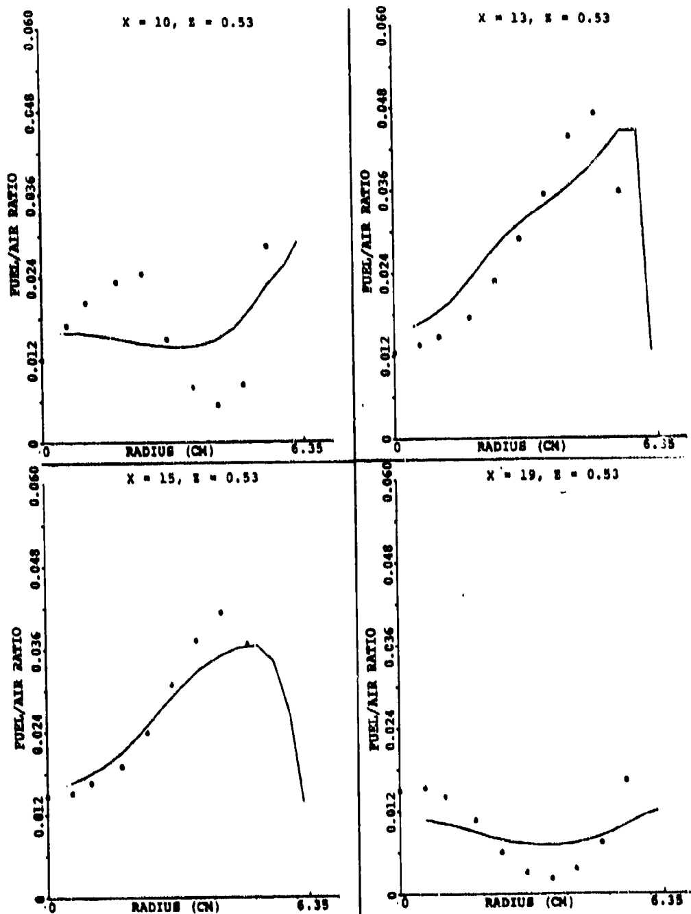
Figure 127. Comparison Between Predicted and Measured Profiles of Fuel/Air Ratio for the X-Y Planes in Line With the Primary Jet for Set-8 of Table 15 (Sheet 1 of 2).
