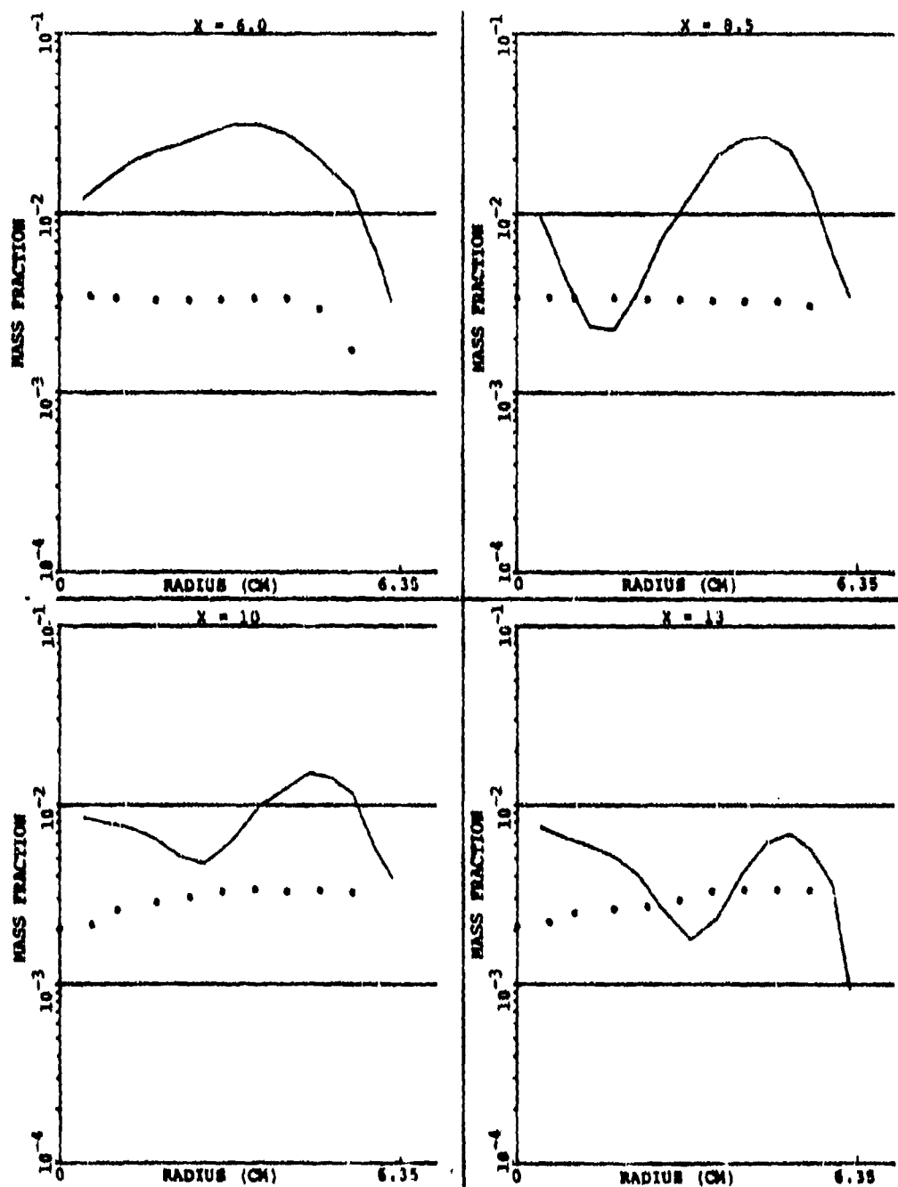
Figure 114. Comparison Between Predicted and Measured Profiles of CO at Different X-Y planes ( \theta = 0^\circ ) In Between the Primary Jet ( \theta = 30^\circ ) for Set-2, Table 15 (Sheet 1 of 2).
