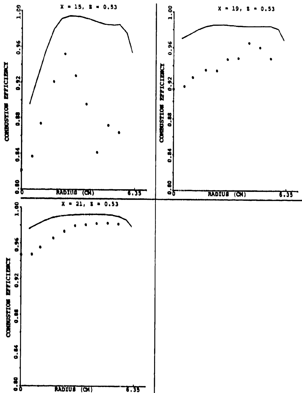
Figure 122. Comparison Between Predicted and Measured Combustion Efficiency Along \theta = 30^\circ for Set-2, Table 15 (Sheet 2 of 2).
