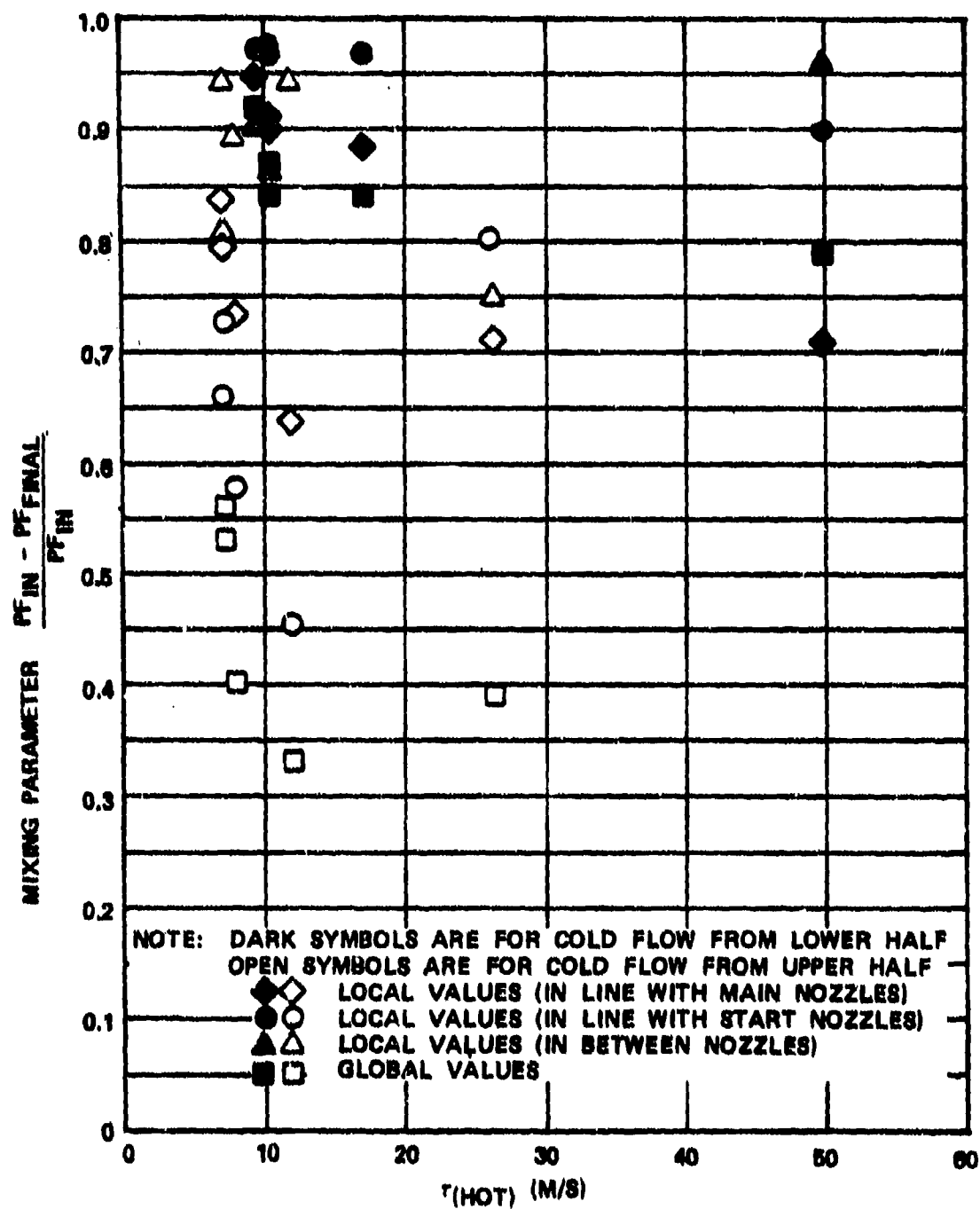
Figure 75. Mixing Parameter Versus T(Hot) .
