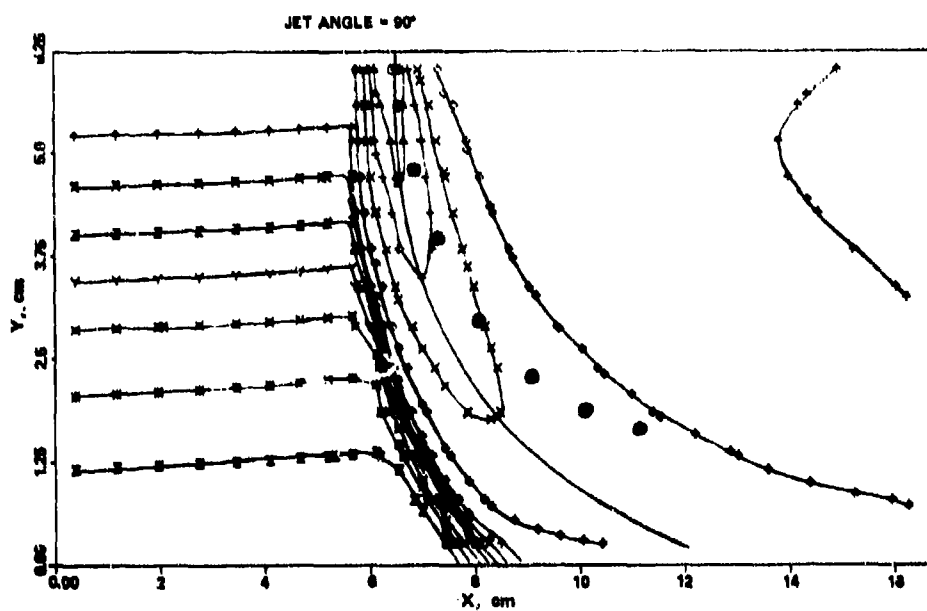
Figure 84. Effect of Jet Angle on Predicted Isothermal Lines of Set-3 of Table 10.
