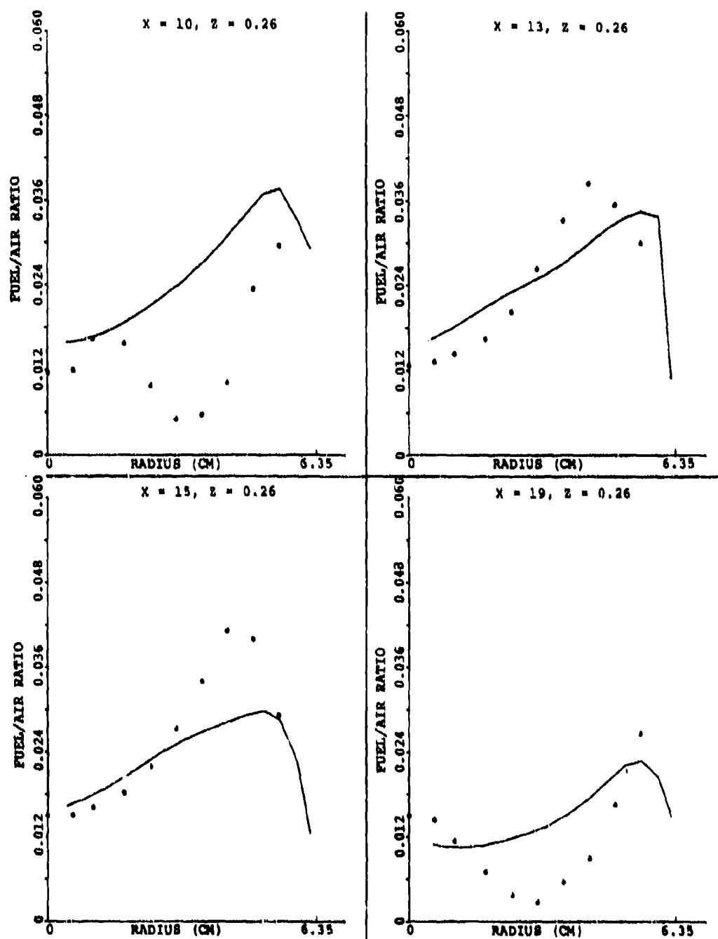
Figure 126. Comparison Between Predicted and Measured Profiles of Fuel/Air Ratio for the \theta = 15^\circ Plane for Set-8 of Table 16 (Sheet 1 of 2).
