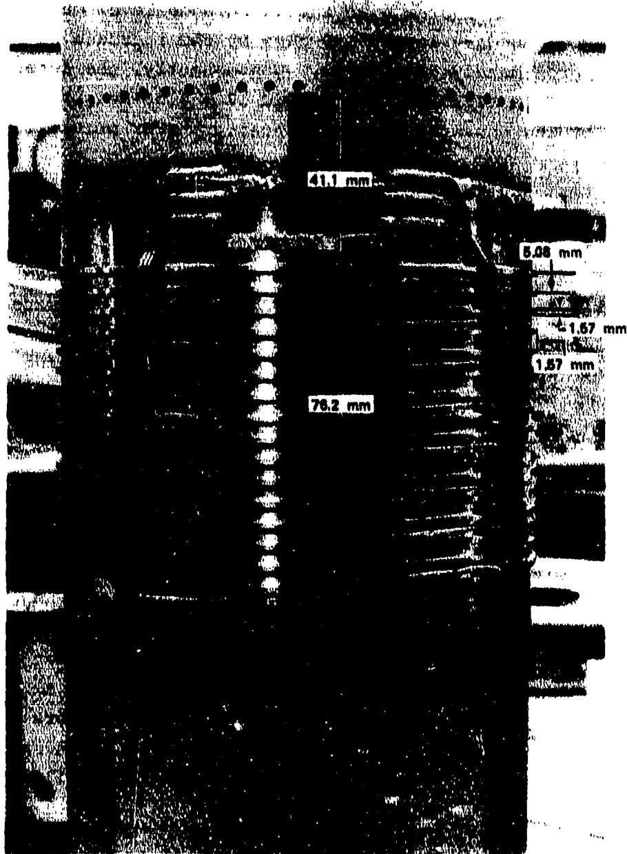
Figure 25. Film/Extended Surface Convection Cooling Scheme.
