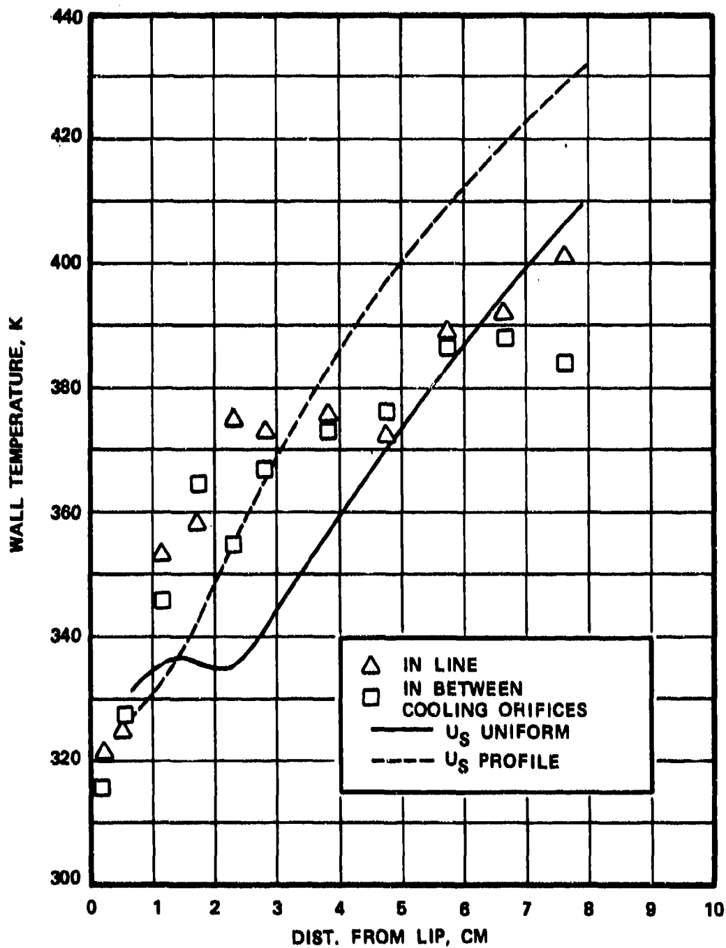
Figure 78. A Comparison Between Predicted and Measured Liner Wall Temperatures for Set-2 of Table 2.
