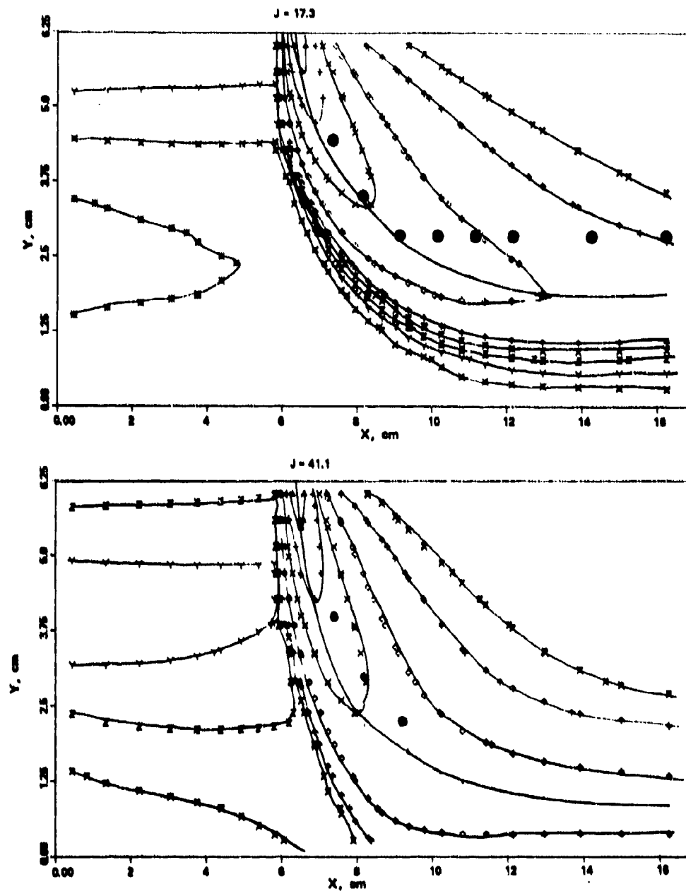
Figure 91. Comparison Between Predicted and Measured Jet Trajectories of Six-Opposing Jets With Jet Momentum Ratio As a Parameter. (Sheet 2 of 3)
