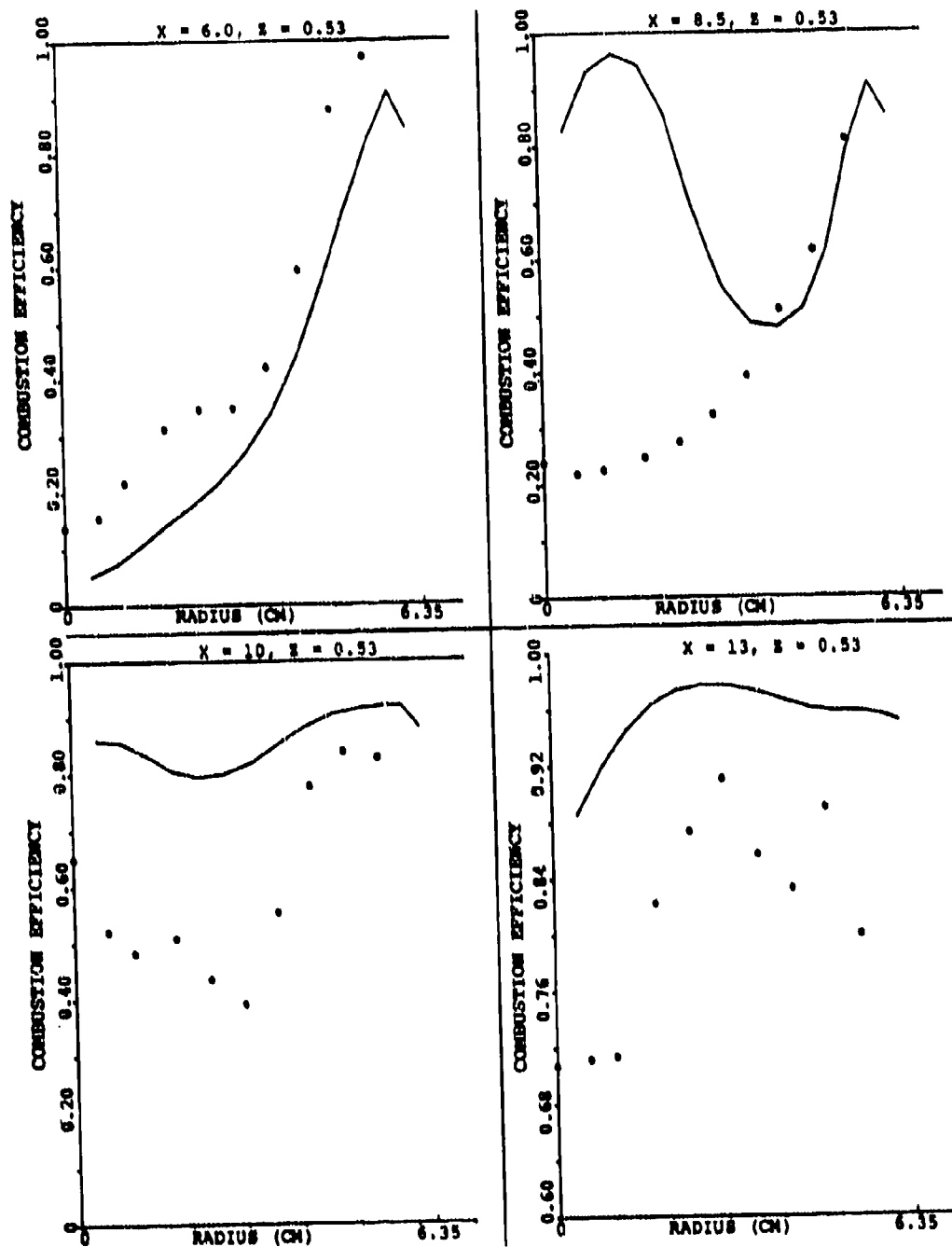
Figure 122. Comparison Between Predicted and Measured Combustion Efficiency Along \theta = 30^\circ for Set-2, Table 15 (Sheet 1 of 2).
