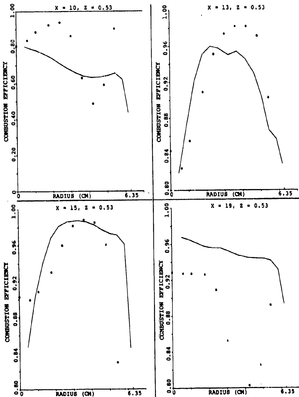
Figure 130. Combustion Efficiency Profiles for the X-Y Planes In Line With the Primary Jet for Set-8 of Table 16 (Sheet 1 of 2).
