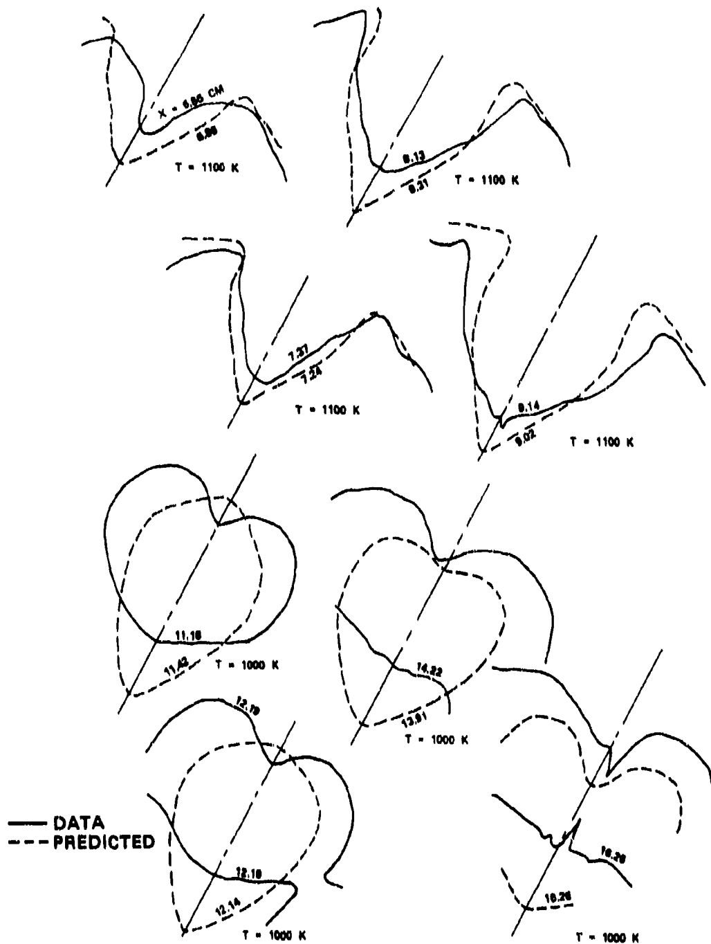
Figure 94. Comparison Between Predicted and Measured Isothermal Lines of a Six-Opposing Jet, J = 17.3 , Set-3 of Table 11.
