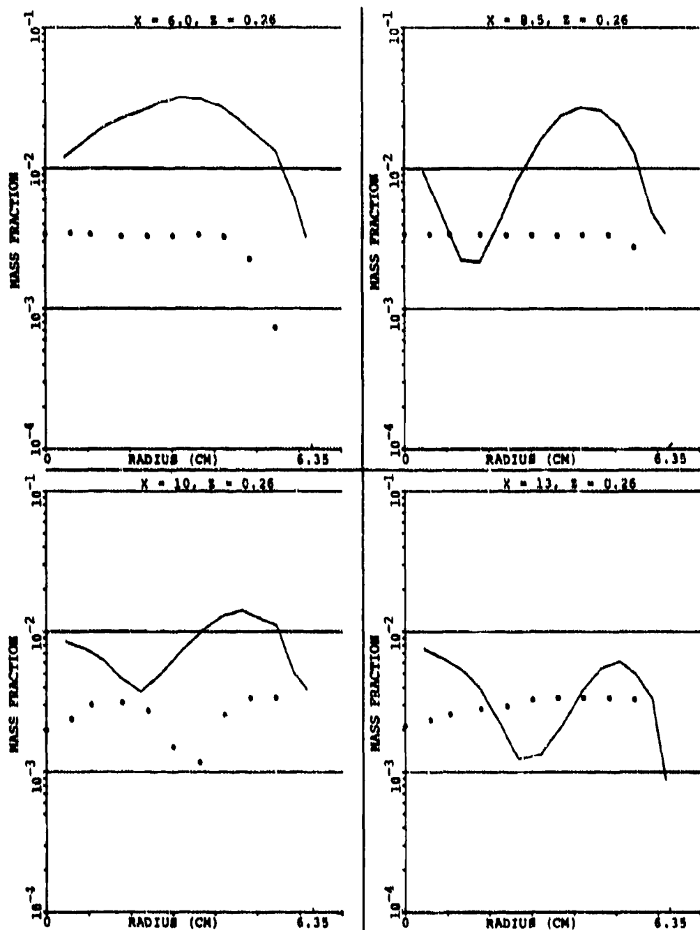
Figure 115. Comparison Between Predicted and Measured CO at Different X-Y Planes ( \theta = 15^\circ ) for Set-2, Table 15 (Sheet 1 of 2).
