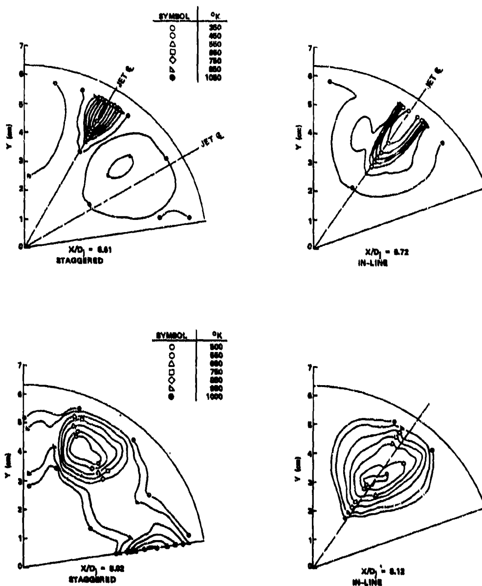
Figure 36. A Typical Comparison Between Mixing Characteristics of In-Line and Staggered Rows of Dilution Jets the Region Downstream of the Second Row (Sheet 1 of 2).
