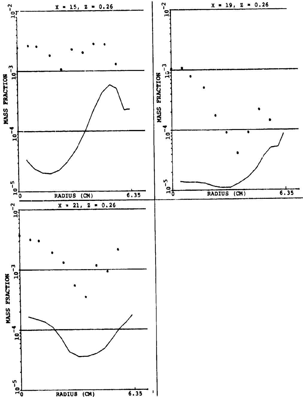
Figure 111. Comparison Between Predicted and Measured Unburned Fuel At Different X-Y Planes ( \theta = 15^\circ ) (As Compared to the Primary Jet Located at \theta = 30^\circ ) for Set-2, Table 15. (Sheet 2 of 2)
