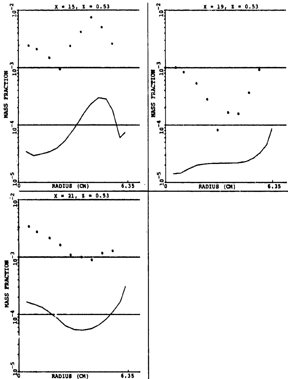
Figure 112. Comparison Between Predicted and Measured Unburned Fuel at Different X-Y Planes in Line With the Primary Jet ( \theta = 30^\circ ) for Set-2, Table 15 (Sheet 2 of 2).
