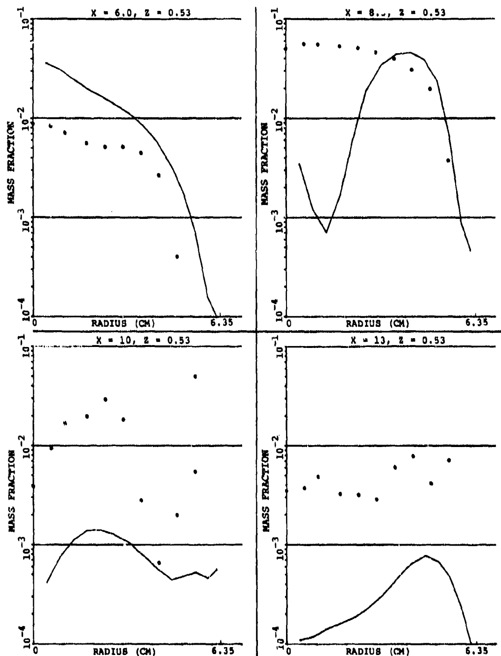
Figure 112. Comparison Between Predicted and Measured Unburned Fuel at Different X-Y Planes In Line With the Primary Jet ( \theta = 30^\circ ) for Set-2, Table 15 (Sheet 1 of 2).
