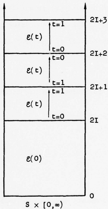
Figure 3.4.1. The family \{\mathcal{E}'(t')\}_{t' \in [0, \infty)}
