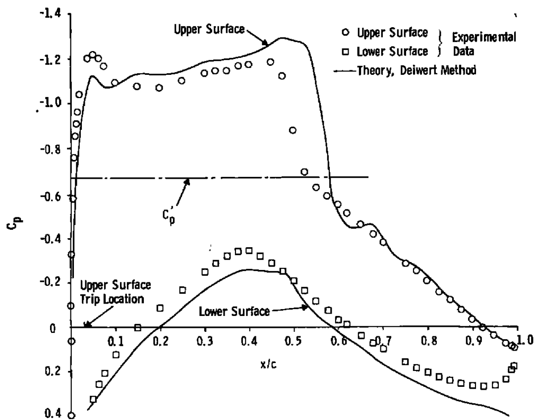
c. M_\infty = 0.73 , Re_{m,c} = 2.7 \times 10^6 , \alpha = 3.19 (case 12) Figure 3. Concluded.
