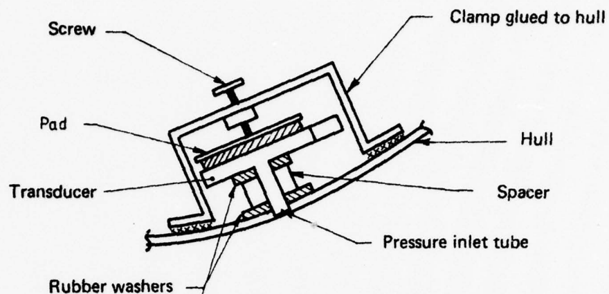
FIG. 4. METHOD OF CLAMPING AND SEALING PRESSURE TRANSDUCER TO HULL.
