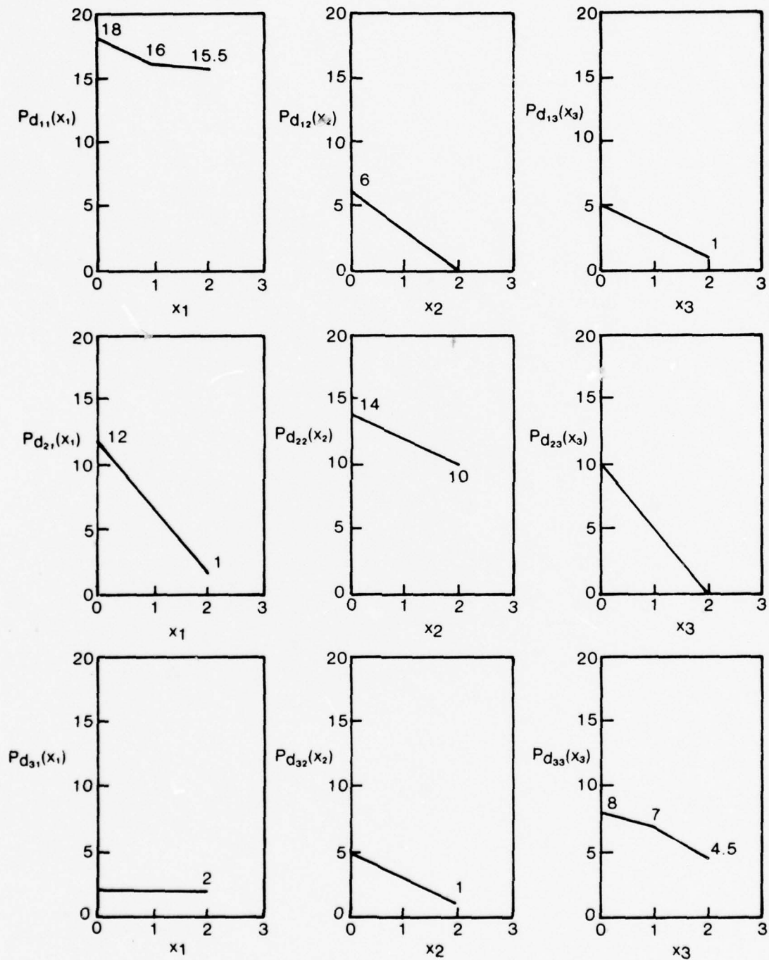
Figure 6. Demand Functions for Piecewise Linear Market
