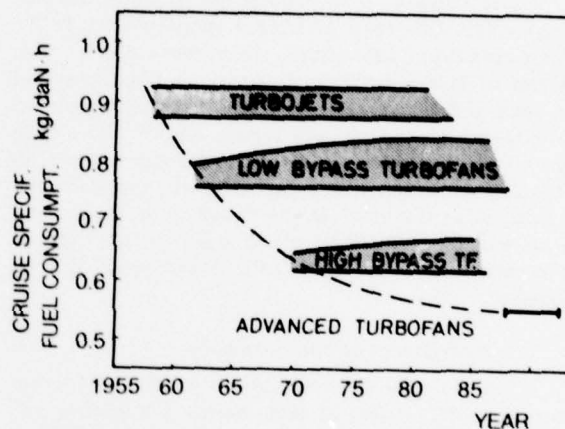
Fig.9 Development of cruise specific fuel consumption of aero gas turbines with time 5
