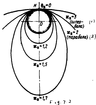
Fig. 7.2. Family of characteristic trajectories of flight at high altitudes.
