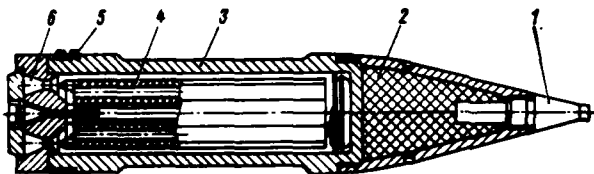
Fig. 0.14. Rocket projectile (ABS): 1 - fuse; 2 - warhead; 3 - rocket camera/chamber; 4 - charge of rocket propellant; 5 - driving bands; 6 - nozzle unit.
