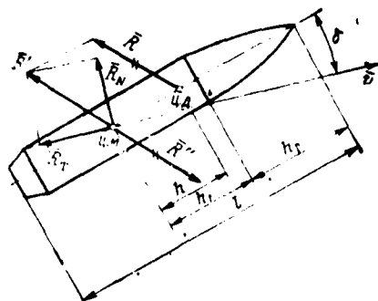
Fig. 2.23. Circuit of bringing the main vector of aerodynamic forces to the center of mass of the rotating projectile.
