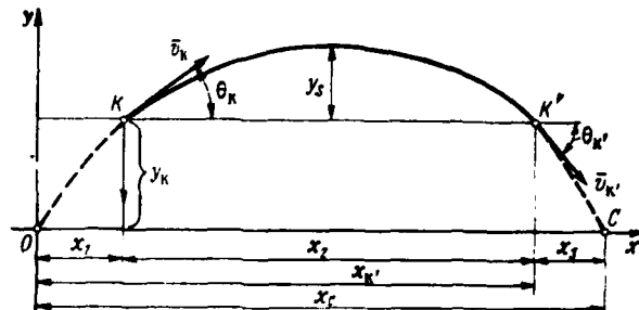
Fig. 7.9. Dividing circuit of trajectory into separate calculated sections.
