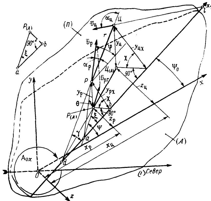
Fig. 4.13. Schematic of the angles, which determine the position of the line of sighting and velocity vector the center of mass of rocket in space and on the plane of interception (B).
