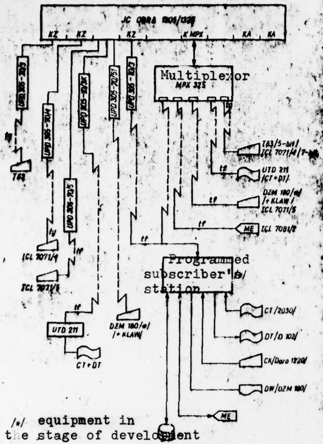
Fig.2 The ODRA 1305(1325) computer. The configuration of teletransformation (in the stage of development)
