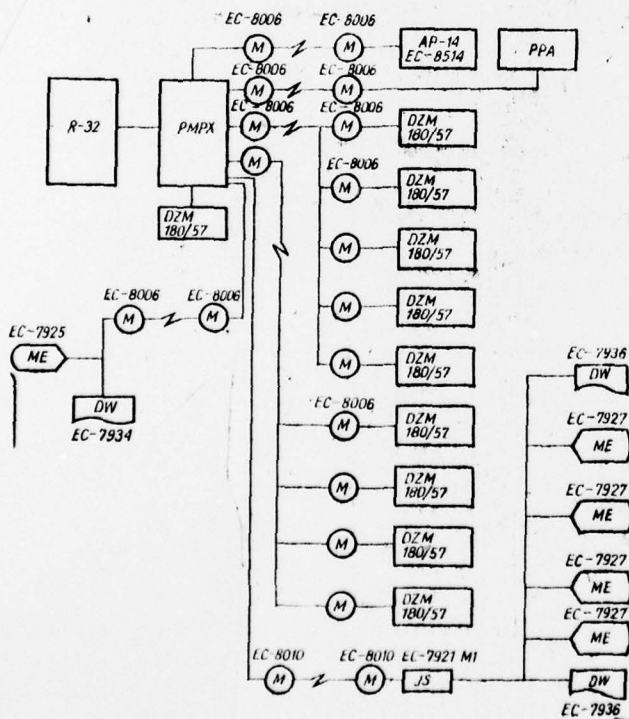
Fig.5 . The R-32 computer's configuration of teletransformation (in the stage of preparation)
