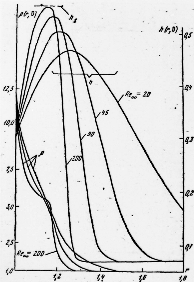
Fig. 5. Profiles of functions \rho and h on the stagnation line \theta=0 ( M_\infty=6 )
