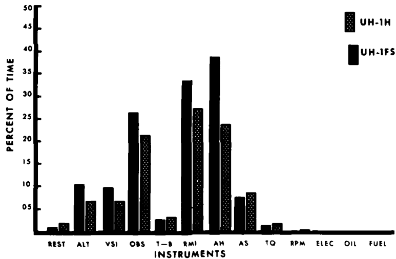
FIGURE 7. SCAN RATE COMPARISONS OF AIRCRAFT DURING ILS MANEUVERS
