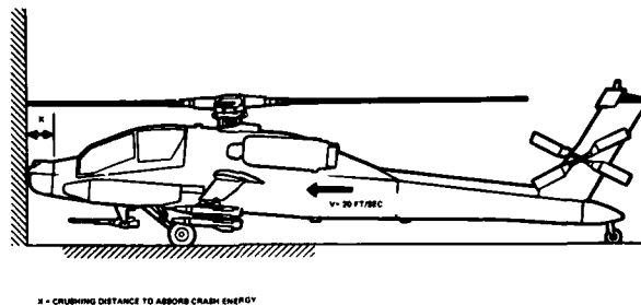
Fig. 2. Longitudinal rigid barrier impact at 20 ft/sec.
