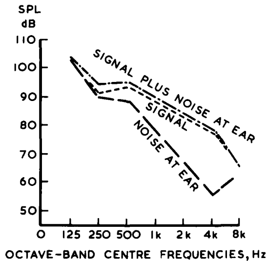
Fig. 6. NOISE AND SIGNAL COMBINED TO GIVE TOTAL EXPOSURE
