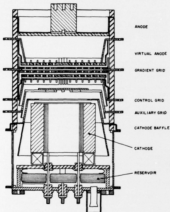
Figure 1. External view of MAPS-40 thyatron.
