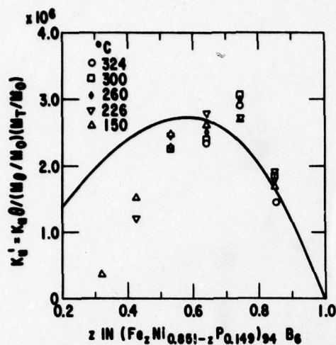
Fig. 4 Maximum induced anisotropy corrected for annealing temperature and magnetization for Fe-Ni-P-B alloys. Composition axis modified to include Fe, Ni, and P in DRPHS network. Solid line proportional to calculated composition dependence for (K_a)_{Fe} < (K_a)_P or (K_a)_{Ni} .
