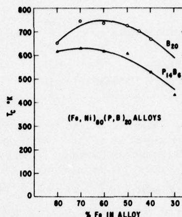
Fig. 3. Curie temperatures of amorphous alloys as function of transition metal composition. Curves calculated as described in text.
