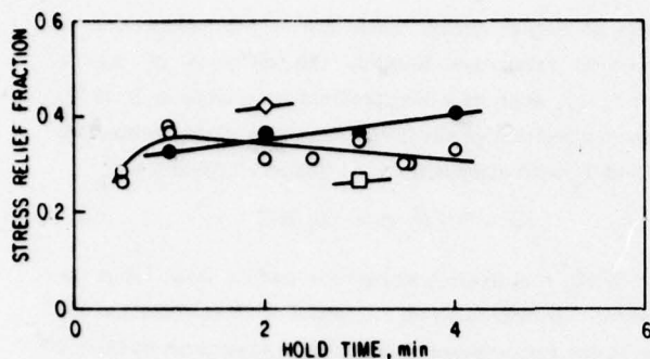
Fig. 7 Stress relaxation of \text{Fe}_{83}\text{B}_{17} as a function of process variations. ◇ 25cm diameter wheel, gas hold down; ● 25cm diameter wheel; □ 10cm diameter wheel; ○ 10cm diameter wheel with new furnace.
