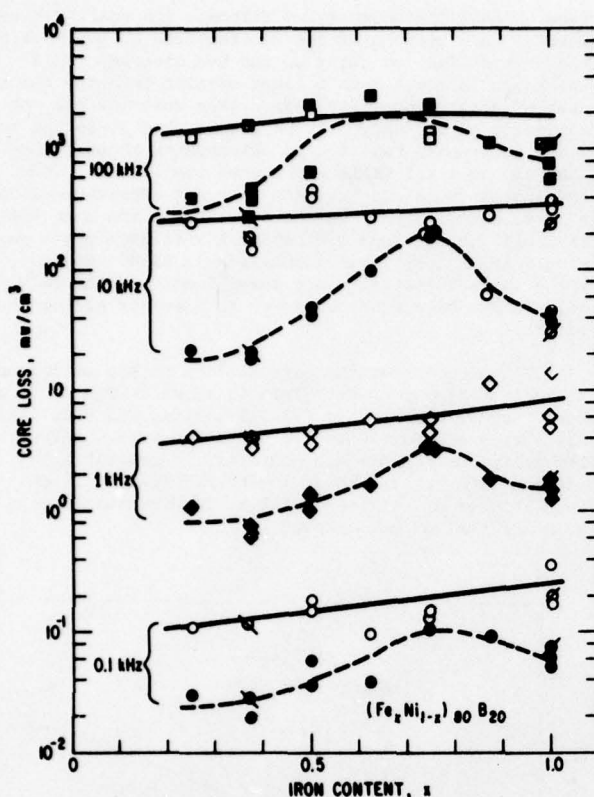
Fig. 6 Losses as a function of composition for \text{Fe}_x\text{Ni}_{80-x}\text{B}_{20} alloys at various frequencies at B_m = 1 kG using sine H excitation. Open symbols for as-wound toroids, solid symbols for annealed toroids.
