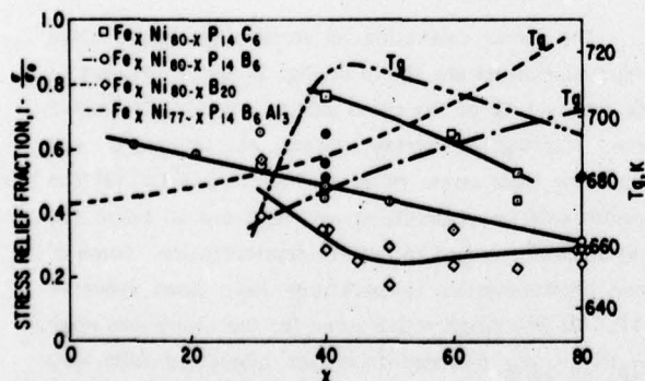
Fig. 4 Stress-relaxation after 2 hrs. at 225^\circ\text{C} for various alloys as a function of Fe given by solid curves. Alloys prepared by Allied Chemical Co. shown by solid symbols. Dashed curves show T_g ; — 22, --- and - - - [17].
