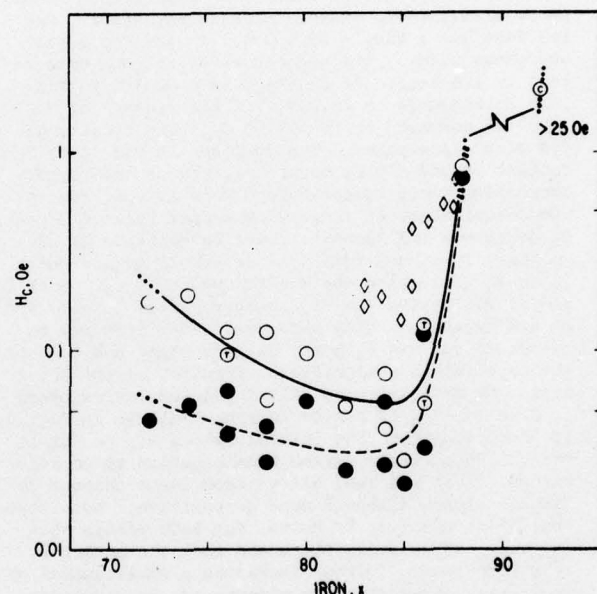
Fig. 5 Coercive field of FeB alloys. Open symbols for as cast alloys, solid symbols for minimum after annealing. \circ , \bullet Luborsky et al.; (7) \square Hargita and Lovas. (16) \Delta indicates a trace of crystallinity was observed in x-ray diffraction, \times indicates highly crystalline sample. Dotted lines indicates the presence of some degree of crystallinity as deduced from 4\pi M_s results.
