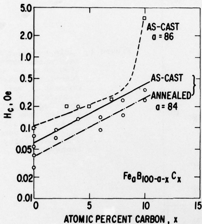
Figure 3. Intrinsic coercive field as a function of carbon content for as-cast and annealed \text{Fe}_{84}\text{B}_{16-x}\text{C}_x samples prepared in this work, \circ , and for as-cast \text{Fe}_{86}\text{B}_{14-x}\text{C}_x samples prepared at University of Pennsylvania, \square .
