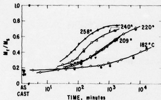
Fig. 1. Change in ratio of remanence to saturation on isothermal annealing in a circumferential field at different temperatures, after a preliminary anneal in a transverse field. Open symbols for measurements at the anneal temperature; solid symbols for measurements at room temperature.
