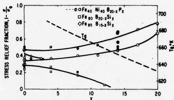
Fig. 5 Stress relaxation after 2 hrs. at 225^\circ\text{C} for various alloys as a function of metalloid composition given by solid curves. Alloys prepared by Allied Chemical Co. given by solid symbols. Dashed curve shows T_g [22]. \theta for one-half thickness of O.
