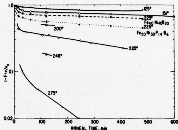
Fig. 1 Stress relaxation isotherms at various temperatures for \text{Fe}_{40}\text{Ni}_{40}\text{P}_{14}\text{B}_6 (open symbols), and at 225^\circ for \text{Fe}_{50}\text{Ni}_{30}\text{P}_{14}\text{B}_6 and \text{Fe}_{40}\text{Ni}_{40}\text{B}_{20} (solid symbols).
