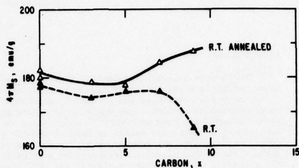
Fig. 4 Effect of annealing on saturation magnetization of some FeBC alloys.
