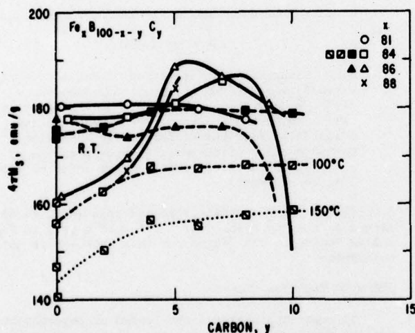
Fig. 3 Saturation magnetization of FeBC alloys as B is replaced by C. \circ , \square , \Delta , \times Hatta et al. (6) using solid lines; \bullet , \blacksquare , \blacktriangle , \times Luborsky et al.; (7) \blacktriangle measured by Luborsky et al. (7) on Hatta's samples using broken lines.
