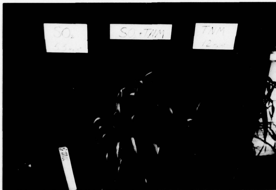
Fig. 34. \text{SO}_2 , 5.3 \text{ mg/m}^3 , and \text{TNM} , 1.2 \text{ mg/m}^3 , singly and combined on wheat.
