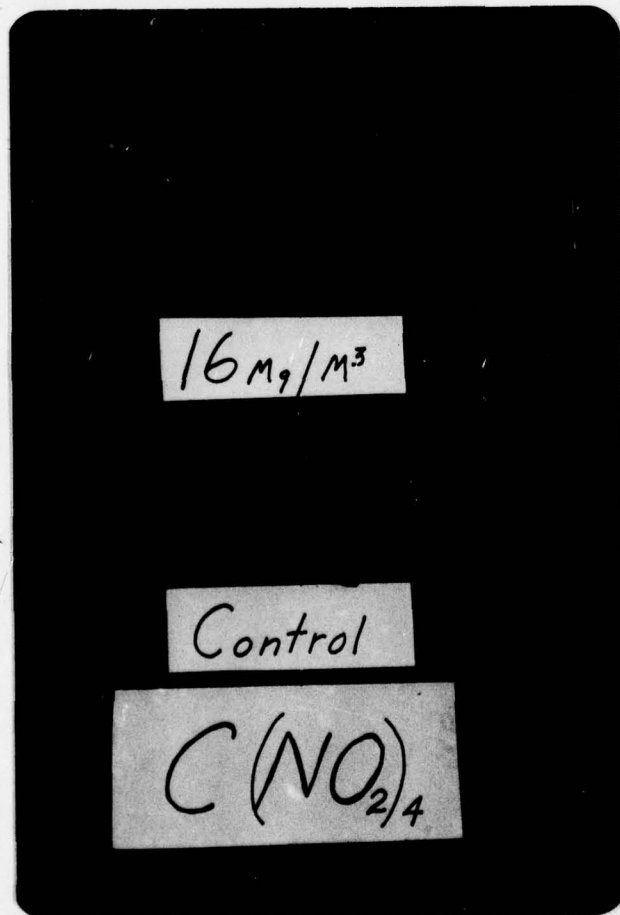
Fig. 37. Effect of TNM, 16.0 \text{ mg/m}^3 , on young oak leaf showing stipple and interveinal necrosis.
