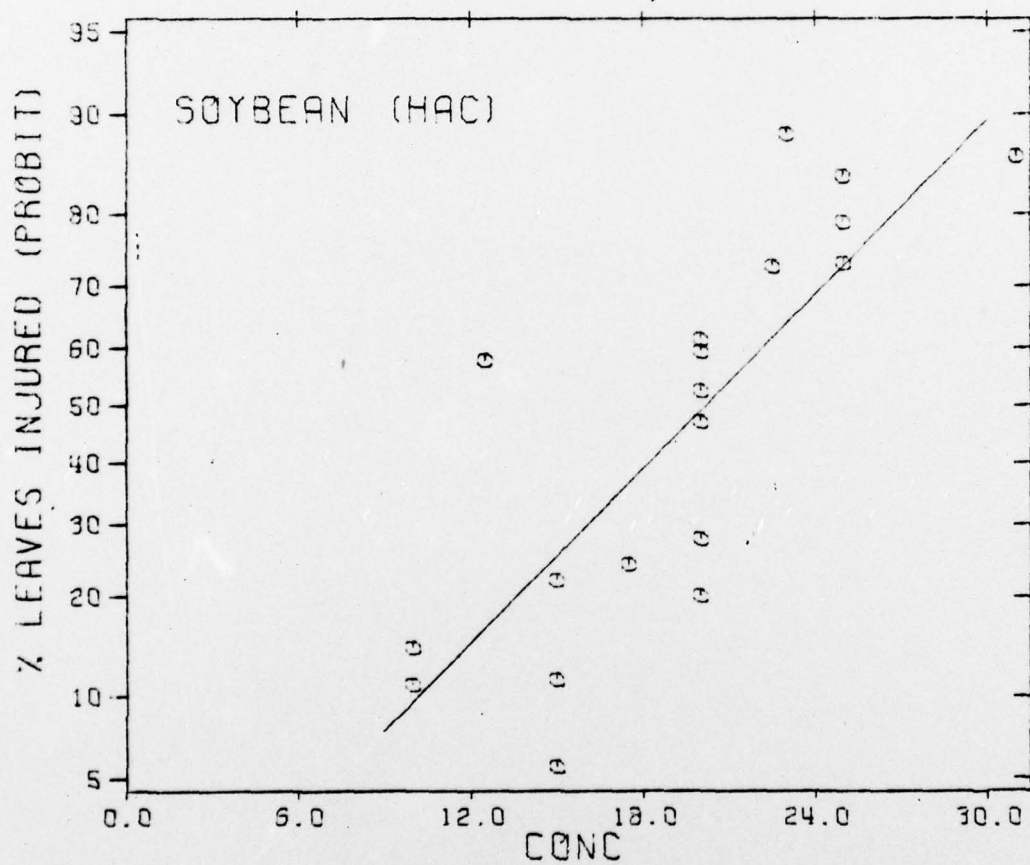
Figure 9. Effect of Acetic Acid on Percent of Leaves Injured With Soybean
