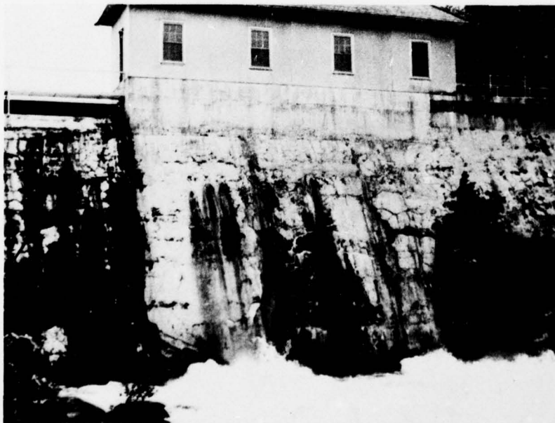
DOWNSTREAM FACE OF GATE HOUSE
