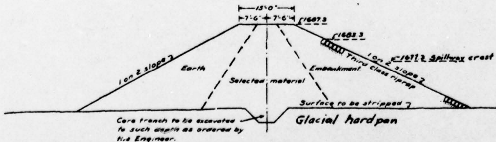
SECTION-SOUTH DAM
