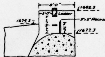
ELEVATION LOGWAY BULKHEAD
