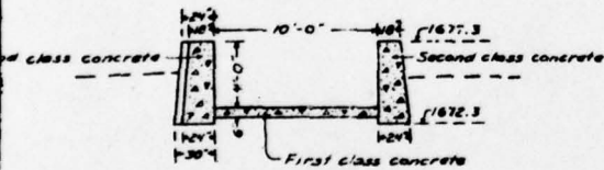
SECTION D-D LOGWAY
