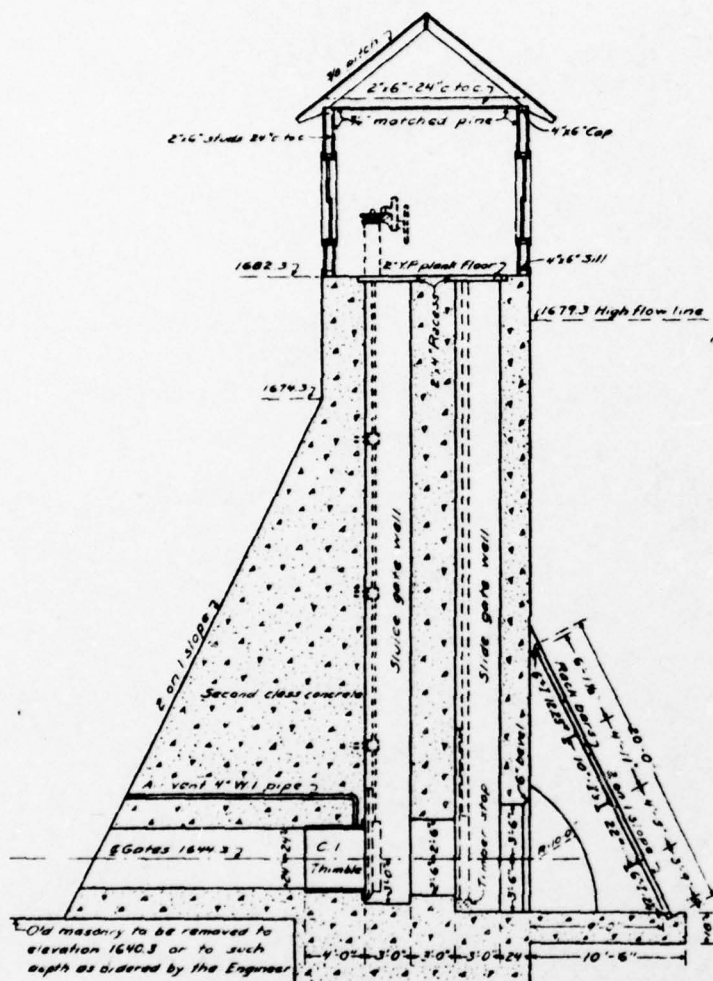
SECTION G-G
