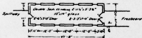
WALL PLAN - GATE HOUSE
