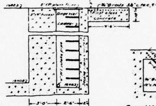
SECTION F-F
