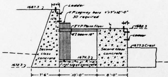
SECTION C-C-LOGWAY
