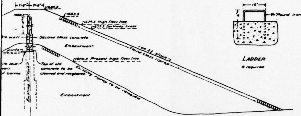
SECTION-NORTH DAM
