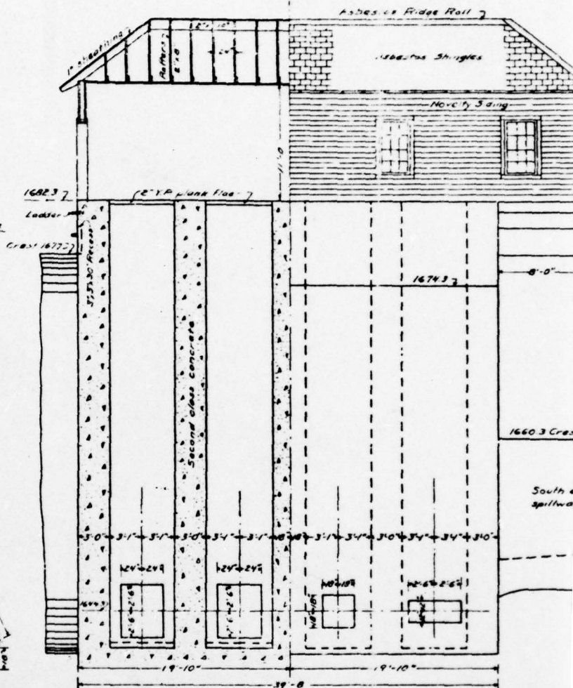
HALF SECTION H-H
