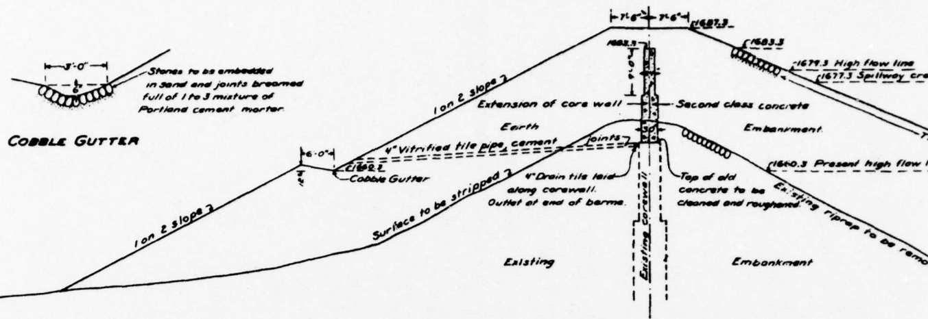
SECTION-NORTH DAM
