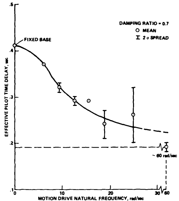
Fig. 7. Effective pilot time delay vs motion drive natural frequency.
