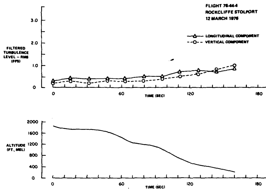
FIG. 6(b): TURBULENCE LEVEL VARIATION DURING APPROACH
