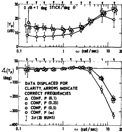
Fig. 4 Pilot describing functions for the pitch task, averaged over 4 pilots
