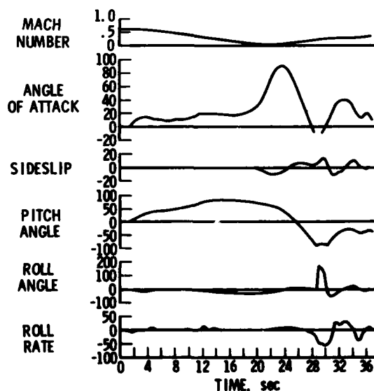
Figure 12. Vertical Stall Entry Maneuver
