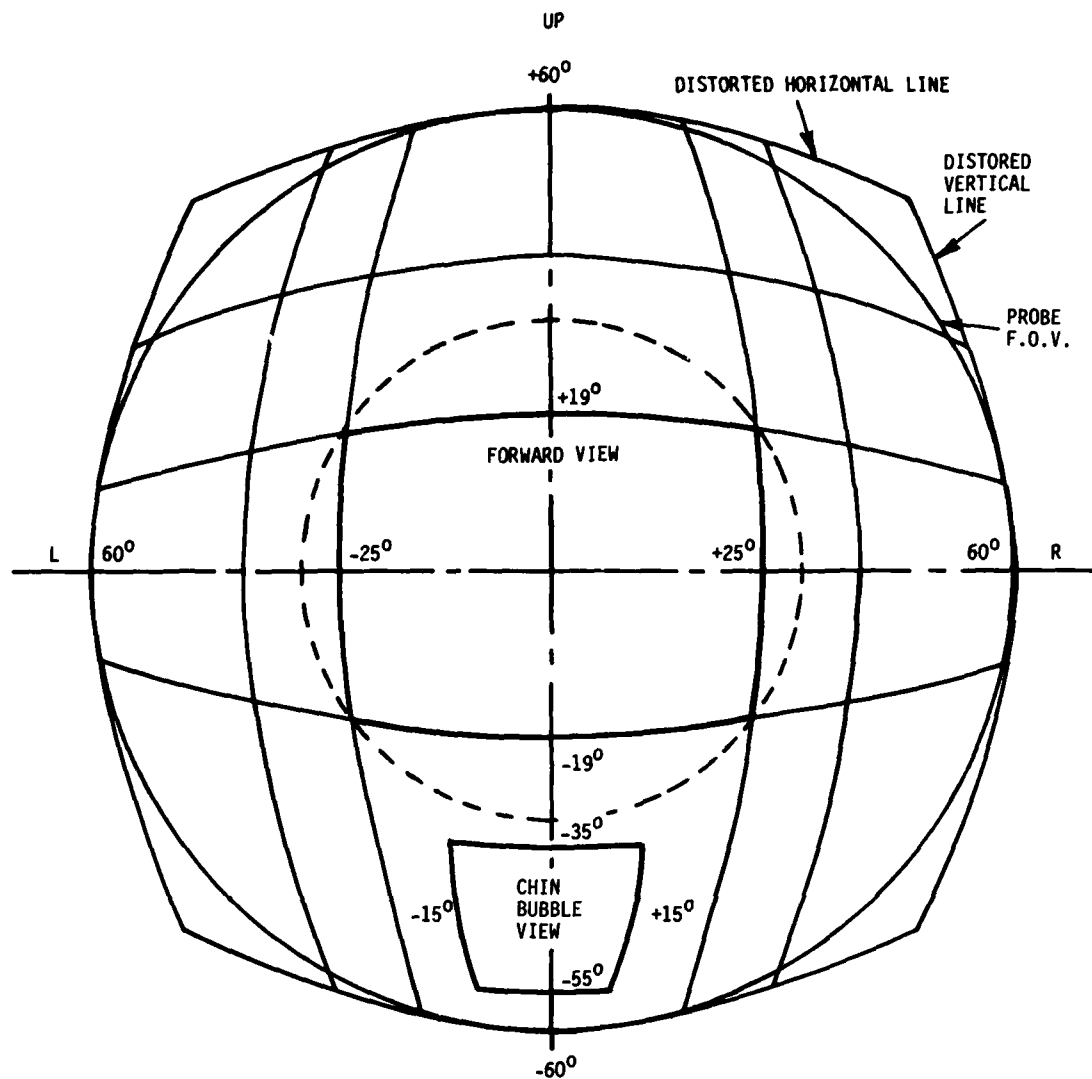
Figure 6 Field of View of CH-47 Probe
