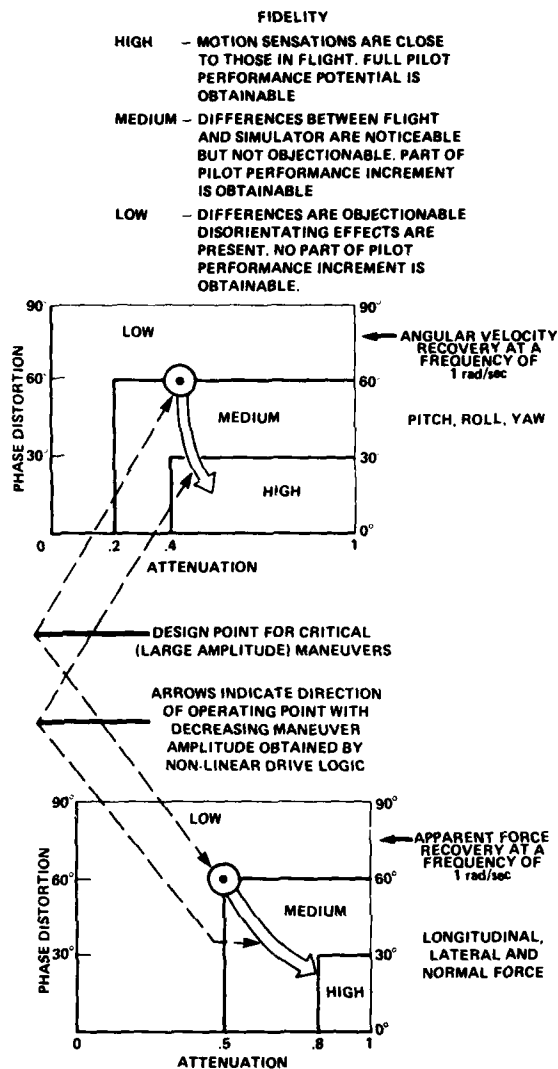
Fig. 6. Platform motion fidelity criteria.
