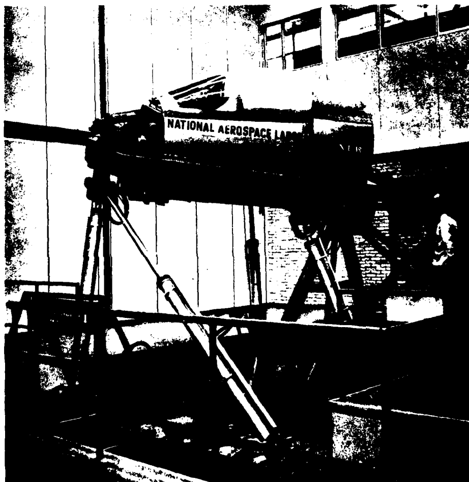
Figure 9 - The Four Degree of Freedom Flight Simulator with Single Seat Fighter Aircraft
