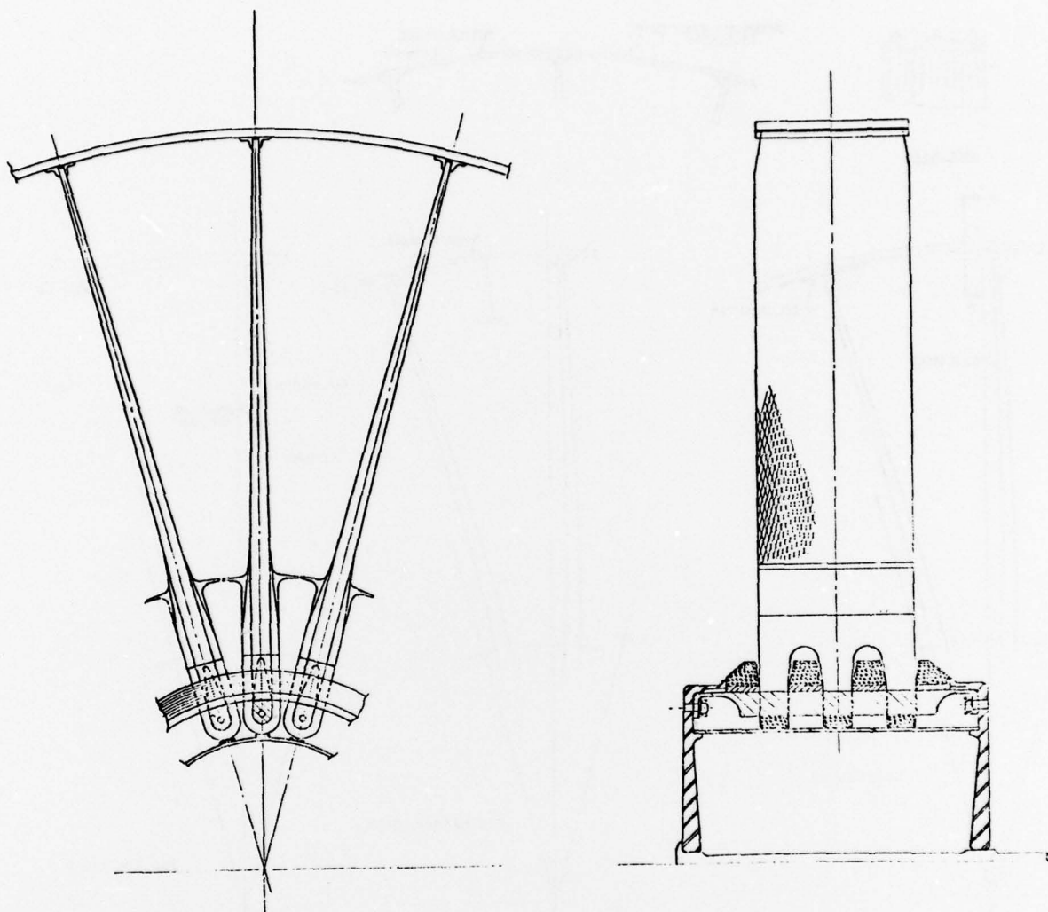
Figure A-28. Supersonic-Flight Fan: Pinned-Blade/Hoop Demonstrator.
