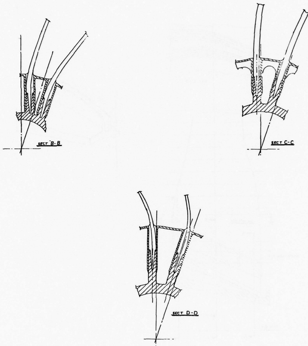
Figure A-4. Supersonic-Flight Composite Blisk: Double Lap Shear Design (Radius Slot).
