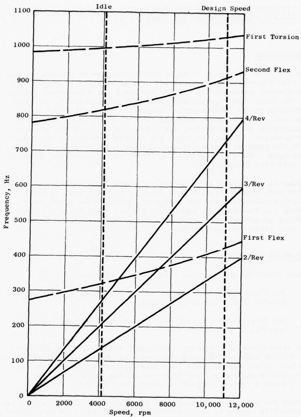
Figure 13. Supersonic-Flight; Unshrouded 18-Blade-Fan-Rotor Campbell Diagram.
