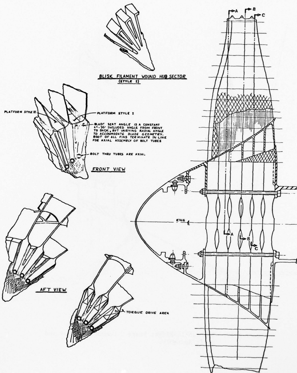
Figure A-11. Supersonic-Flight Blisk with Composite Hub (Concluded).
