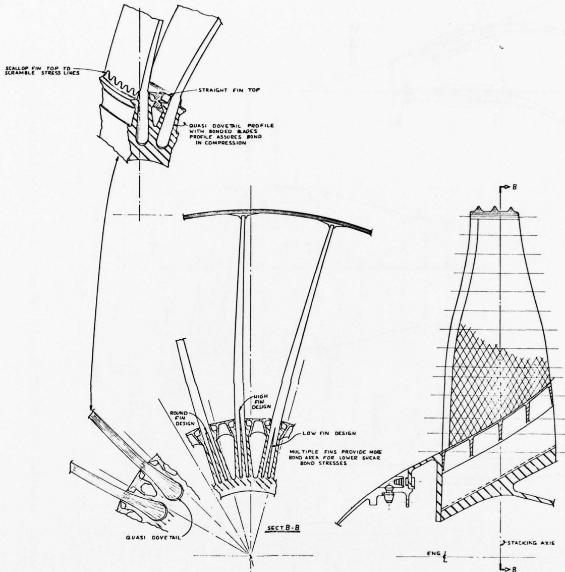
Figure A-10. Supersonic-Flight Composite Blisk.
