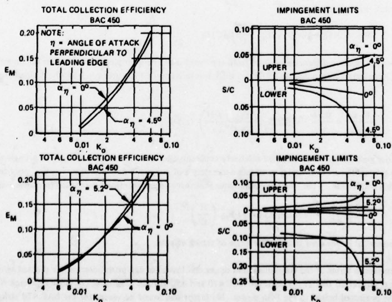
Figure 18—Test Airfoil Impingement Characteristics
