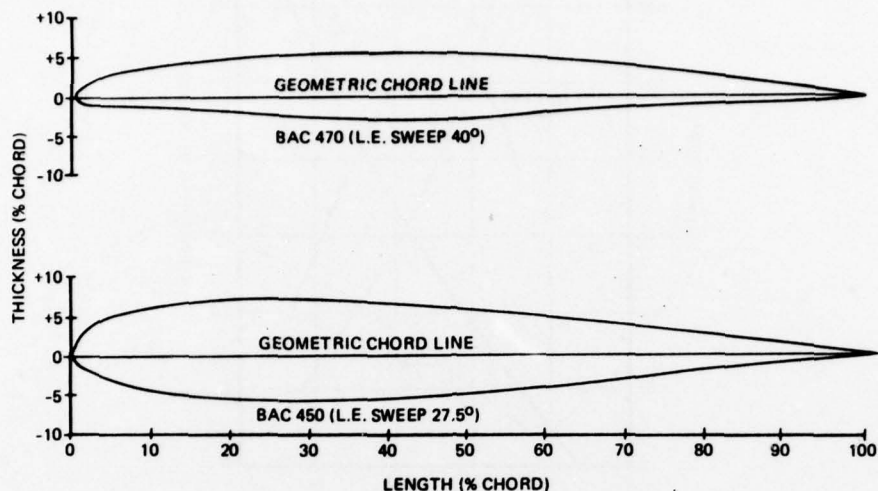
Figure 7—Airfoil Cross Section Streamwise Direction
