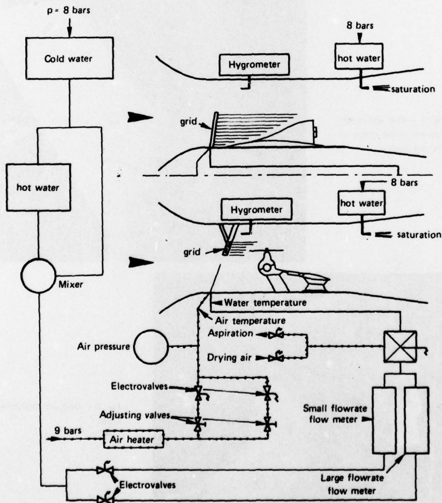
Fig. 3 - Icing and saturation devices.
