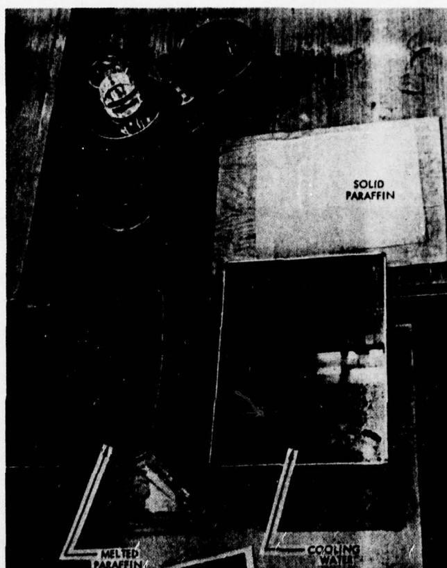
Figure 9—Test Equipment for Weighing and Obtaining Ice Shape Molds
