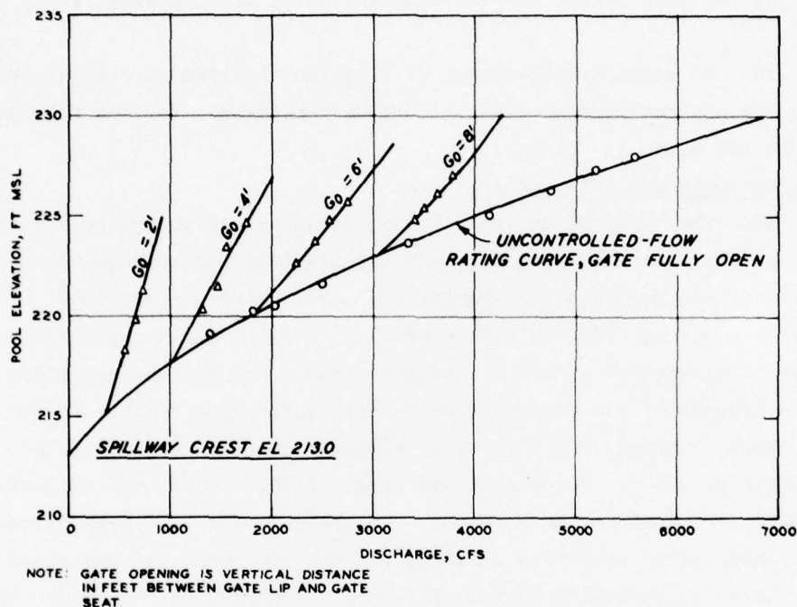
Figure 5. Rating curves for one gate bay of Spillway A
