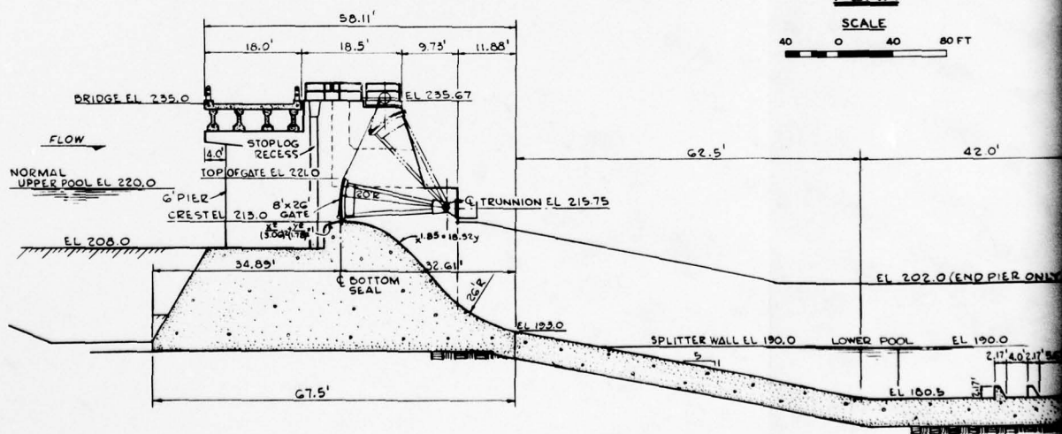
GATED SPILLWAY SECTION
