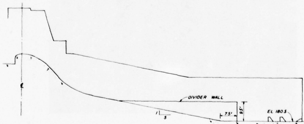
Figure 8. Type 1 divider wall, Spillway A
