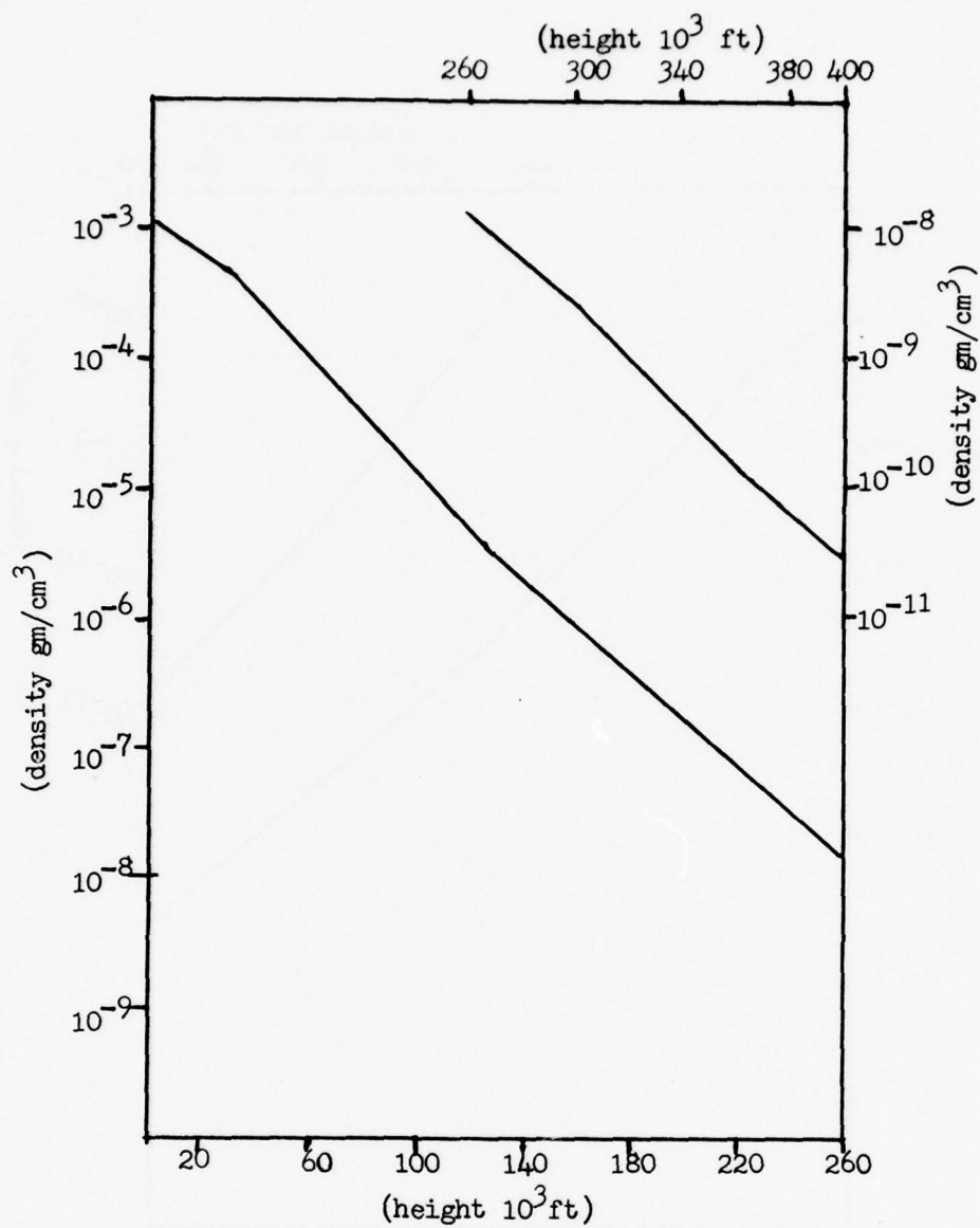
FIGURE C4: Example of an extended density profile (46N, January).
