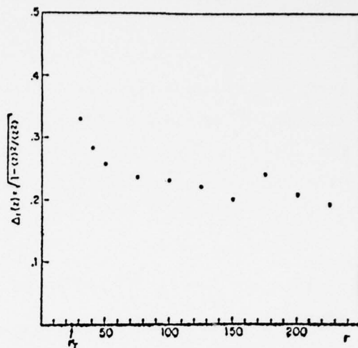
Average normalized fluctuations \Delta r(z) = \Delta \langle z \rangle / \langle z^2 \rangle^{1/2} for various values of r . Fig.2
