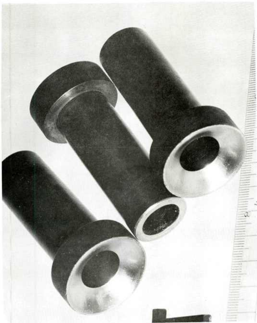
Figure 9. Typical Teflon-coated steel die agates following seven weeks of production use.
