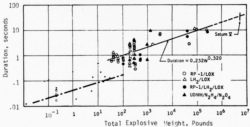
Figure 9. Fireball Durations
