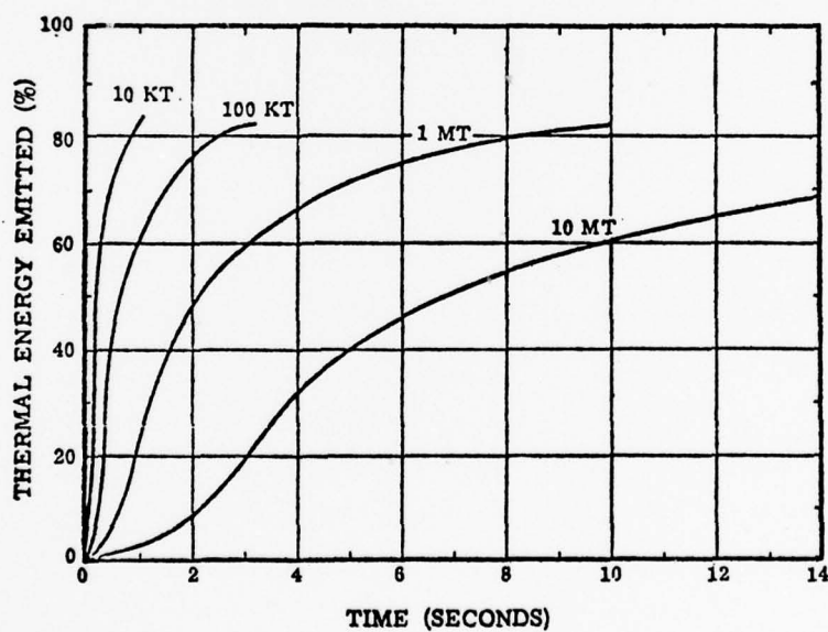
Figure 1b. Percentage of Thermal Energy Emitted as a Function of Time for Air Bursts of Various Yields.
