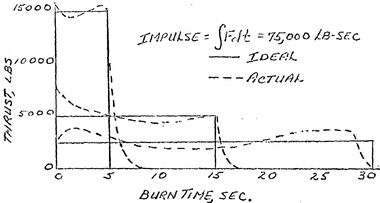
FIG. 2. THRUST-TIME PERFORMANCE
