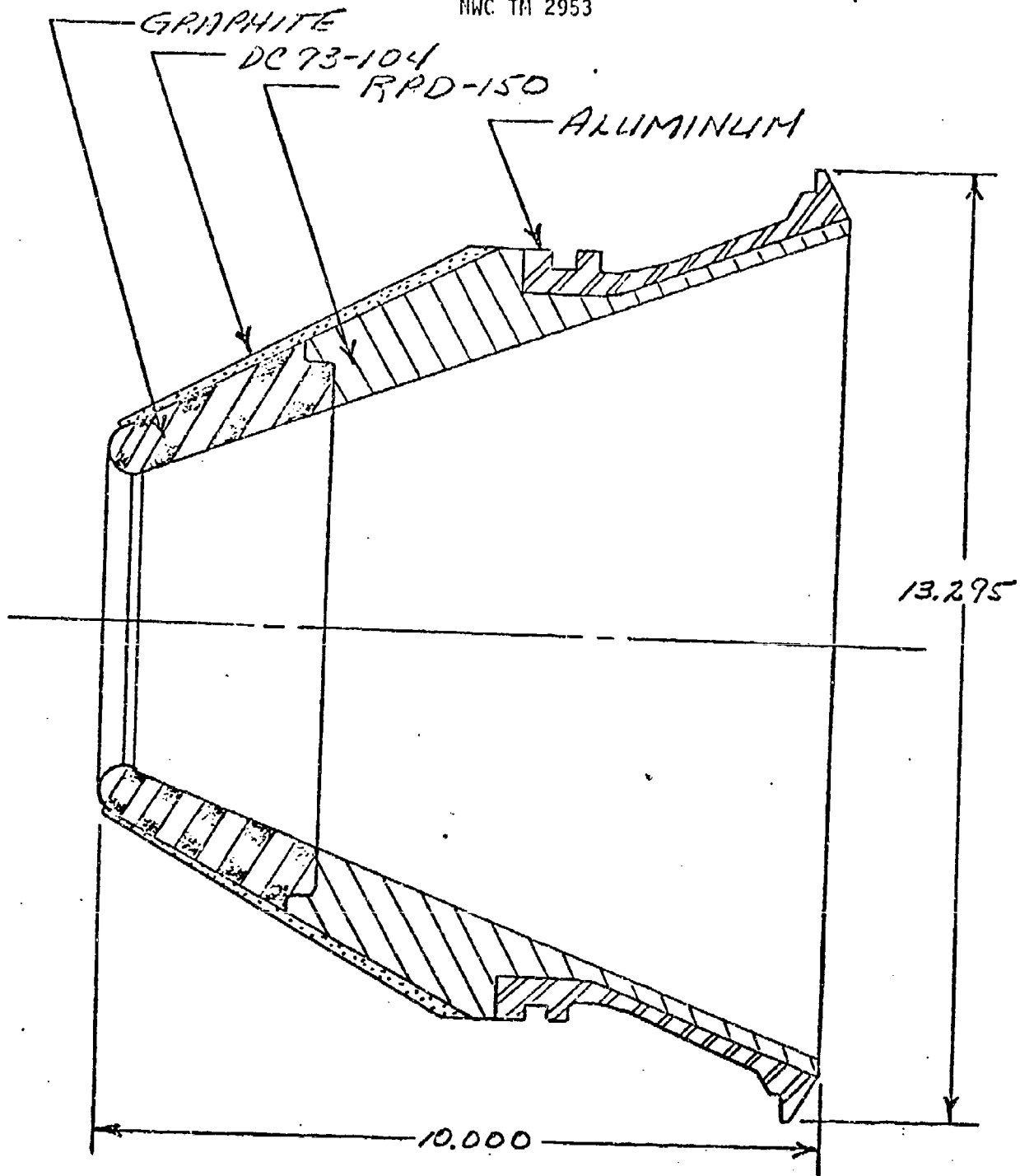
FIG. 13. NOZZLE DESIGN
