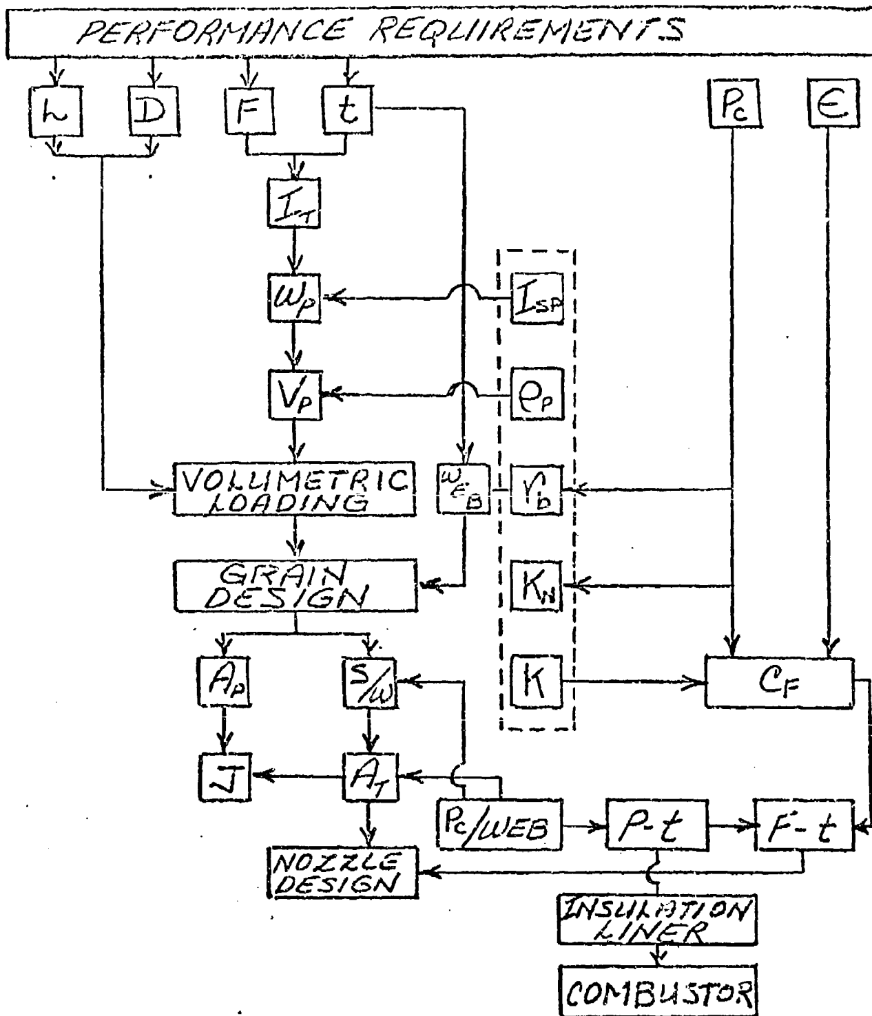
FIG. 11. CALCULATION SEQUENCE
