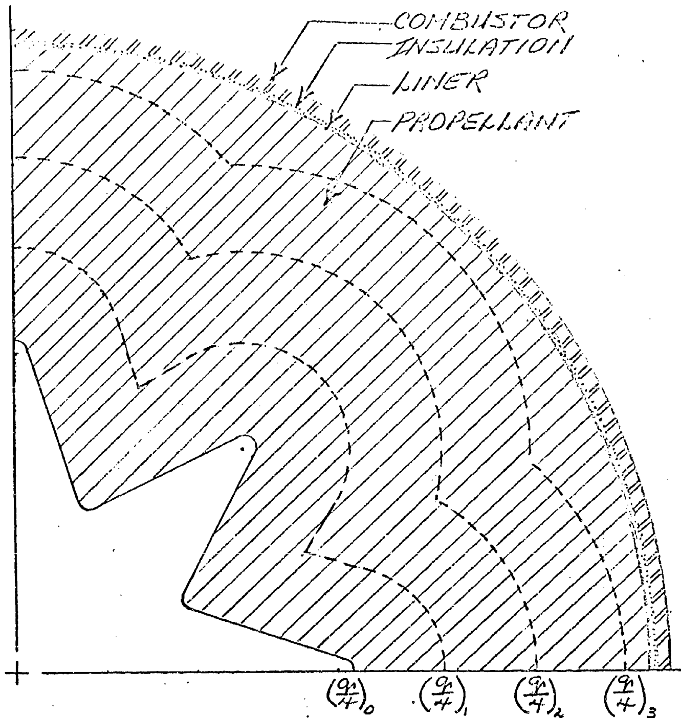
FIG. 5. SURFACE AREA BURN-BACK CONTOUR
