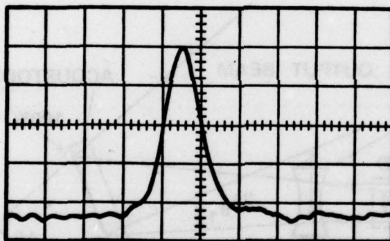
FIGURE 12. A Q-Switched Pulse From the Nd/YAG Cavity is Shown in This Oscilloscope Trace. The horizontal time scale is 50 nsec/div and the acoustic bandwidth is 33 MHz.
