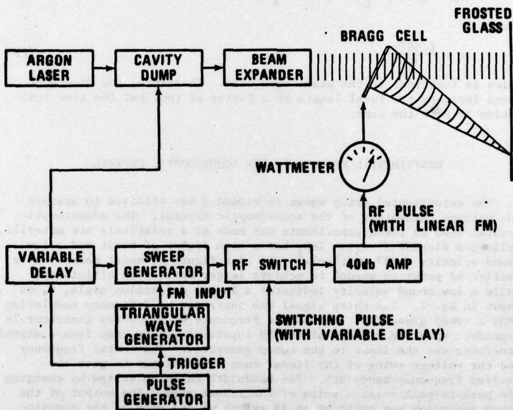
FIGURE 5. This Schematic Diagram Illustrates the Experimental Arrangement Used to Observe and Measure the Coordinates of the Focus of the Acoustooptic Lens.
