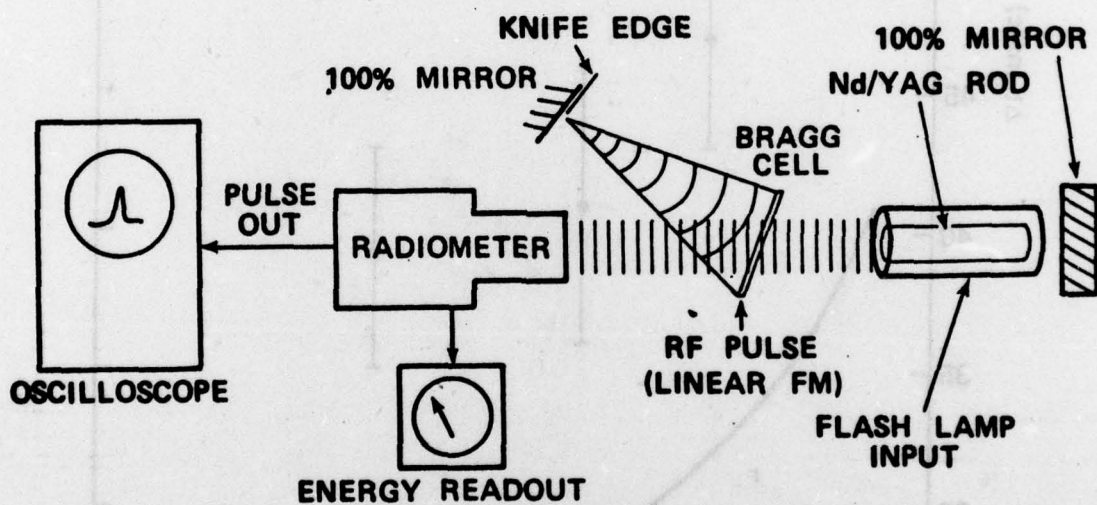
FIGURE 11. Experimental Arrangement of Nd/YAG Cavity Q-Switched With Acoustooptic Lens.
