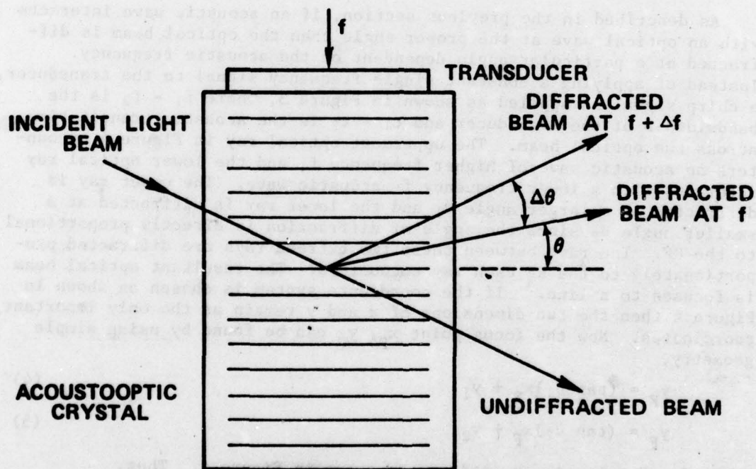
FIGURE 2. Physical Relationship Between the Optical Beam and Acoustic Frequency; Larger Frequency Yields a Larger Diffraction Angle.
