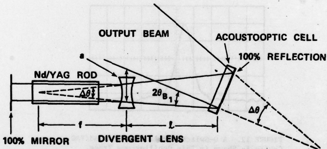
FIGURE 13. This Proposed Configuration of a Nd/YAG Cavity Eliminates one of the Undesired Output Beams and Increases Laser Efficiency.
