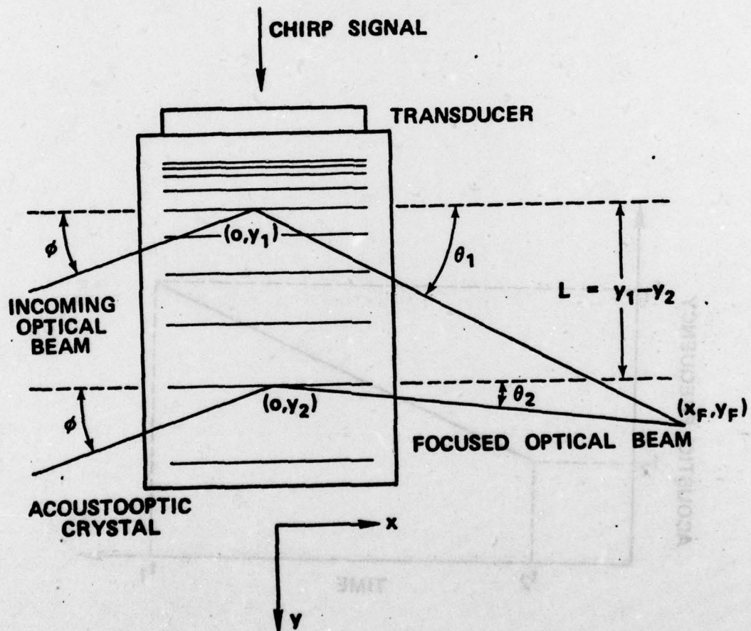
FIGURE 4. Output Optical Beam is Focused at Point x_F, y_F Due to the Traveling Acoustic Wave.
