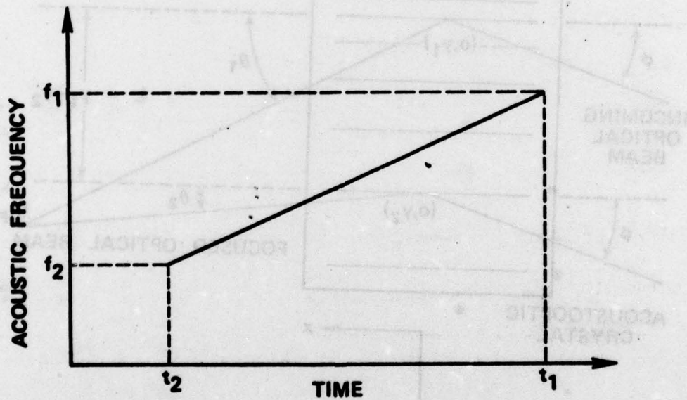
FIGURE 3. Chirp Signal Applied to the Acousto-optical Crystal. The frequency varies linearly with time.
