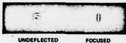
FIGURE 7. This Photograph of the Undeflected Argon Laser Beam on the Left and the Focused Deflected Beam on the Right was Observed Through a Frosted Glass Placed in the Focal Plane of the Acoustooptic Lens. The argon laser was pulsed in synchronism with the presence of the acoustic pulse in the Bragg cell in order to "freeze" the motion of the focal line.
