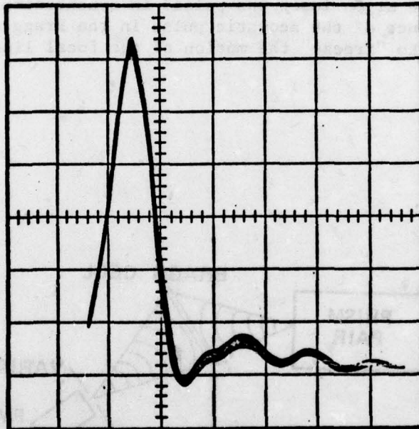
FIGURE 9. A Typical Oscilloscope Trace of the Output of the Photomultiplier. The horizontal time scale is 50 nsec/div and the bandwidth of the acoustic pulse is 30 MHz.
