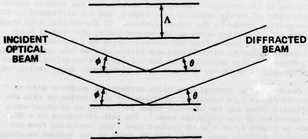
FIGURE 1. An Optical Beam Incident Upon an Acoustical Wave at Angle \phi and the Optical Beam Diffracted at Angle \theta .
