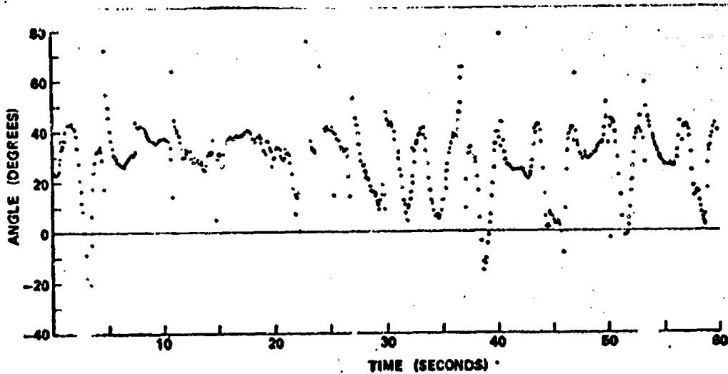
FIGURE 13. Angle of the Plane With Respect to the Vertical at Which the Ship Flexure Occurs Plotted as a Function of Time. Data taken from the angular flexure measurements of wave height of 4 feet. The average angle from vertical about which the ship flexes is 29.8 degrees.
