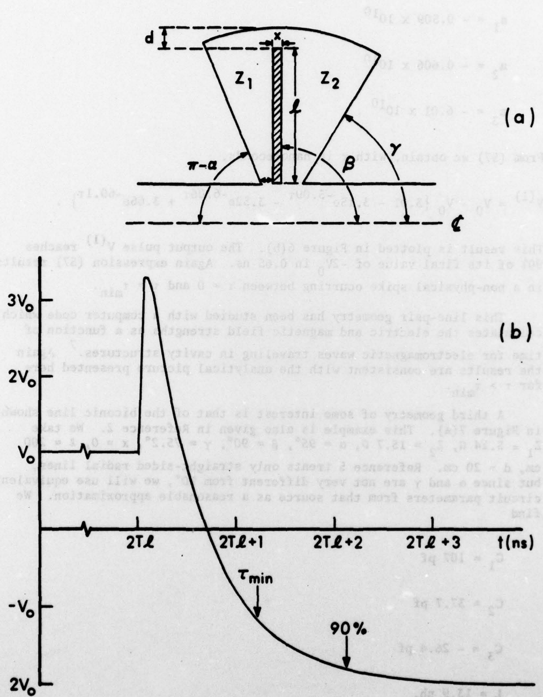
Figure 7. (a) Asymmetric biconic radial-line pair. (b) Open-circuit output pulse V^{(1)} .
