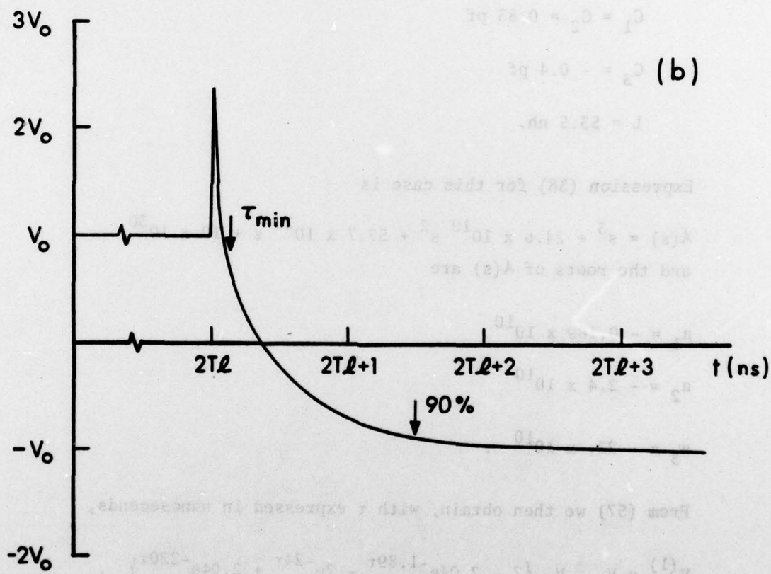
Figure 5. (a) Symmetric strip-line pair. (b) Open-circuit output pulse V^{(1)} .
