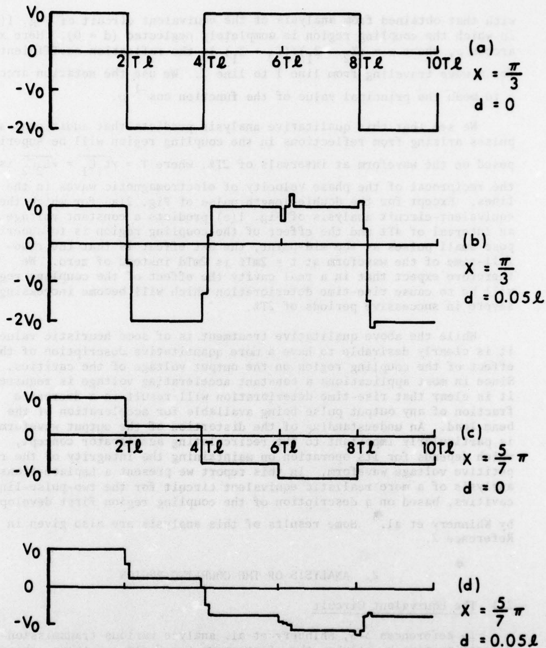
Figure 2. Idealized effect of coupling region on open-circuit output voltage. (a) x = \frac{\pi}{3} , coupling region neglected. (b) x = \frac{\pi}{3} , coupling region approximated by transmission line of length d = 0.05l . (c) x = \frac{5}{7}\pi , coupling region neglected. (d) x = \frac{5}{7}\pi , coupling region approximated by transmission line of length d = 0.05l .
