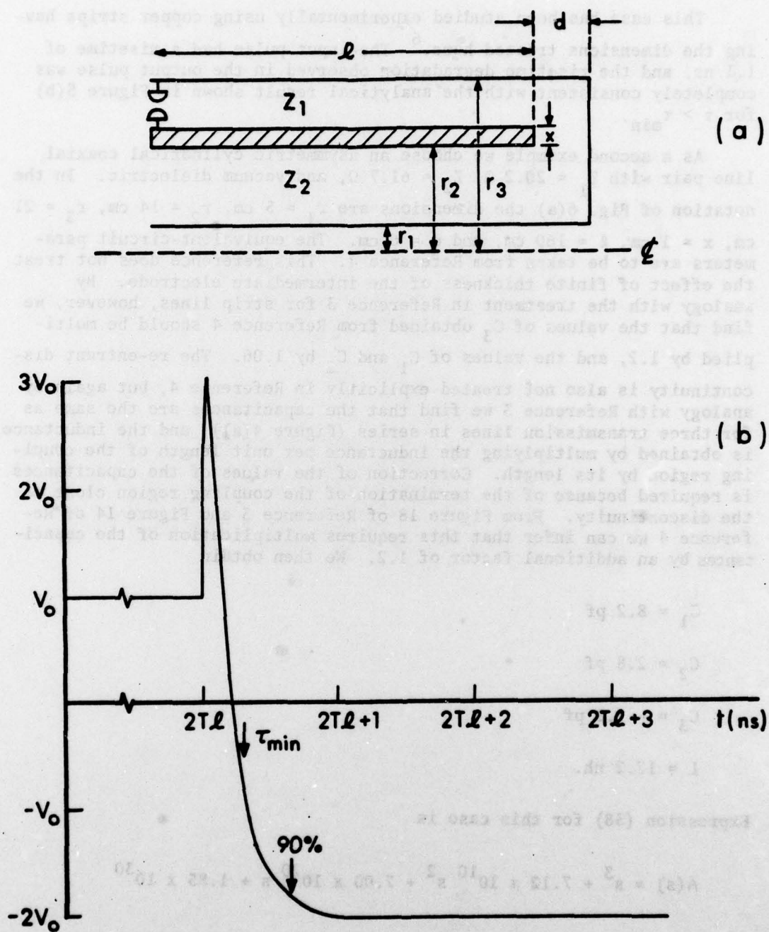
Figure 6. (a) Asymmetric coaxial-line pair. (b) Open-circuit output pulse V^{(1)} .
