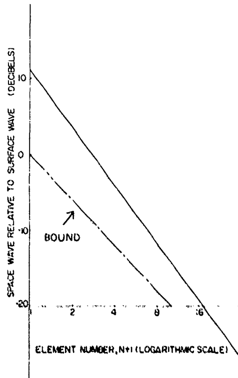
Fig. 6 -- Decay along the Yagi structure of the space-wave component of the current relative to the surface-wave component, computed for an infinite array of inclined dipoles with the same \theta_0 , a , b , and D as in Fig. 5 and for a free-space wavelength of 1 m ( kD = 1.257 )
