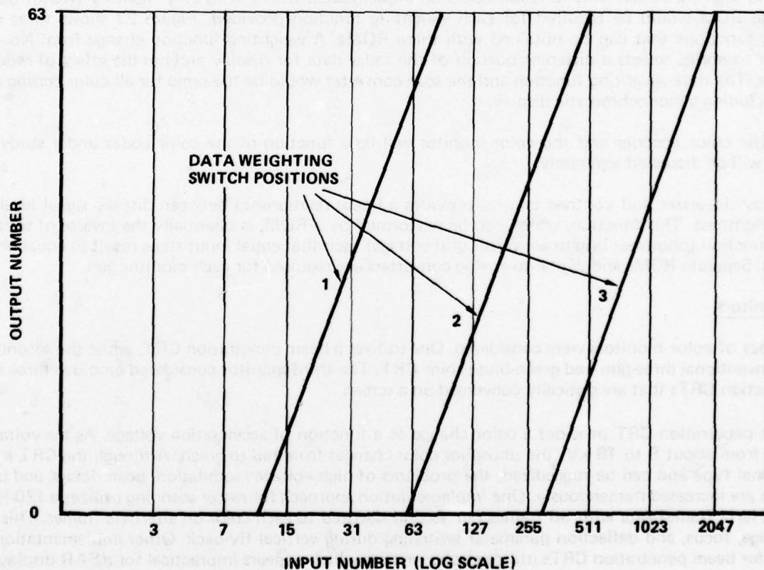
Figure 23 - Data Weighting
