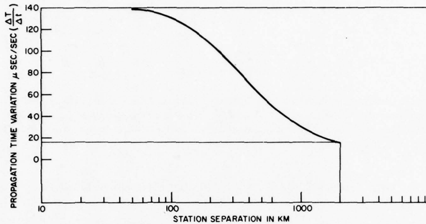
Fig. 10 — Propagation time variation vs station separation
