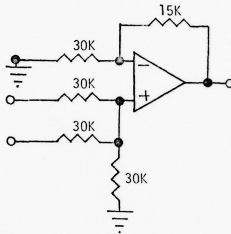
Difference Circuit
