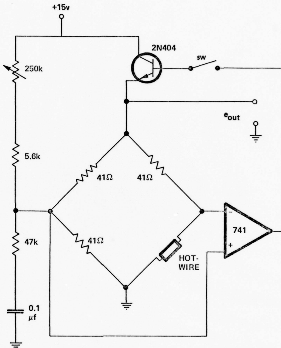
Figure 12 HOT-WIRE ANEMOMETER
