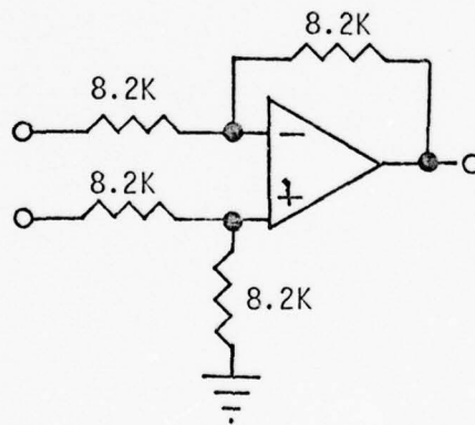
Difference Circuit
