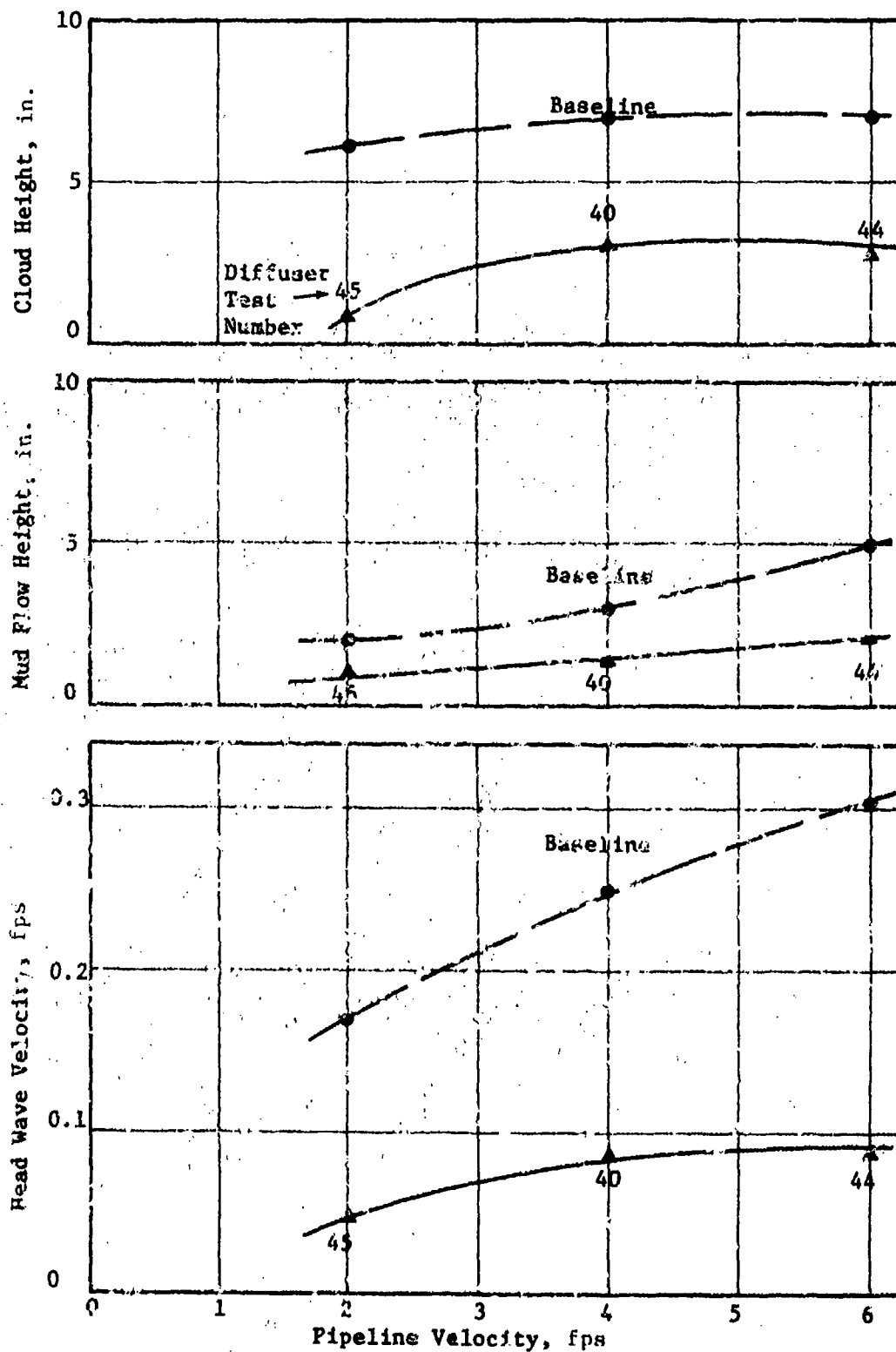
Figure 50. Diffuser results versus baseline results for various pipeline velocities
