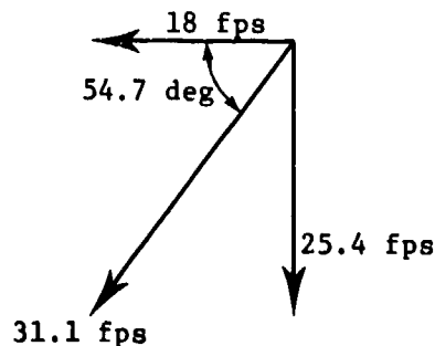
Figure 3. Jet vector diagram
