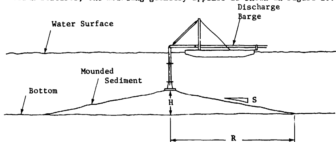
Figure 10. The conical mound
