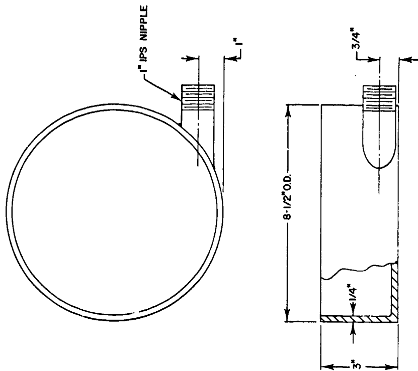
Figure 42. Weir model fabrication sketch
