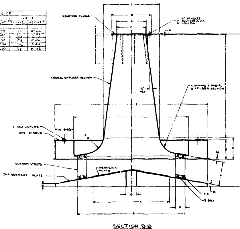
SECTION BB
