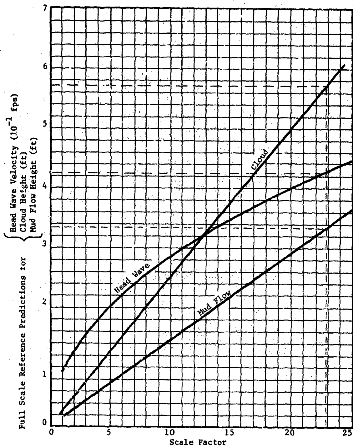
Figure 58. Full-scale predictions for operations with diffuser
