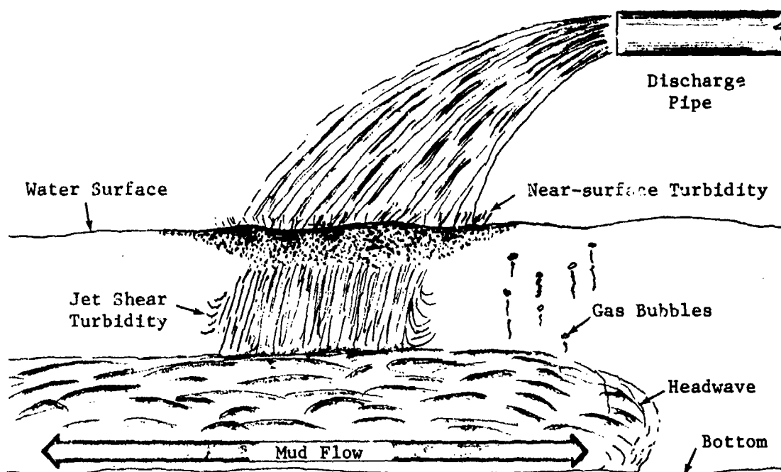
Figure 1. Slurry discharge jet
