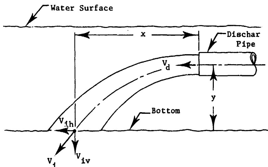
Figure 12. Schematic of horizontal submerged discharge
