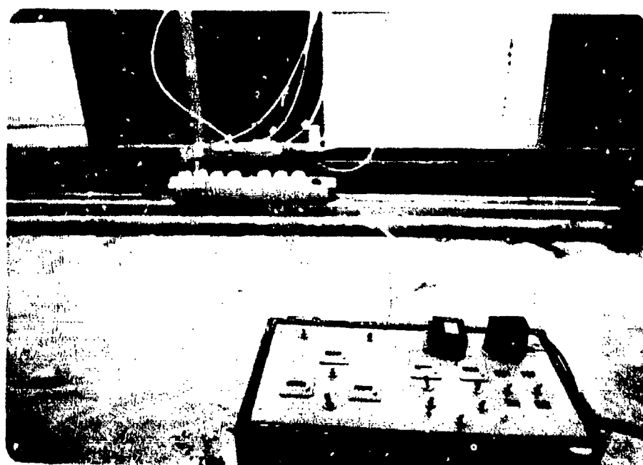
b. Camera timing control
