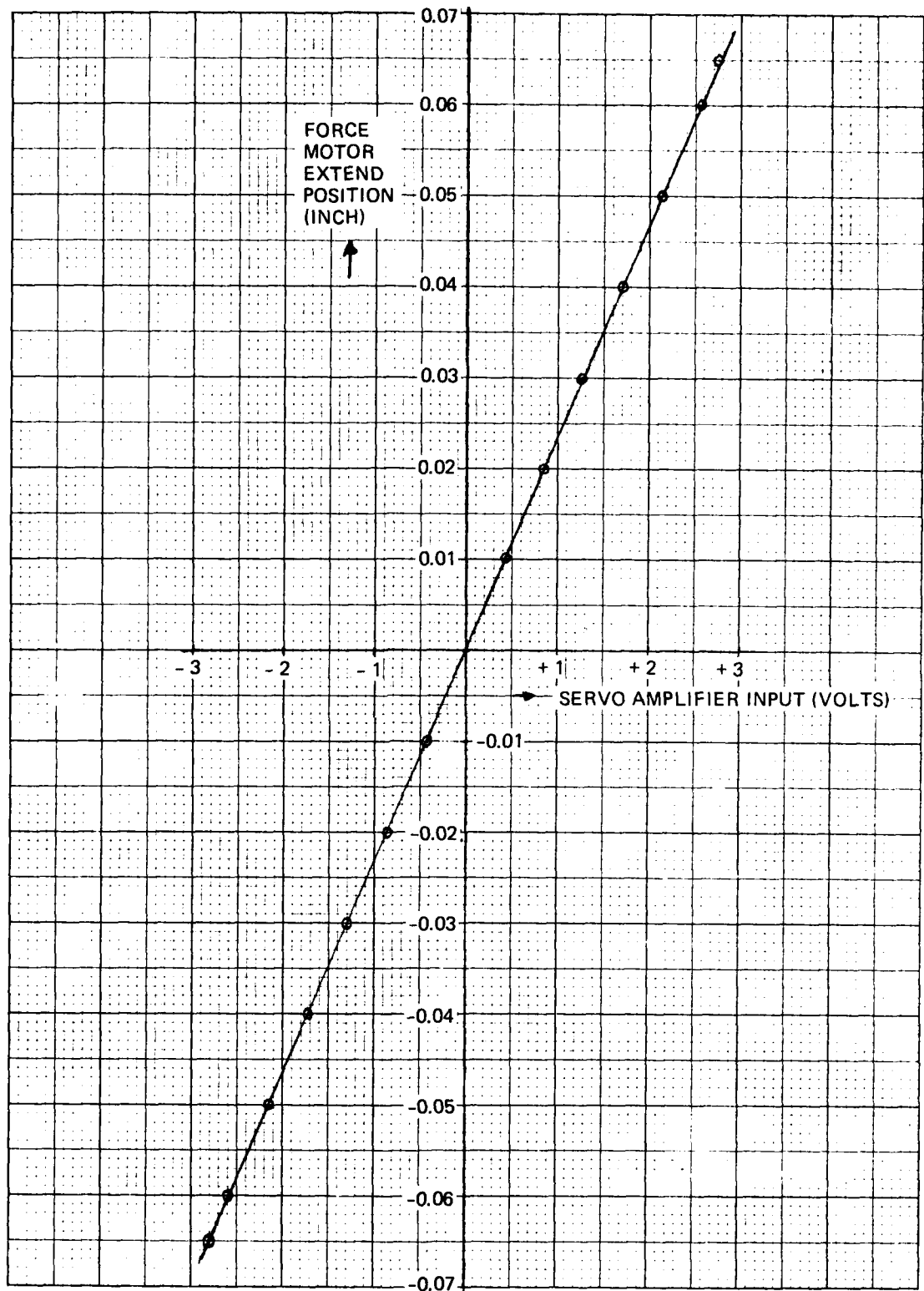
Figure 8. Force Motor Closed Loop Position Gain
