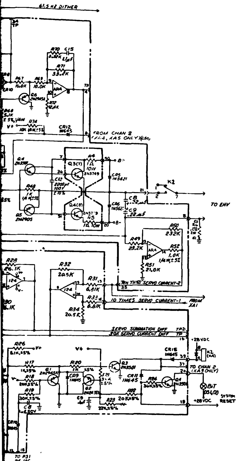
Electrical Schematic, Sheet 2
